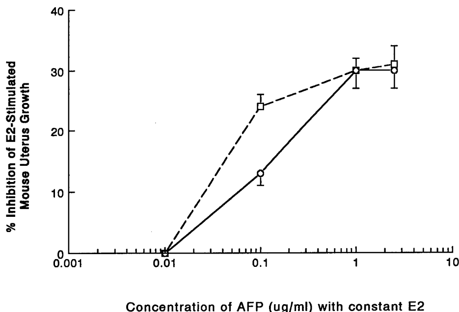
Fig. 1. Similarity of dose-response curves between natural (—○—) and recombinant (—□—) transformed human AFP. Various concentrations of AFP were incubated with 5 \mu\text{g/ml} \text{E}_2 for 1 hr at room temperature to induce transformation of AFP. Each incubation mixture was injected i.p. in a volume of 0.1 ml into 5 replicate mice. Mice were then challenged with \text{E}_2 and uterine wet weights were measured as described in Table 1. Inhibition of uterine growth was determined by comparing uterine weights in the AFP-treated groups to those in groups injected with saline (unstimulated) and those injected with \text{E}_2 only (fully stimulated) as described in Table 1. The mean percent growth inhibitions \pm the standard errors were calculated for each dose of AFP.
