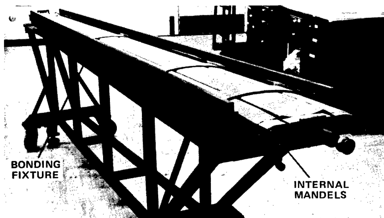
Figure 15 - X-Wing Box Beam Bonding Fixture
