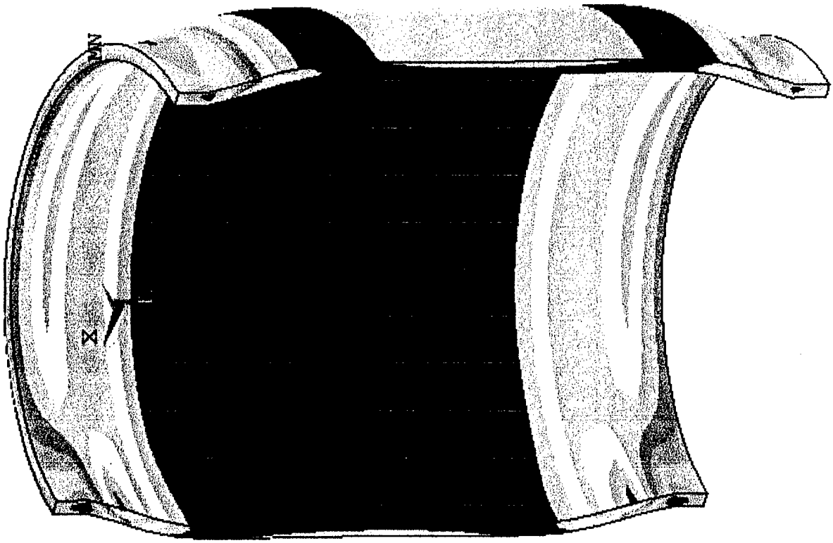
stress contours on the cylindrical housing under 100 PSI, t=1/8"
