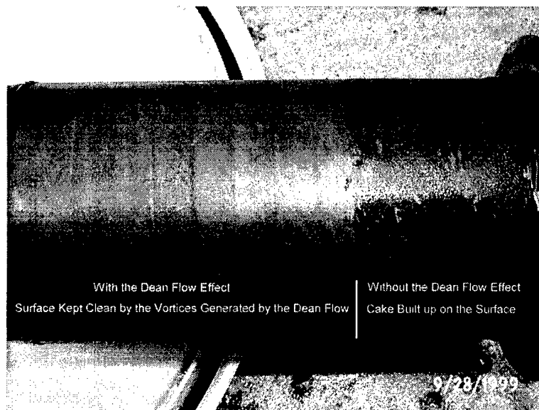
Figure 7: Effect of Dean Flow on Test Cartridge Used in Water Filtration
