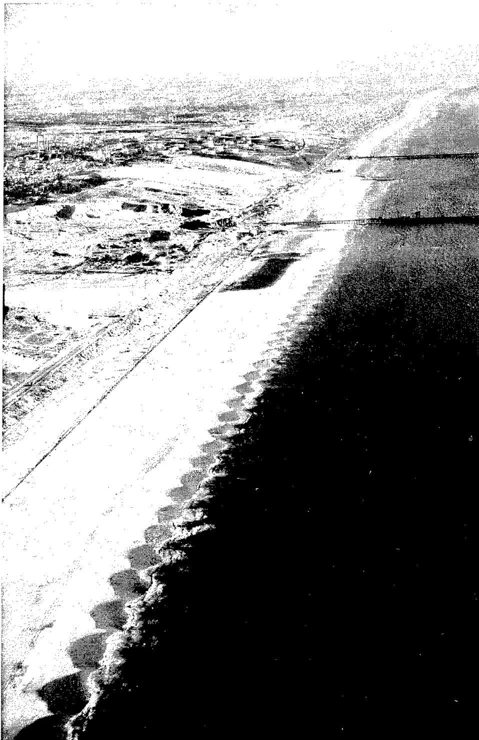
Figure 21. Beach cusps, El Segundo, Santa Monica Bay, CA (by U.S. Marine Corps, probably 1949) (from Wiegel et al. 1951)
