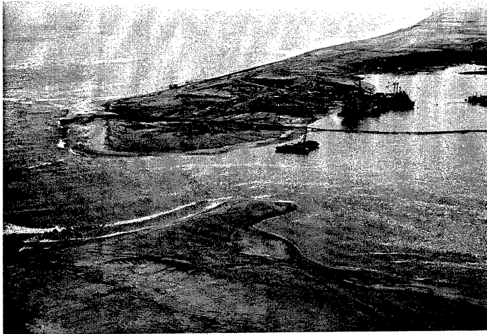
Figure 33. Tuy Hoa, Vietnam; aerial photograph of Air Force air base harbor, dredging and entrance (by R. L. Wiegel, November 1966)
