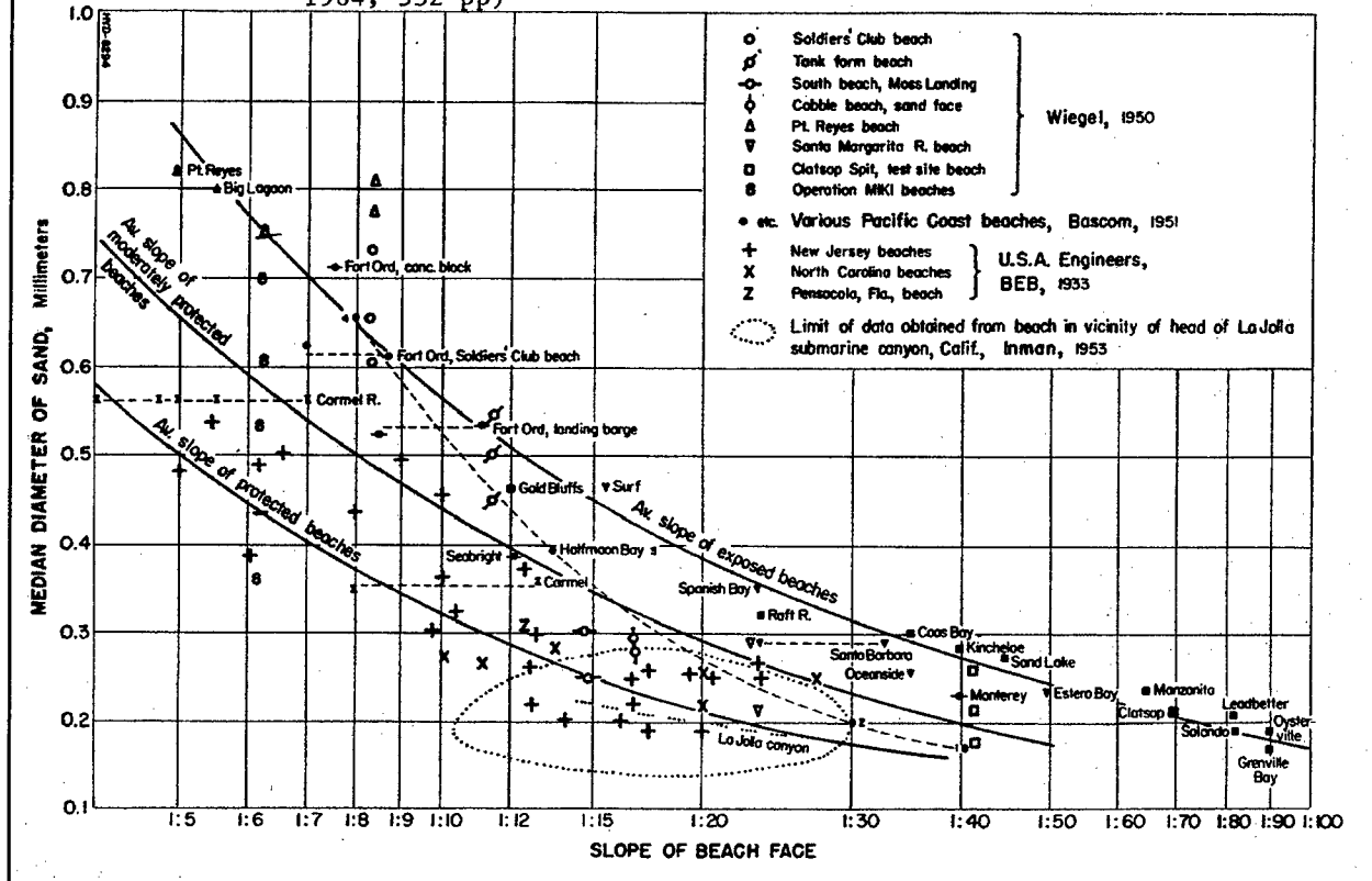
Figure 25. Size-slope-exposure relationship of beaches at the reference point (from Wiegels 1964)
