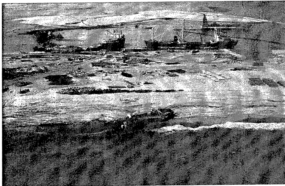
Figure 34. Tuy Hoa, Vietnam; aerial photograph of dredging harbor in Song Da Rang Bay (Note ship aground on beach and ships in harbor. By R. L. Wiegel, November 1966)
