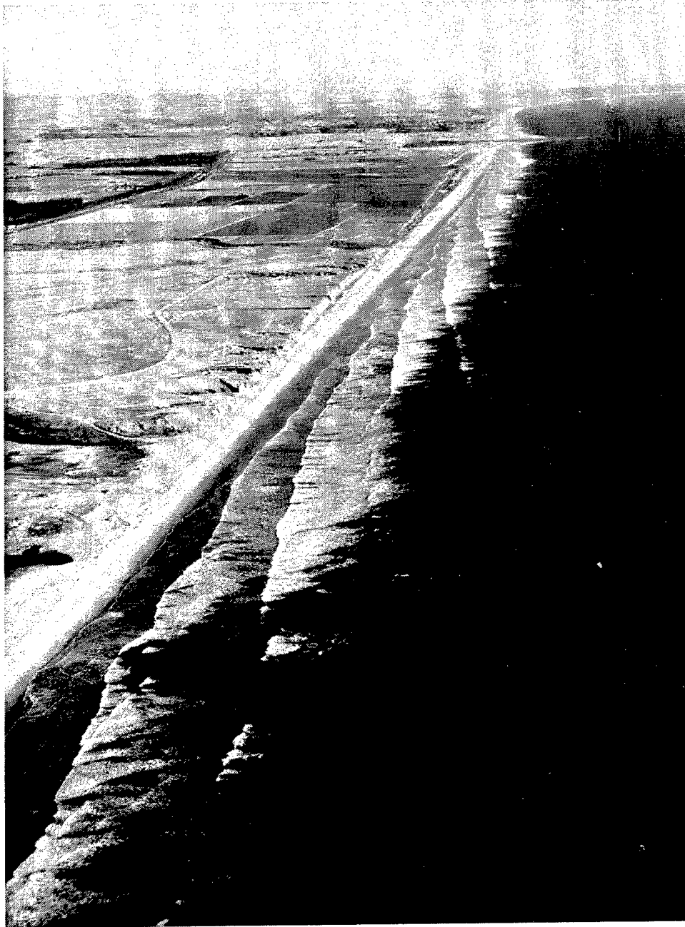
Figure 22. Long-crested waves breaking at an angle with beach; alongshore currents generated (by U.S. Marine Corps 1949)
