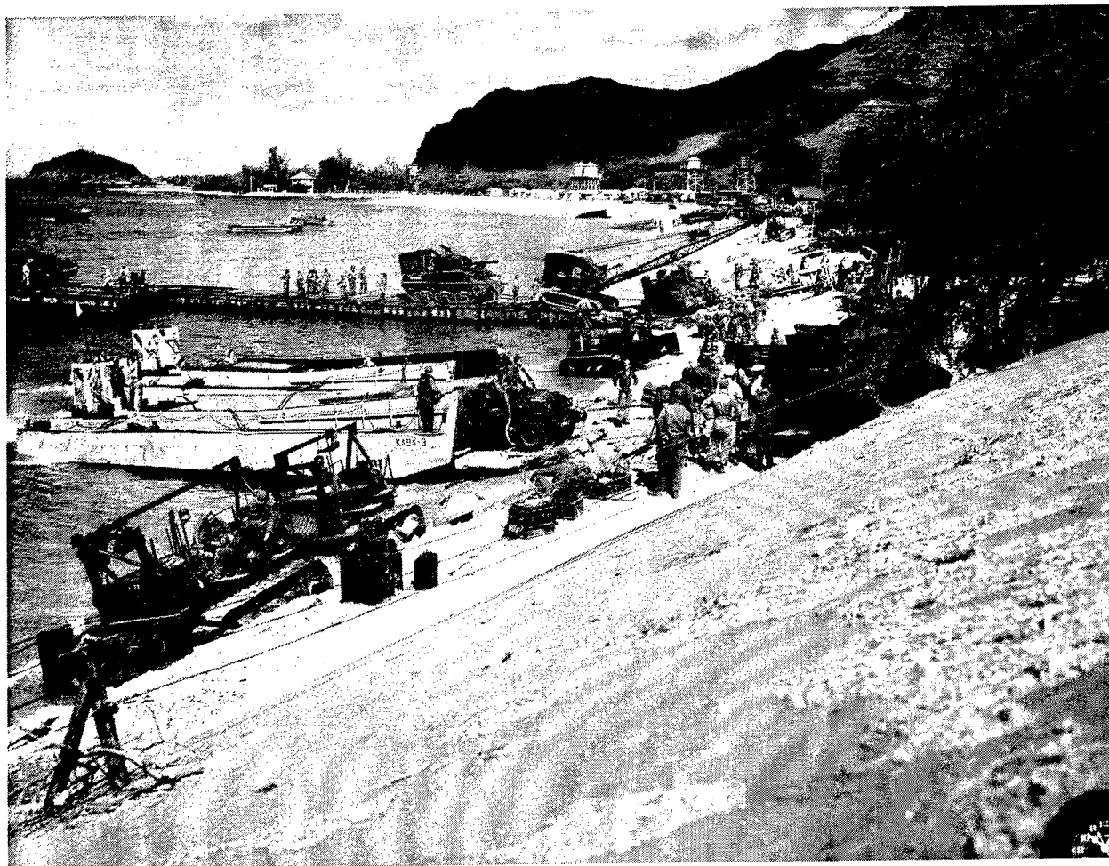
Figure 18. Operation MIKI, Waianae, Oahu, HI; congested beach during amphibious assault training exercise, October 1949 (from Wiegel and Kimberley 1949)
