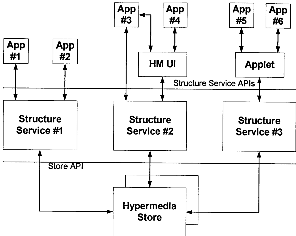
Figure 1 Open Hypermedia Architecture [Wil and Nurnberg, 1999]
