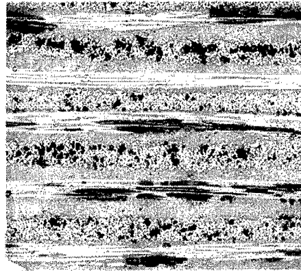
Figure 14. Sample showing 16% BN fill
