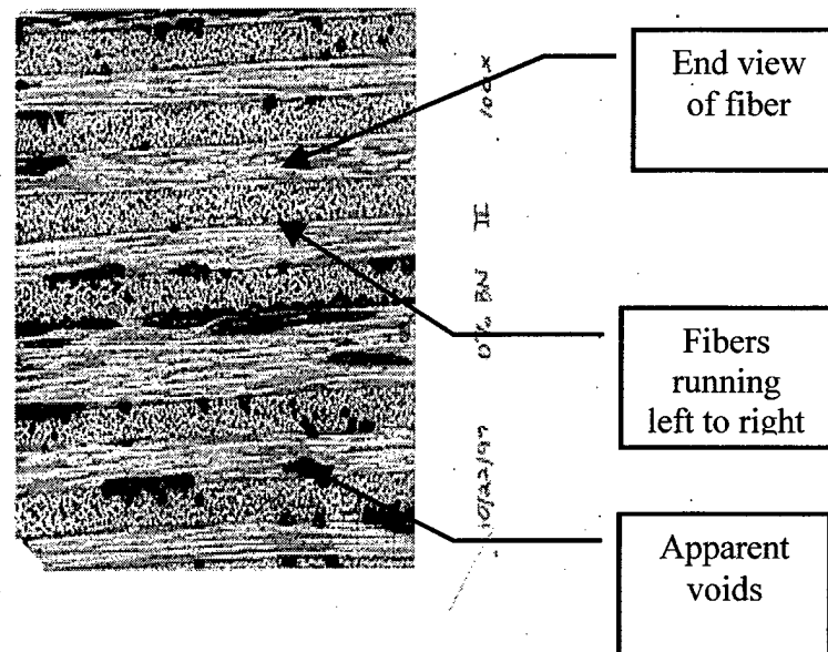
Figure 12. Sample showing 0% BN fill
