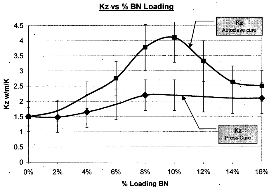
Figure 4. Kz for press and autoclave cured laminates
