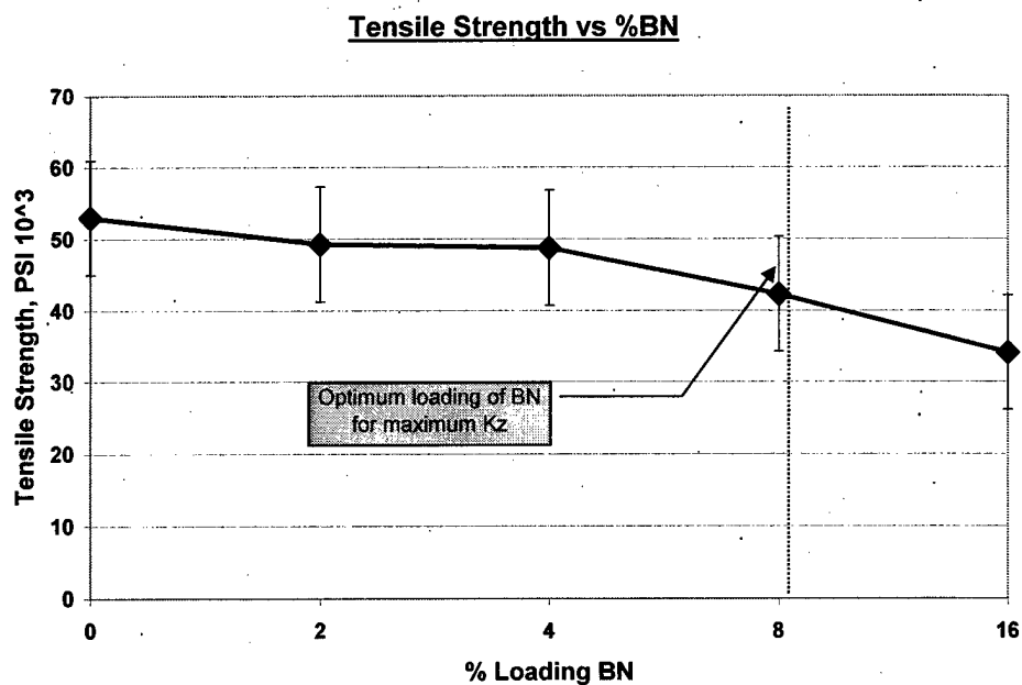
Figure 8. Tensile strength
