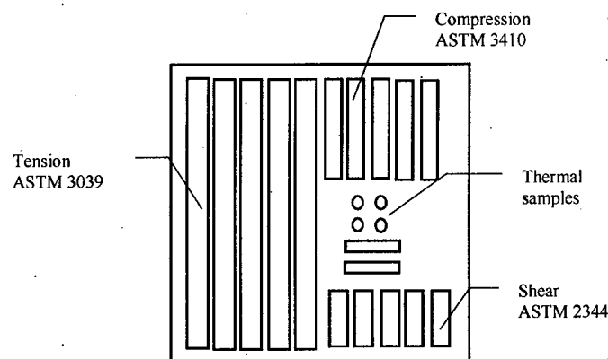
Figure 11. Layout of samples on 12" square test panel
