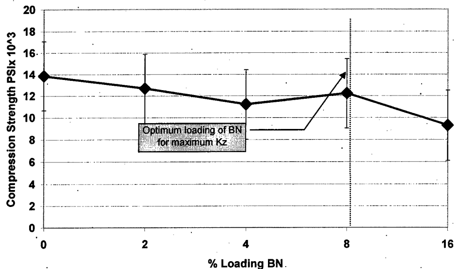
Figure 9. Compression strength
