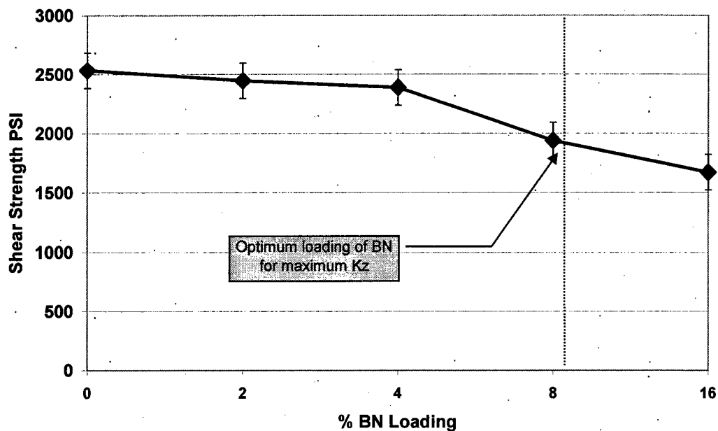
Figure 10. Shear strength
