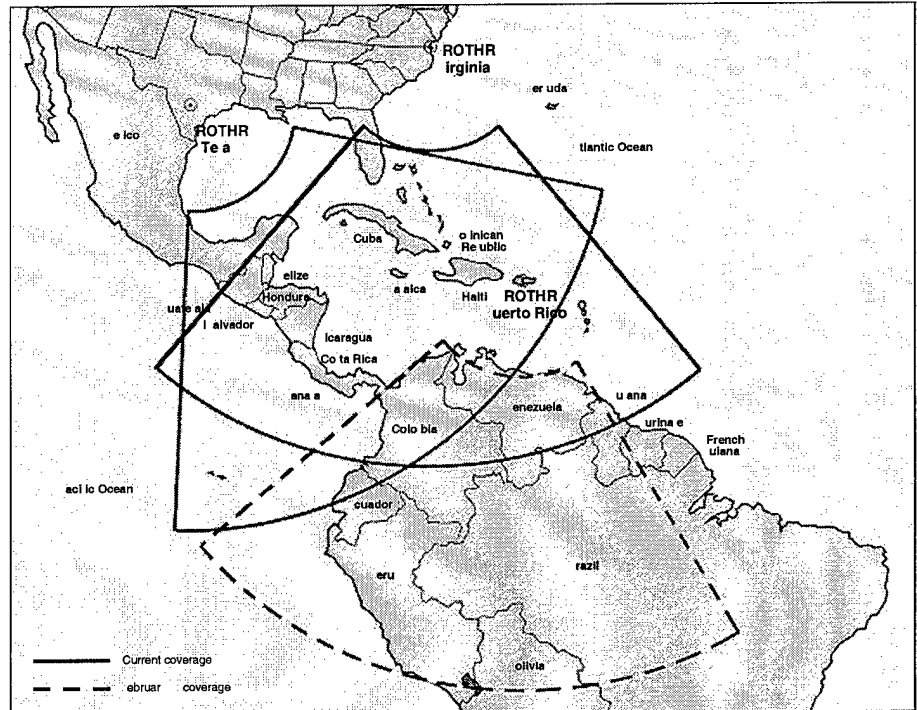
Figure 8: Relocatable Over-The-Horizon Radar Coverage
