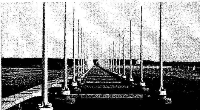
Relocatable Over-The-Horizon Radar (Receiver site antennas)
