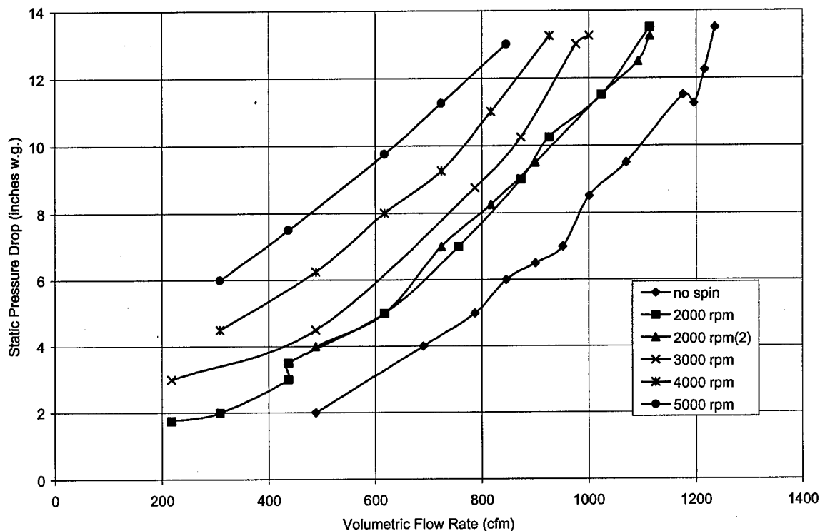
FIGURE 14. Pressure Drop vs. Flow Rate for the 800-ACFM BLMT Filter at Incremental Disk Spin Rates
