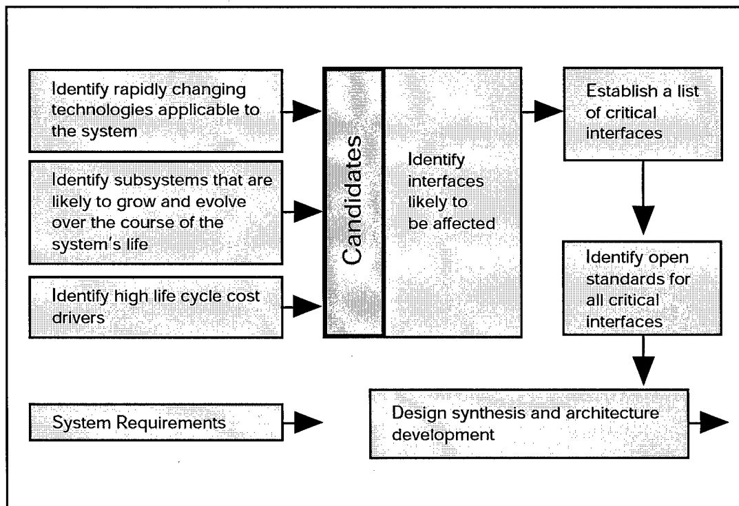
Figure 3. Open Systems Analysis for Integrated Design Solution
