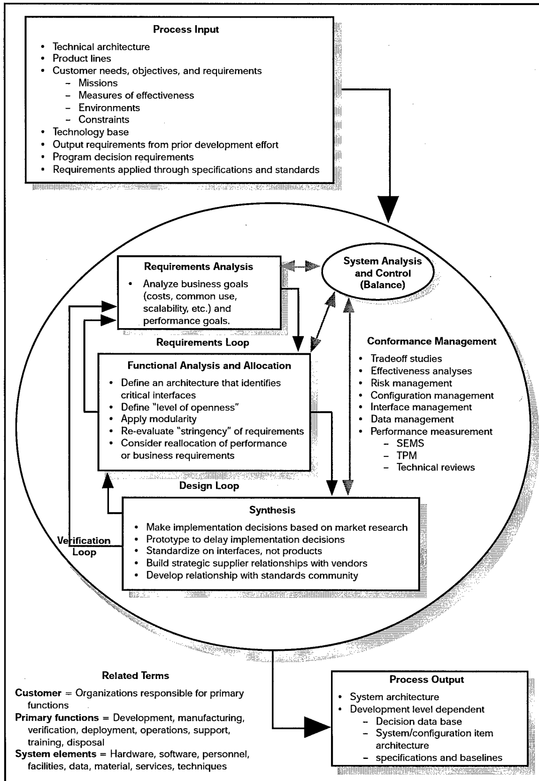
Figure 4. Integrating Open Systems and the Systems Engineering Process
