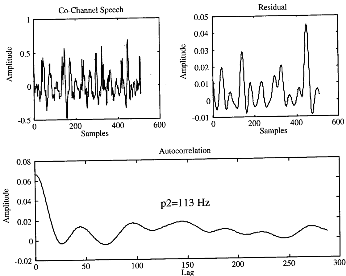
Figure 3.16: Modified autocorrelation pitch estimation on overlapping vocalic speech at SIR = -6 dB. Pitch estimated at 113 Hz.
