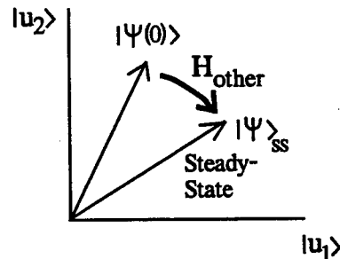
Figure 5.1.2: \hat{H}_{\text{other}} causes a disturbed wave function to relax to steady state.
