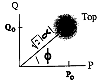
Figure 4.3.5: The amplitude and phase of the Wigner distribution.
