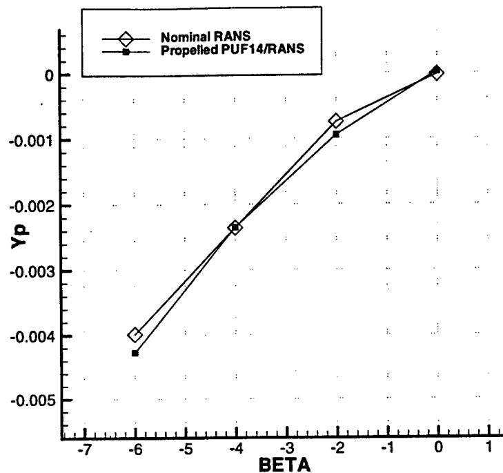
Figure 9-5: Lateral Force
