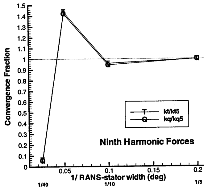
Figure 7-12: Convergence of K_T and K_Q for mean and 9th harmonic rotor forces versus RANS-stator width.
