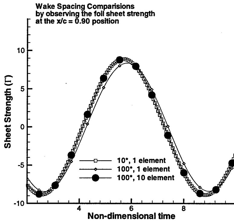
Figure A-5: Vortex sheet strength behavior at x/C = 0.9 on the foil in a sinusoidal gust. Using a non-dimensional time step of 100^* with N_f = 10 vortices in the first interval yields similar results as a time step of 10^* and no subdivision.
