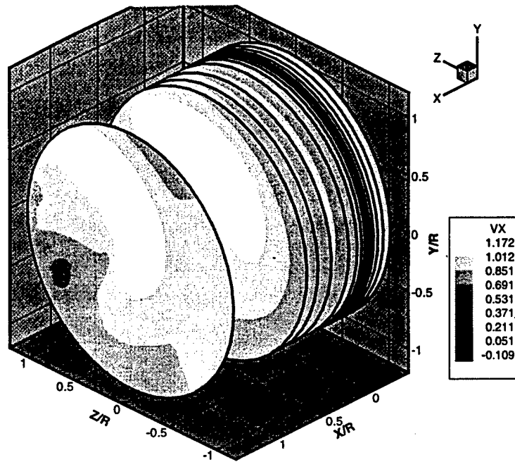
Figure 8-5: This figure shows the total inflow at every 3 rd velocity disk.
