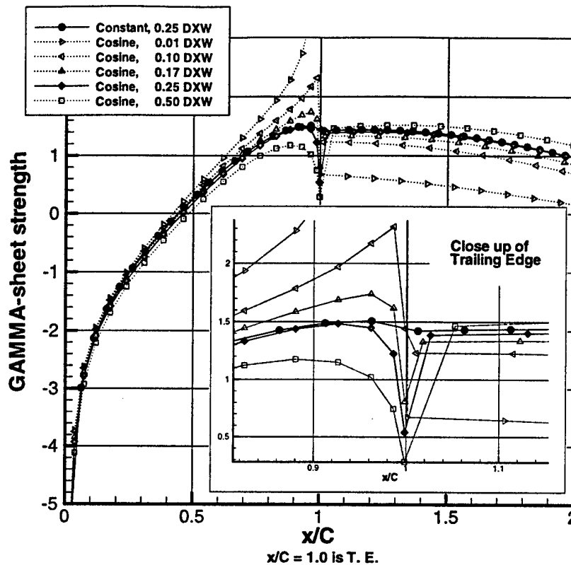
Figure A-2: Trailing edge behavior of the vortex sheet strength.
