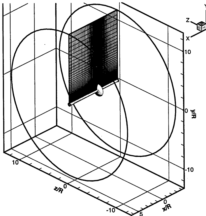
Figure 7-1: Straight-shaft RANS grid, grid outline, and the swept volume of propeller 4119
