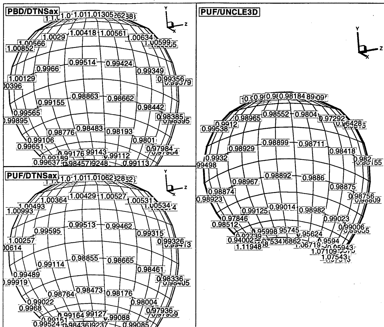
Figure 7-3: Away from hub and tip effects, the axial effective inflow for propeller 4119 on a straight shaft should be equal to 1.0.
