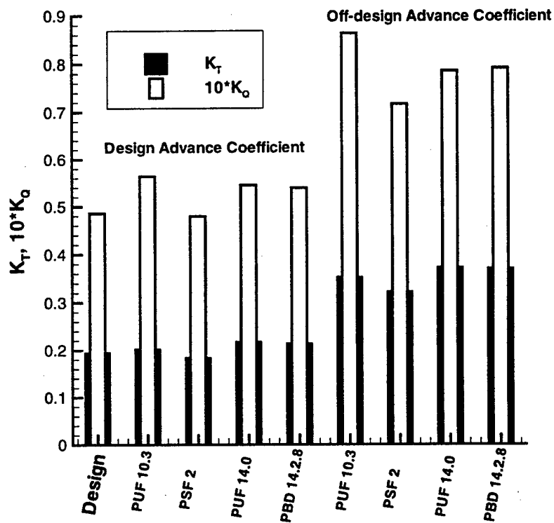
Figure 5-19: Propeller 4679 mean K_T and K_Q for the design J_S = 1.078 and an off-design J_S = 0.719 .
