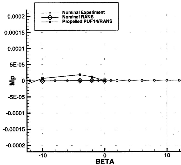
Figure 8-17: Pitch moment when in yaw.
