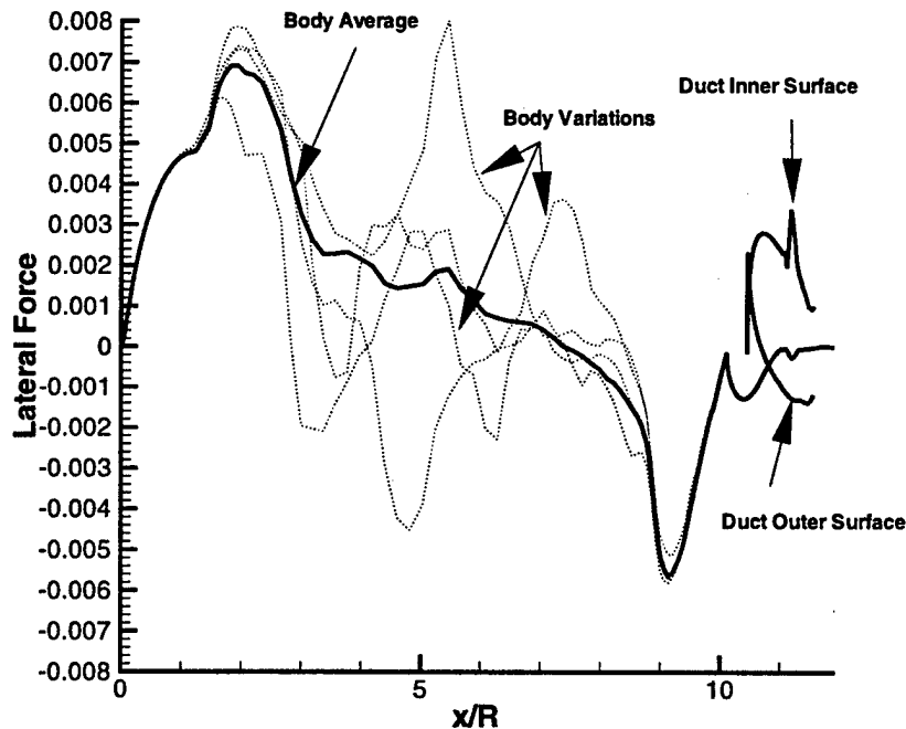
Figure 9-4: Lateral force ( F_z ) verses body position
