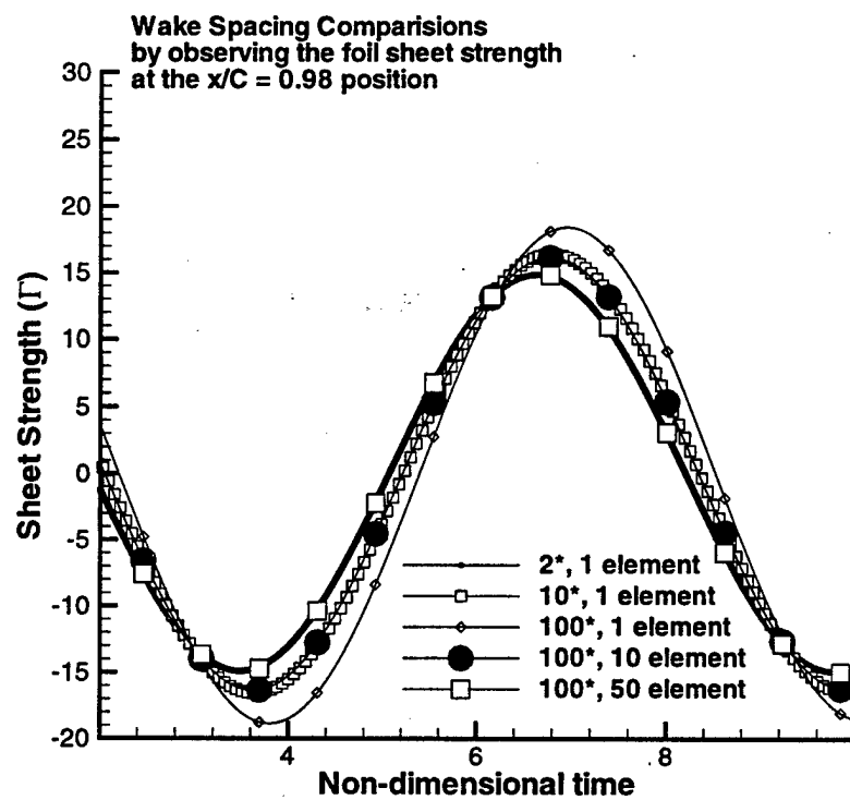
Figure A-6: Vortex sheet strength behavior at x/C = 0.98 on the foil in a sinusoidal gust. The new formulation converges to similar accuracy while using significantly larger time elements in the wake.
