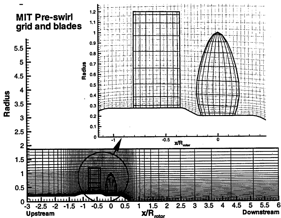
Figure 7-7: One meridional plane of the RANS grid is shown with the stator and rotor blades overlayed. The three-dimensional RANS grid is formed by revolving this meridional plane about the X-axis.
