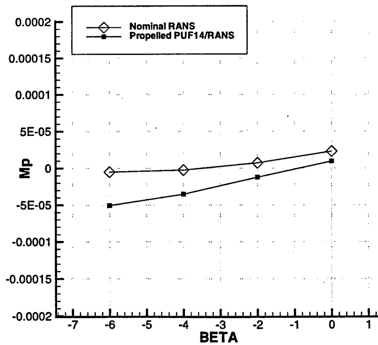
Figure 9-8: Pitch moment when in yaw.
