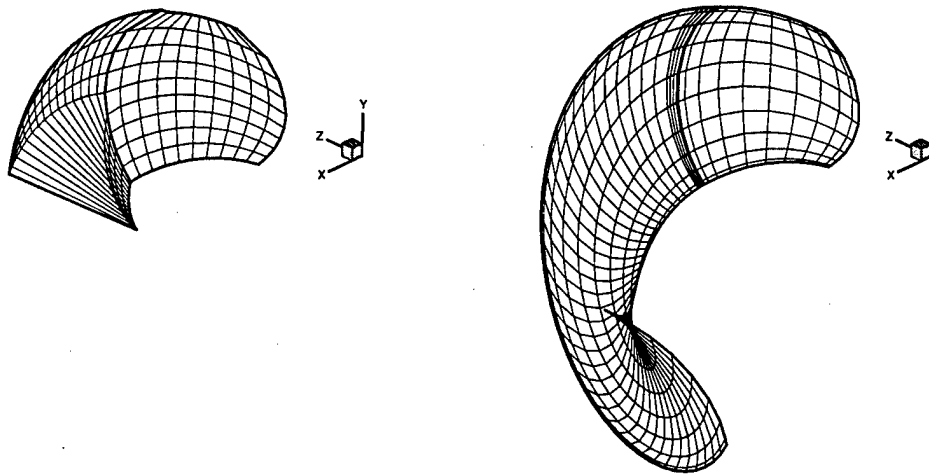
Figure 5-8: The leftmost figure shows PUF-2.1 key blade and transition wake lattice arrangement. The rightmost figure shows PUF-14 key blade and transition wake lattice arrangement. Differences in lattices lead to differences in solved blade circulation shown later.
