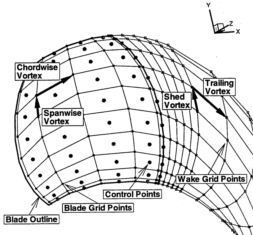
Figure 3-3: This figure shows the blade grid and wake grid points connected by a mesh. The blade control points are also shown. The boundary value problem solves for the blade circulation distribution which simultaneously nulls the normal velocity at every control point on every blade surface.
