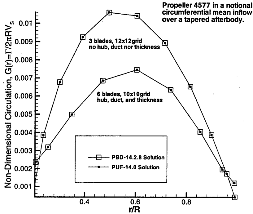
Figure 5-7: Comparison of the Non-Dimensional Circulation versus Radius
