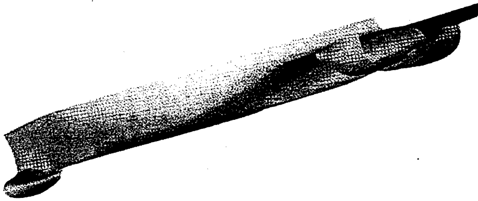
Figure 1-2: Notional surface ship underwater hull form with an integrated propulsor concept (Developed at NSWC under the electric drive program.)
