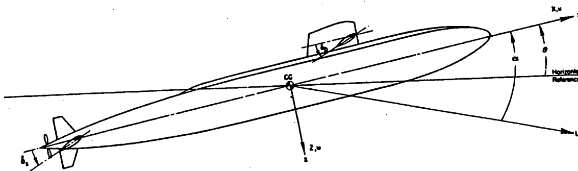
Figure 1-5: Typical steady inflow during depth transient is at an angle \alpha with respect to the body centerline.
