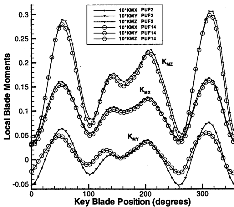
Figure 5-11: Comparison of the PUF-14 and PUF-2.1 moment analysis
