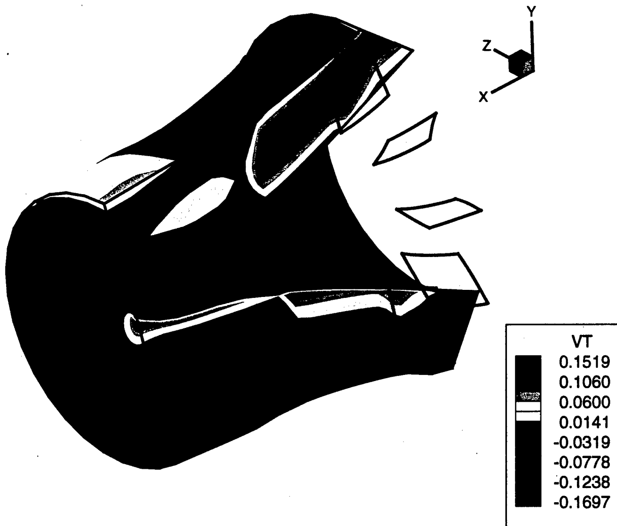
Figure B-3: This figure shows the volume used to perform the stator analysis. This case is at 4^\circ drift angle. Tangential velocity is shown in the contour (see section 9.2)
