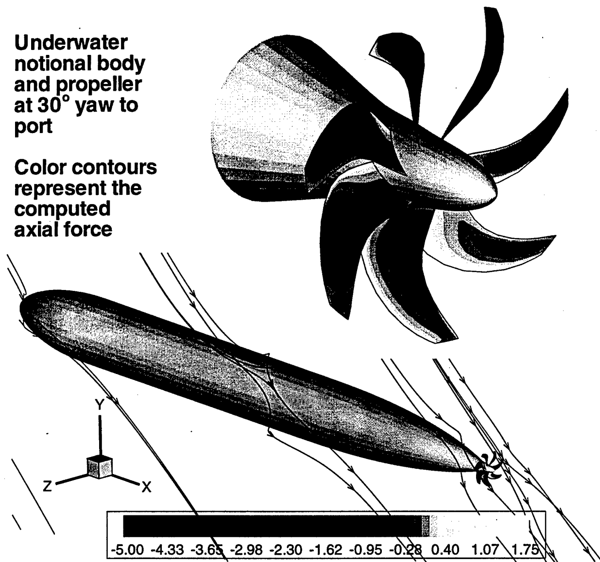
Figure 8-10: Huang body 1 coupled lifting-surface/RANS solution (Color reproduction in figure B-2.)
