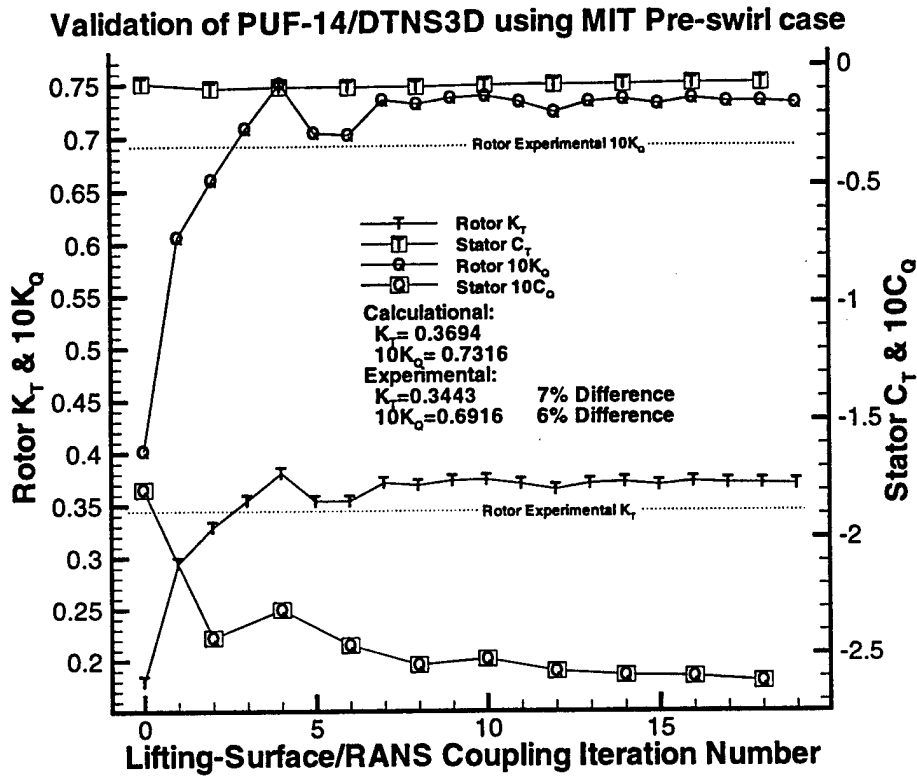
Figure 7-8: Computed MIT Pre-swirl force coefficients versus coupling iterations.
