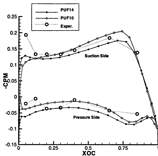
Figure 5-13: Mean pressure distribution on one blade of DTMB 4679 at r/R = 0.7 for the design J_S of 1.078.
