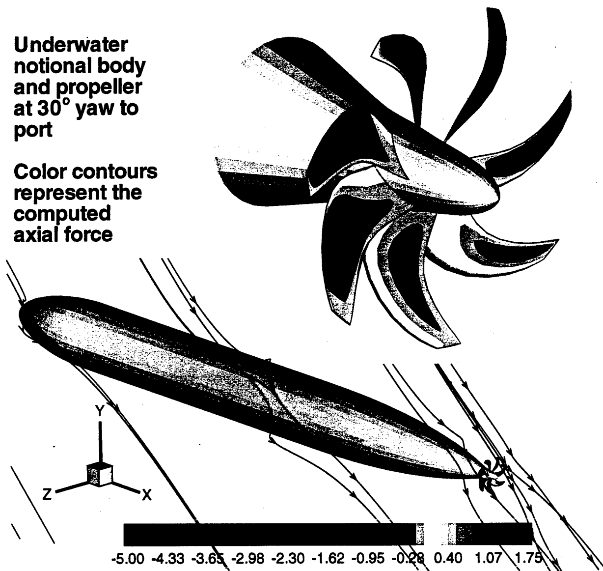
Figure B-2: Huang body 1 coupled lifting-surface/RANS solution (see section 8.4)
