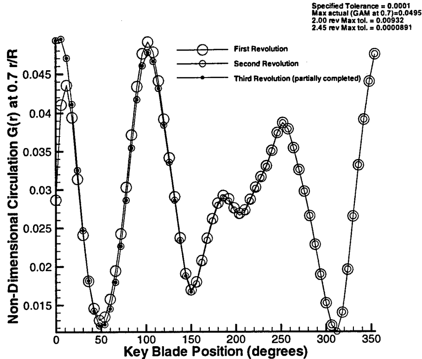
Figure 5-2: The solved circulation is shown for the entire time domain solution calculated by PUF-14. Note that only the converged solution correctly represents the boundary value problem.
