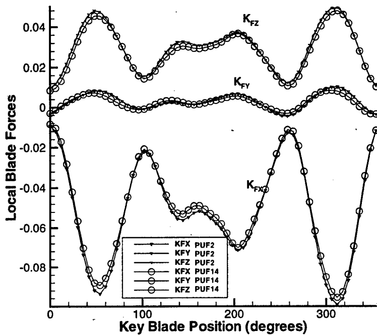
Figure 5-10: Comparison of the PUF-14 and PUF-2.1 force analysis
