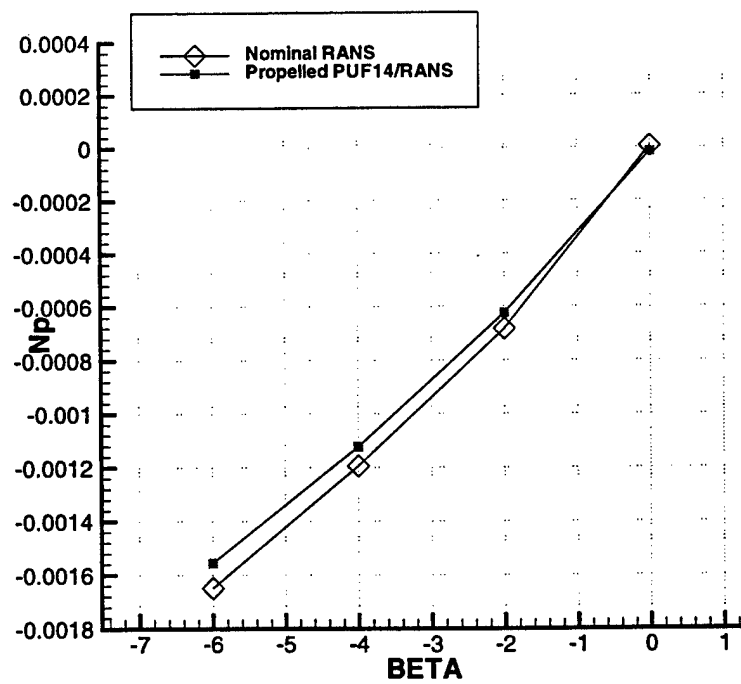
Figure 9-6: Yawing Moment
