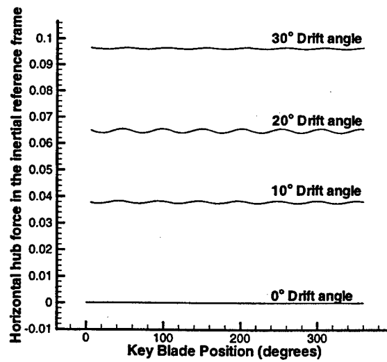
Figure 8-12: Force trends on the shaft in the inertial coordinate system associated with the varying drift angles.
