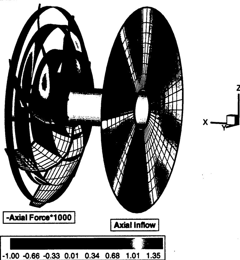
Figure B-1: This figure shows a notional inflow with the corresponding time-average forces in the swept volume of the rotor (see section 6.3.3).
