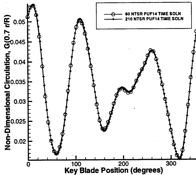
Figure 5-4: Comparison of two angular sizes of the time step, N_\theta
