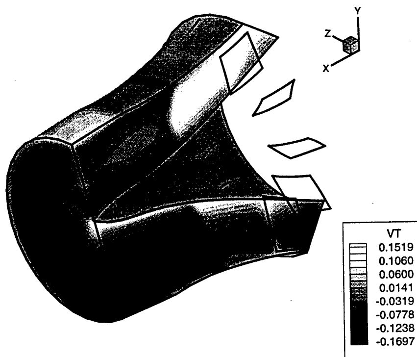
Figure 9-1: This figure shows the volume used to perform the stator analysis. This case is at 4^\circ drift angle. Tangential velocity is shown in the contour (Color reproduction in figure B-3).
