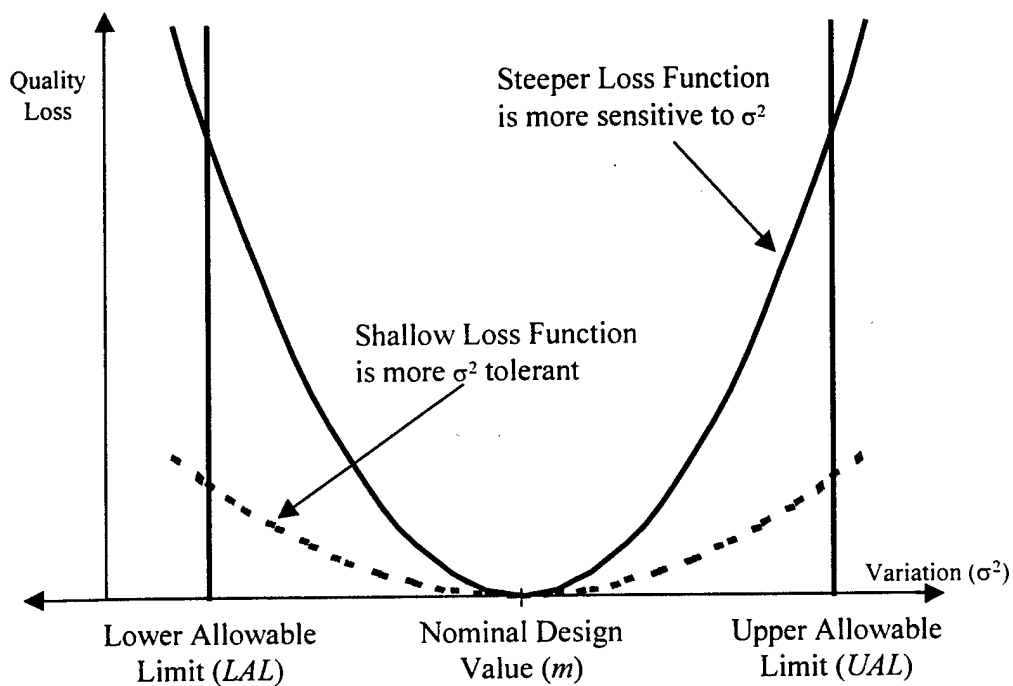
Figure 2: Taguchi Quality Loss Function
