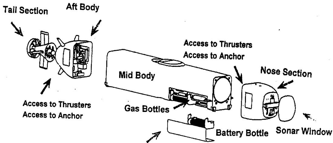
Figure 1-1: External Isometric View of the ASDS
