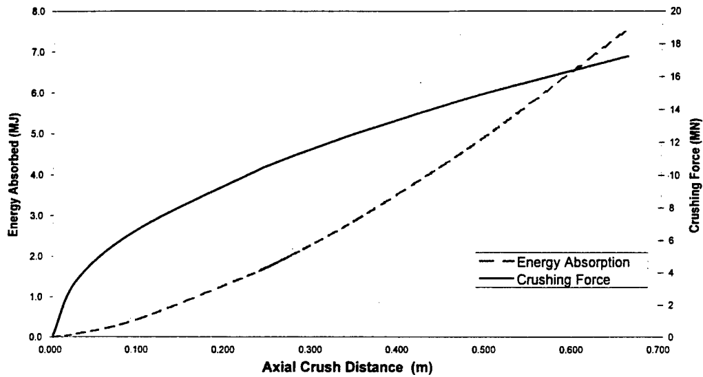
Figure 3-10: Crushing Force and Cumulative Energy Absorption for the Forward Pressure Hull Hemi-head.
