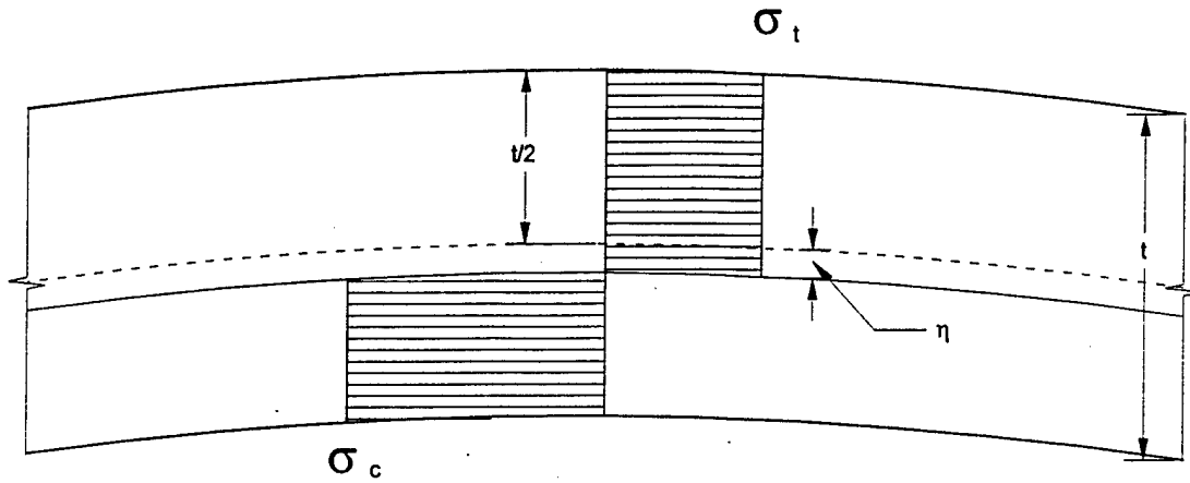
Figure 2-2: Membrane Stress and Fully Plastic Bending Moment Representation for Material having Differing Compressive and Tensile Flow Stresses.
