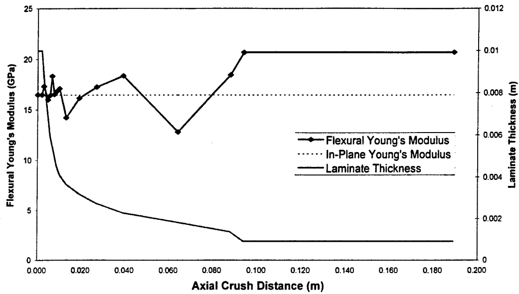
Figure 3-7: Flexural Young's Modulus and Laminate Thickness Variation with Axial Crush Distance of the Frustum Section.
