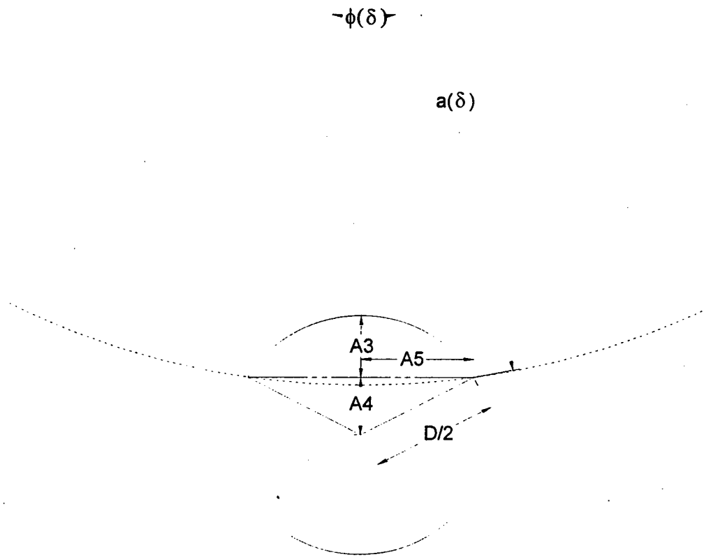
Figure 2-8: Geometrical Relationship of Parameters Used in the Derivation of the Correction Factor for Open Sections in a Dome Structure (top view).
