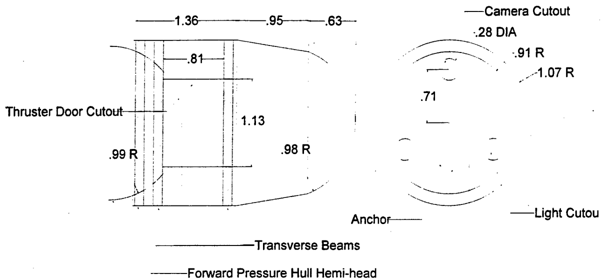
Figure 3-2: Model of ASDS Forward Section (Dimensions in meters).
