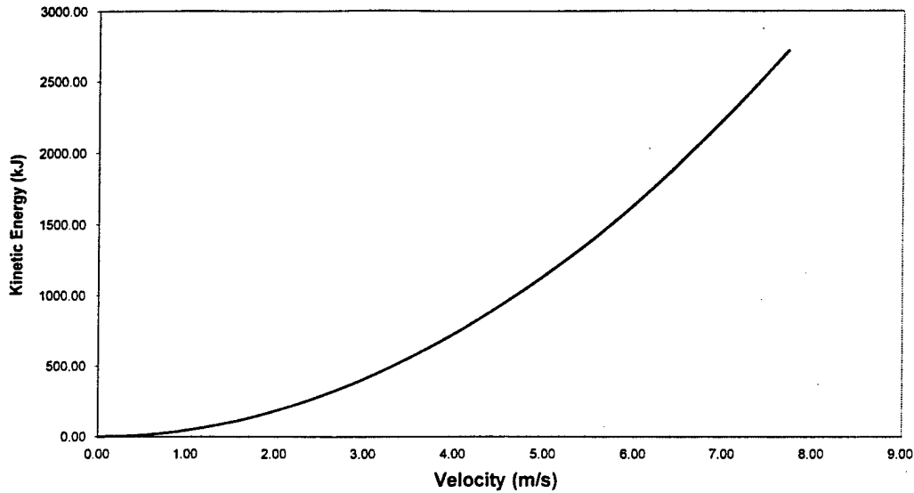
Figure 3-13: Vehicle Kinetic Energy for Various Speeds.
