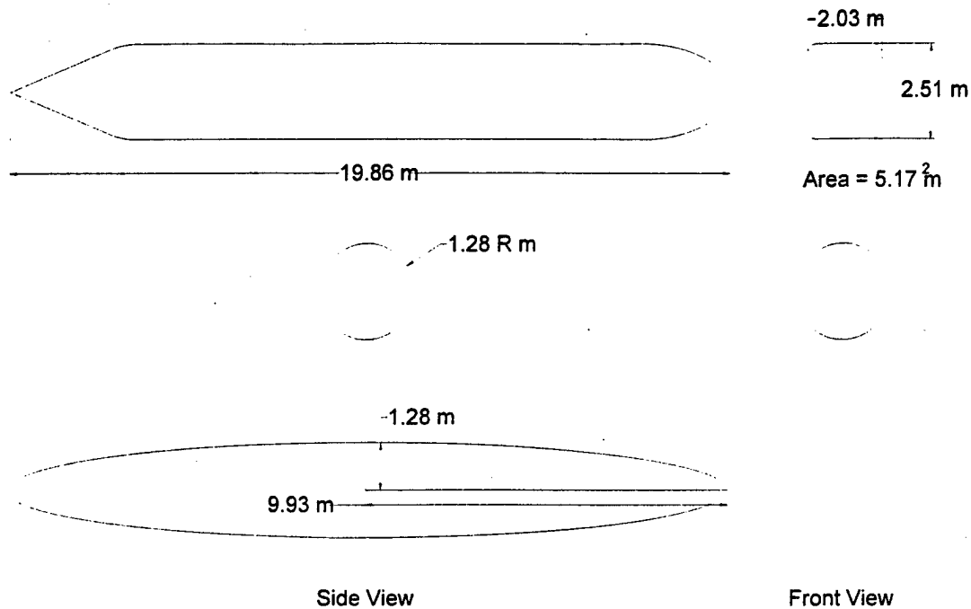
Figure 3-12: Dimensions Used During Added Mass Calculations
