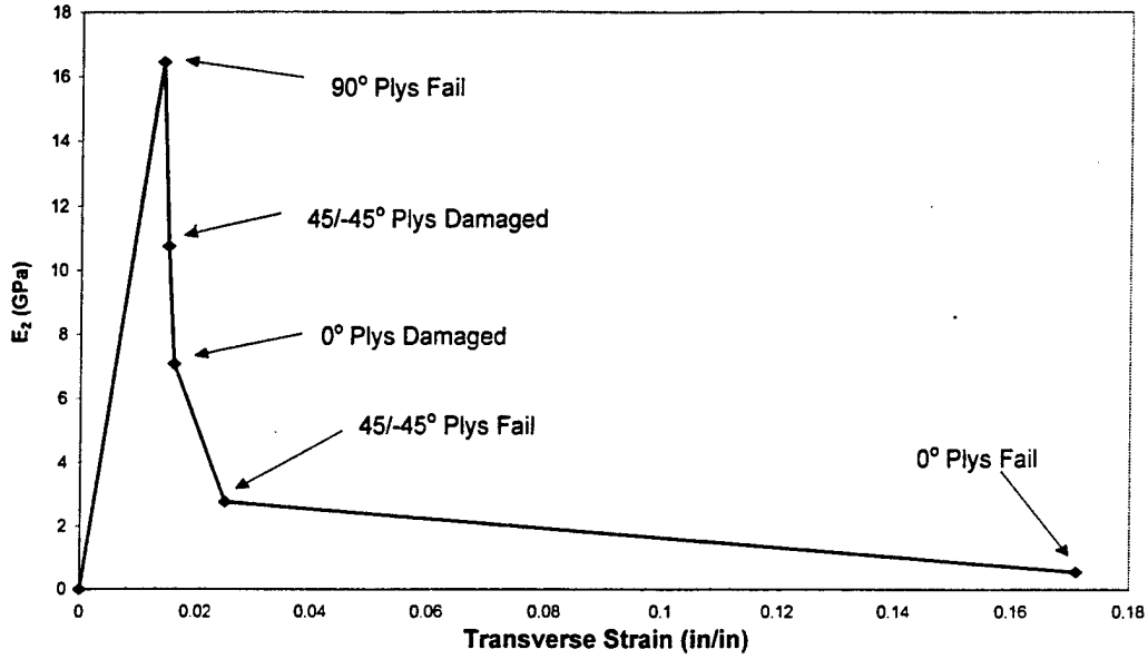
Figure 3-5: Transverse Young's Modulus Variations with Pure Tensile, Transverse Strain for Frustum Section.
