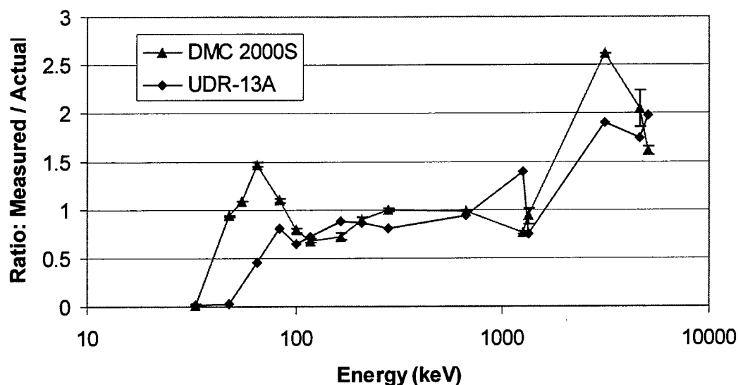
Figure 3: Relative response of the dosimeters as a function of gamma-ray energy. The UDR-13A shows a more or less monotonic dependence on energy, whereas the DMC 2000S exhibits a more exotic energy dependence.
