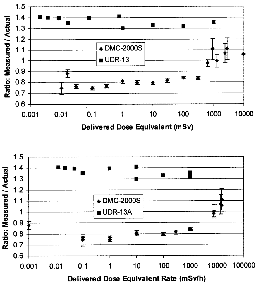
Figure 2: As for the previous figure, but for ^{60}\text{Co} . The DMC 2000S over-responds at very high dose rates.
