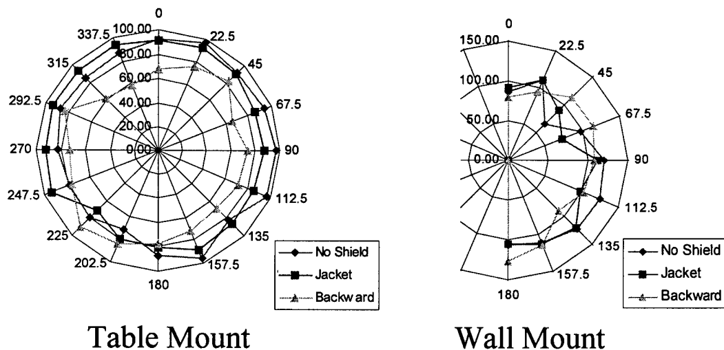
Figure 5: Range of dosimeter-reader communication for table- and wall-mounted readers, using no shielding, a flak jacket, or a human body for shielding. Ranges are indicated by the distance from the centre of the radar plot. The range axis is labelled in centimetres.
