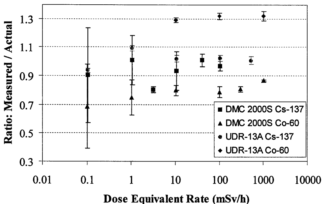
Figure 4: Fluctuations in the reported dose rate from the dosimeters, for ^{137}\text{Cs} and ^{60}\text{Co} sources. The error bars indicate the range of dose rates measured over a period of one to two minutes.
