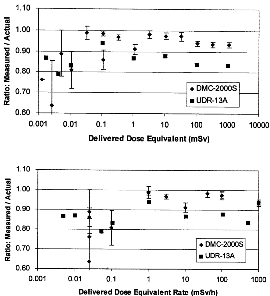
Figure 1: Ratio of measured dose to delivered dose as a function of delivered dose (upper panel) and dose rate (lower panel), from a ^{137}\text{Cs} source. The DMC 2000S appears to under-respond slightly at low dose rates.
