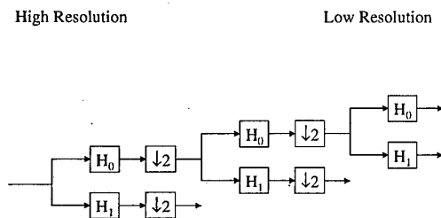
Fig. 2. Multiresolution Filter Bank
