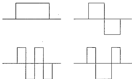
Fig. 8. Walsh functions
