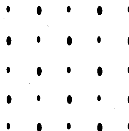
Fig. 6. Non-separable grid
