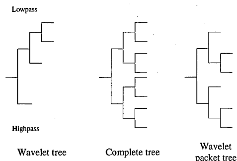
Fig. 7. Dyadic tree structures
