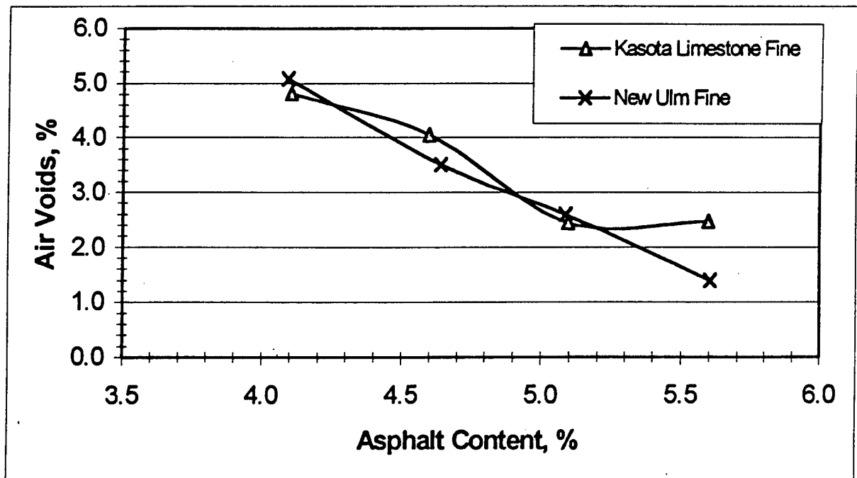
Figure 4.3 Air Voids vs Asphalt Content for PG 58-40 Mixes
