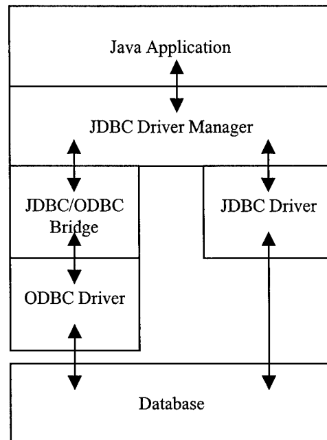
Figure 4-13. JDBC Connectivity
