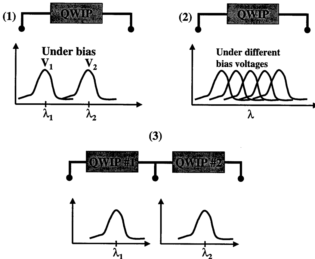
Figure 1 Three different multicolor QWIP approaches: (1) The QWIP has a response peaked at \lambda_1 at voltage V_1 and at \lambda_2 at voltage V_2 ; (2) The QWIP has a response that is continuously tuned by voltage; and (3) shows two QWIPs with different response wavelengths grown in a multi-stack. Intermediate leads are provided so that each QWIP functions independently.
