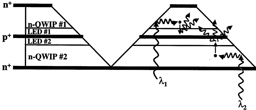
Figure 7 Schematic showing the structure #1 of a two color, three-lead QWIP-LED device.
