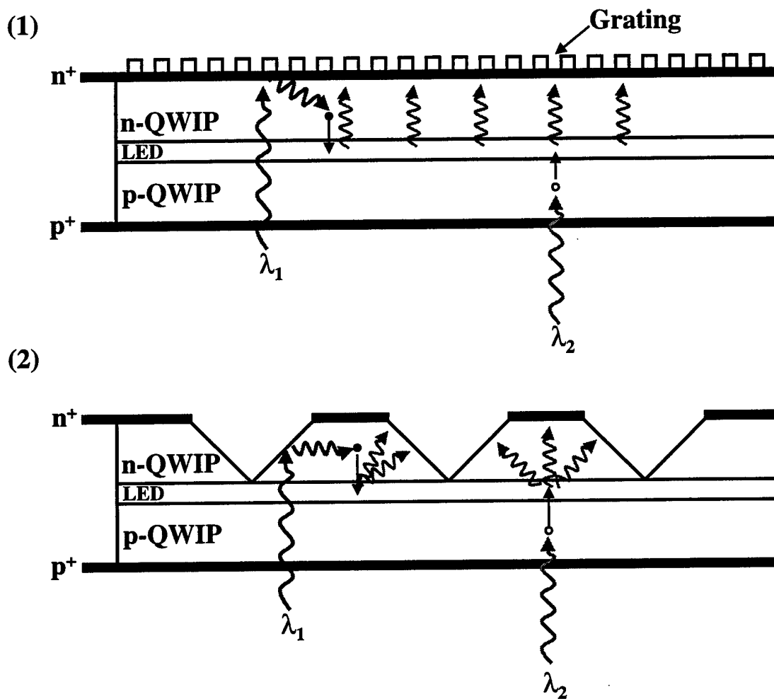
Figure 3 Implementation of a two-lead bicolor QWIP-LED focal plane with either (1) a 2-D grating or (2) a V-groove coupler.
