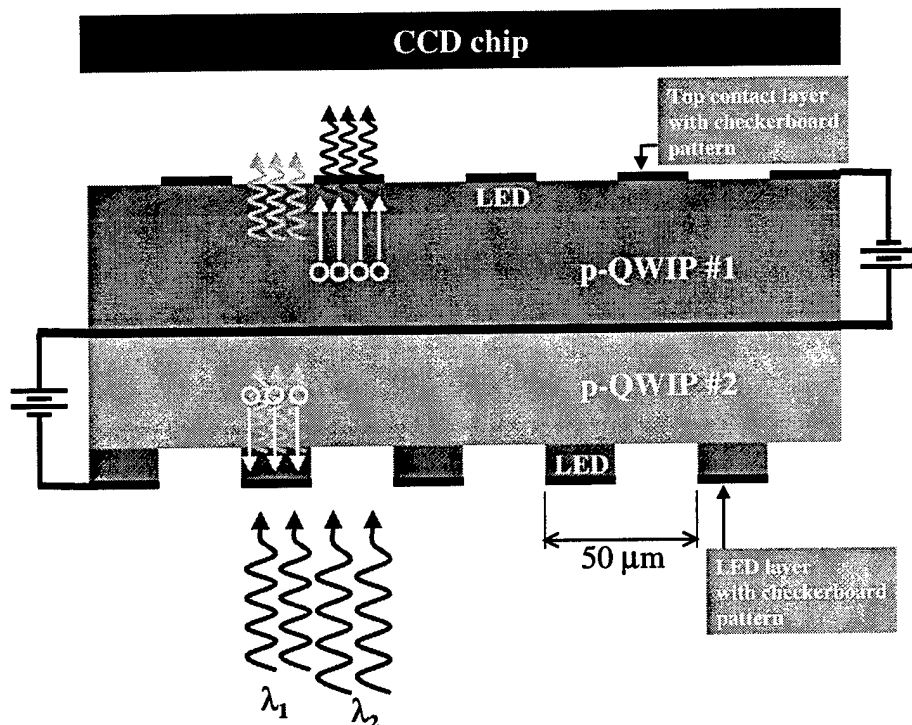
Figure 15 Shown on the top QWIP-LED stack is the top contact layer with checkerboard pattern so that only areas with the contact layer will have the bias voltage to induce photocurrent. The bottom QWIP-LED stack has similar built-in checkerboard implementation except the pattern is built into the LED layer. Similarly for n-type QWIPs the same can be patterned into the grating layer.
