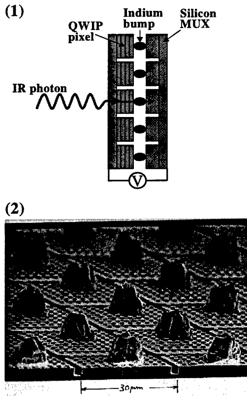
Figure 6 (1) Schematic of a QWIP-MUX array (side view); (2) An SEM picture showing QWIP array with pixels in the size of 30\mu\text{m} \times 30\mu\text{m} , and Indium bumps on them [19].
