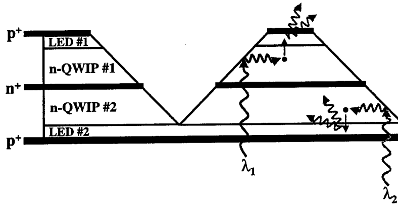
Figure 8 Schematic showing the structure #2 of a two color, three-lead QWIP-LED device.
