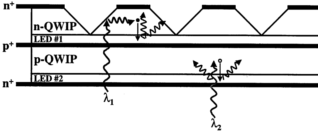
Figure 10 Schematic showing the layer structure of QWIP-LED architecture #4 with a V-groove coupler. A 2-D grating can also be used in place of V-grooves.
