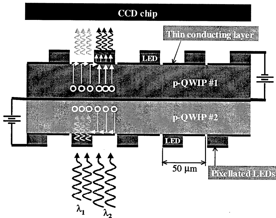
Figure 16 Implementation of a bicolor QWIP-LED focal plane with built-in checkerboard for spatial waveband separation. Near 100% fill factor can be accomplished using this architecture.
