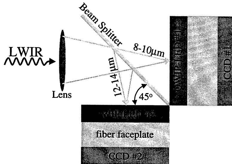
Figure 18 The incoming IR images are separated according to their wavelengths by a waveband beam splitter placed exactly at 45° with respect to the two QWIP-LED focal planes.
