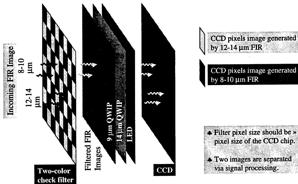
Figure 11 Implementation of a bicolor QWIP-LED focal plane with an external checkerboard bicolor filter.
