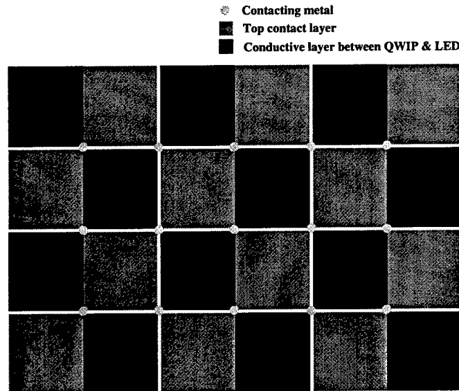
Figure 17 A bicolor QWIP-LED focal plane array with checkerboard pattern etched into the top contact, the LED, and the intermediate thin conductive layers. The rectangular QWIP-LED pixels are connected to each other at the top contact layer by metal deposits.
