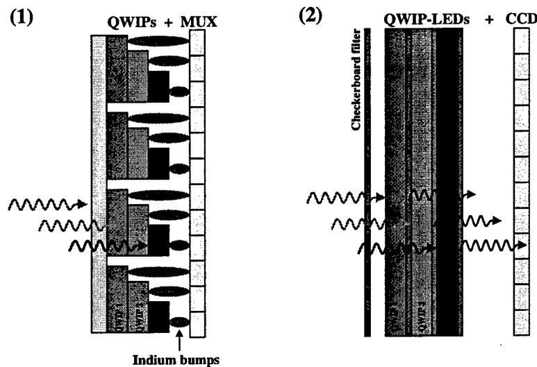
Figure 13 Comparison of a tricolor QWIP-LED device with a QWIP-MUX array: (1) Fill factor is dependent on indium bump contact areas; (2) Fill factor is inversely proportional to the number of colors.
