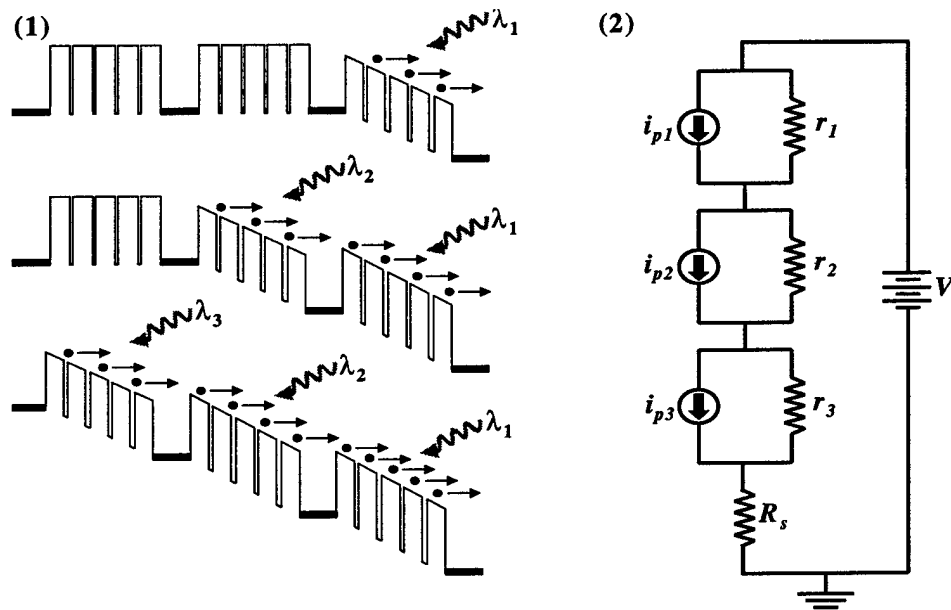
Figure 2 (1) Bandedge profile of a three-color detector at different bias voltages. The top part is for a small voltage where only the highest resistance one-color QWIP (at \lambda_1 ) is turned on; the middle part is appropriate for the situation where two of the three one-color QWIPs (at \lambda_1 and \lambda_2 ) contribute to the photocurrent; and in the lower part the applied voltage is high enough so that all three one-color QWIPs (at \lambda_1 , \lambda_2 and \lambda_3 ) are turned on. (2) Model equivalent circuit of a three-color detector biased through a series load resistor.
