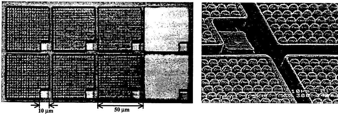
Figure 14 SEM pictures of a bicolor QWIP focal plane array showing part of top QWIP layer removed to make room for contacting the intermediate contact layer [19].
