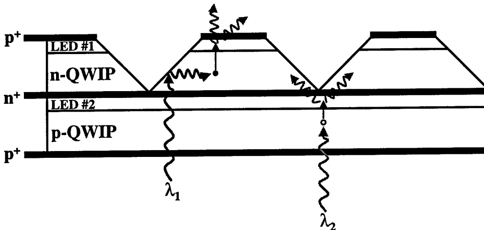
Figure 9 Schematic showing the layer structure of QWIP-LED architecture #3 with a V-groove coupler. A 2-D grating is preferred over the V-grooves for this layer structure.
