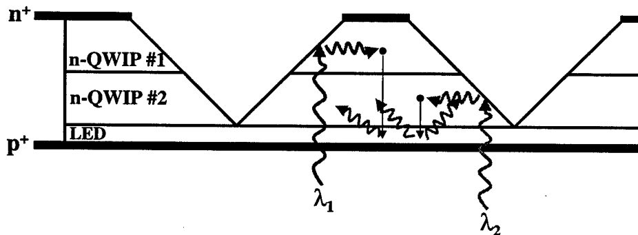
Figure 4 Implementation of a two-lead bicolor QWIP-LED focal plane using the two-lead architecture #2.
