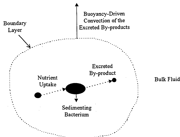
Figure 4-5 Graphical Representation of Proposed Model. As a bacterium consumes nutrients and excretes by-products, the medium immediately surrounding the cell becomes less dense than the bulk fluid. This creates buoyancy-driven convection of the excreted by-products.
