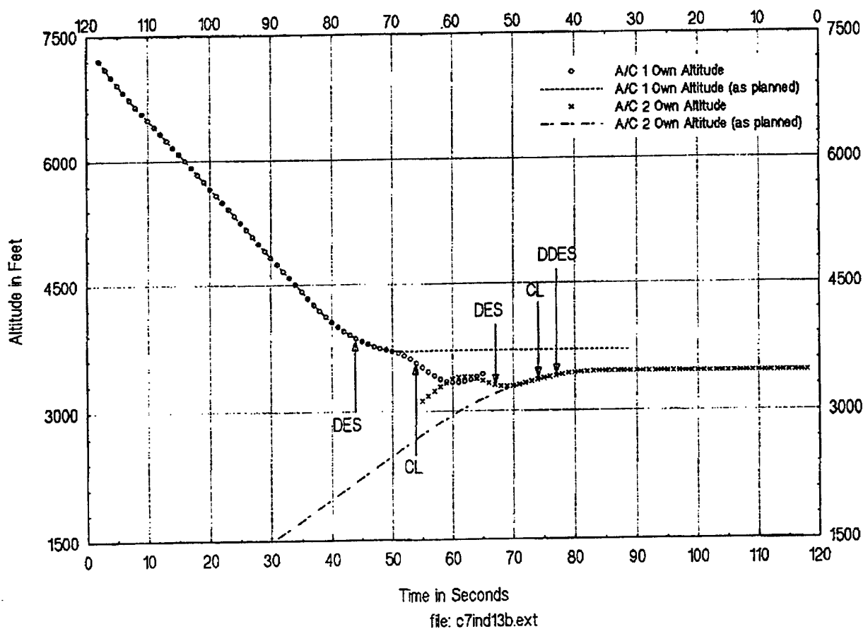
Figure 2-10. Encounter Summary – Aircraft Altitudes. Data file name = CL8B1_N.DAT, REIT Number = 1541, Sim Mode = 1271033.
