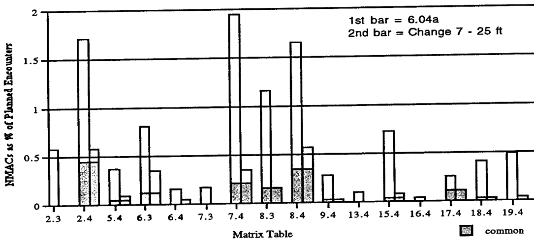
Figure 4-4. NMAC Comparison 6.04a vs. Change 7 25-foot tracker.
