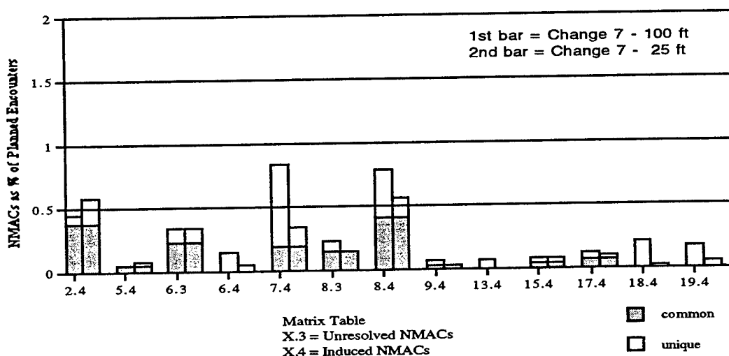
Figure 4-5. NMAC Comparison Change 7 100-foot tracker vs. Change 7 25-foot tracker.
