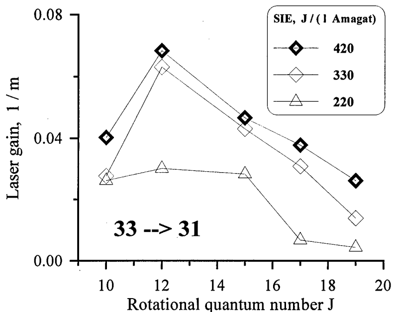
Fig.3.7. Laser gain on 33 \rightarrow 31 vibrational transition vs. rotational quantum number for various SIE.
