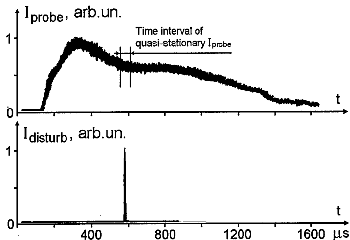
Fig.3.13. Experimentally obtained time behaviors of probe and perturbing laser pulse intensities.
