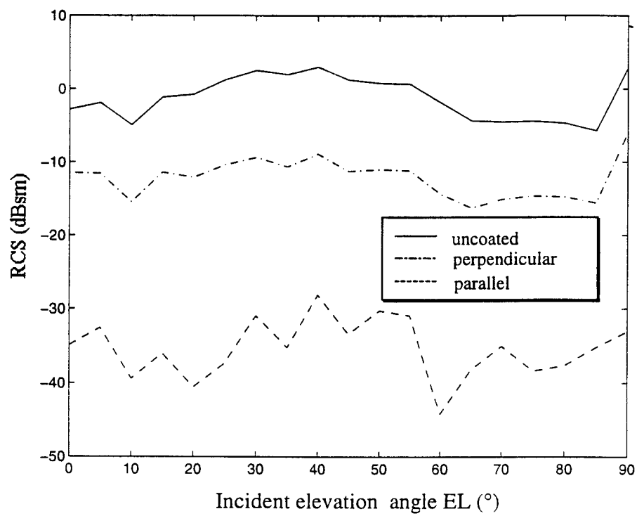
(a) H-polarization
