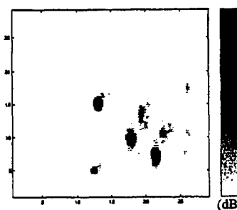
Fig.2(c) ISAR image generated from interpolated result using AFE with 200 calculated points.
