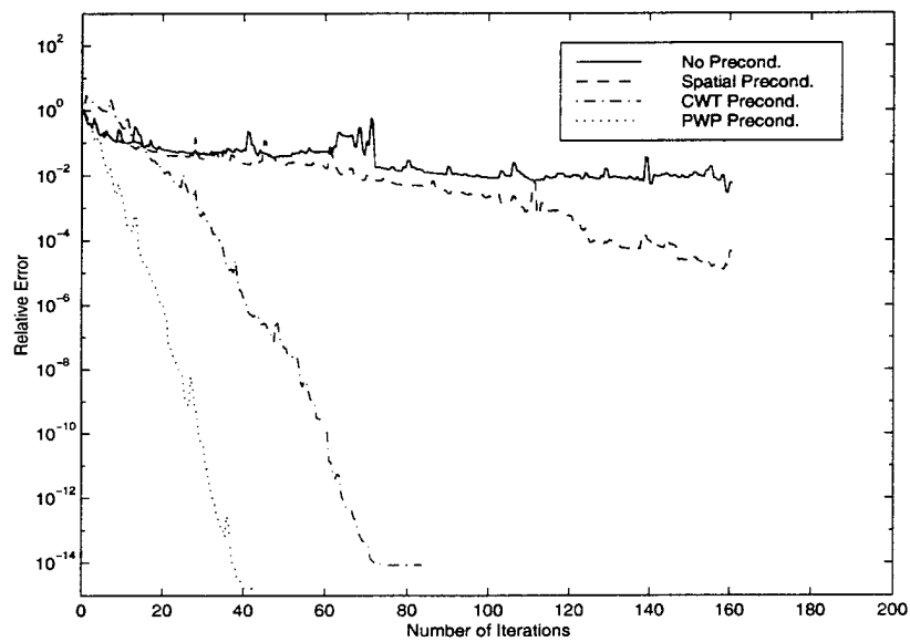
Figure 6. Convergence behaviors of the preconditioned systems versus iteration numbers for PWP and other preconditioning methods in (a) Case 1, (b) Case 2, and (c) Case 3 with N=512 .
