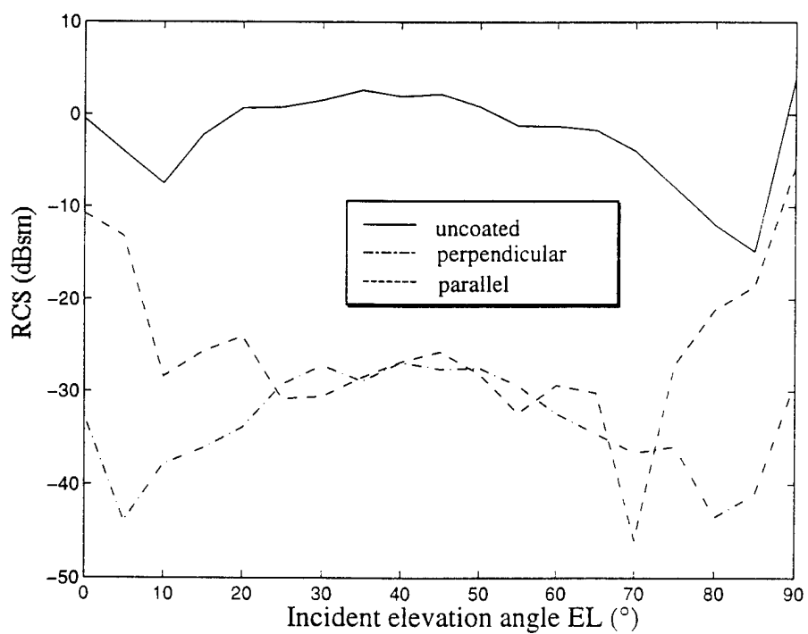
(b) V-polarization
