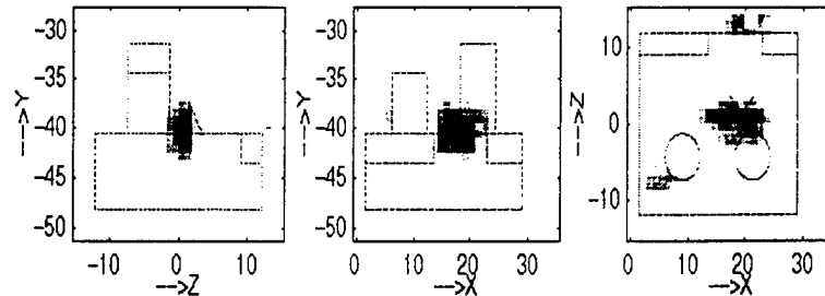
Figure 11. 2-D projected ACSAR images based on frequency-aperture data, formed by first parameterizing the (R, u, v) image using CLEAN and reconstructing the image in the (x, y, z) platform coordinates.
