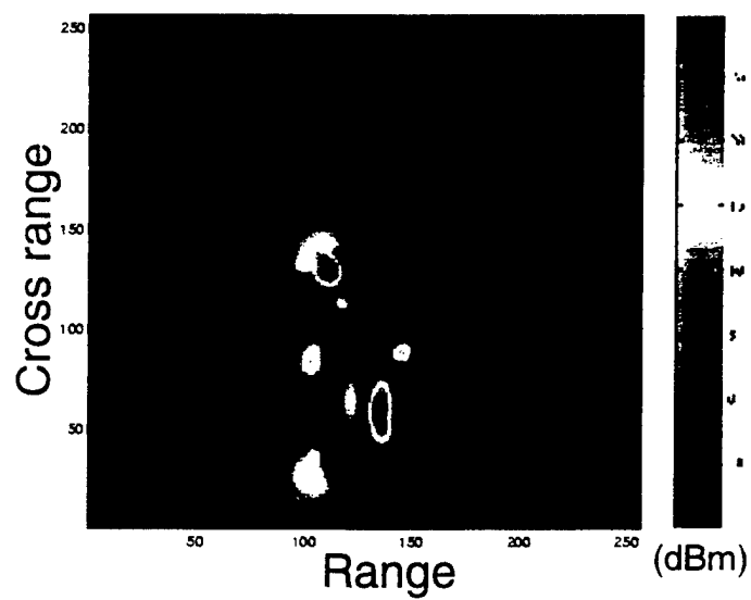
Fig.7 ISAR image generated from interpolated results using current-domain 2-D spline with 15 \times 15 = 225 calculated points.
