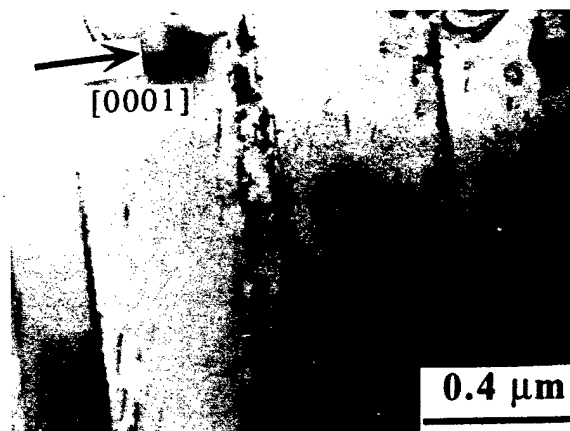
Fig. 3—Bright-field image of an area containing dislocation arrays. The specimen is close to the orientation where basal planes are in an edge-on position
