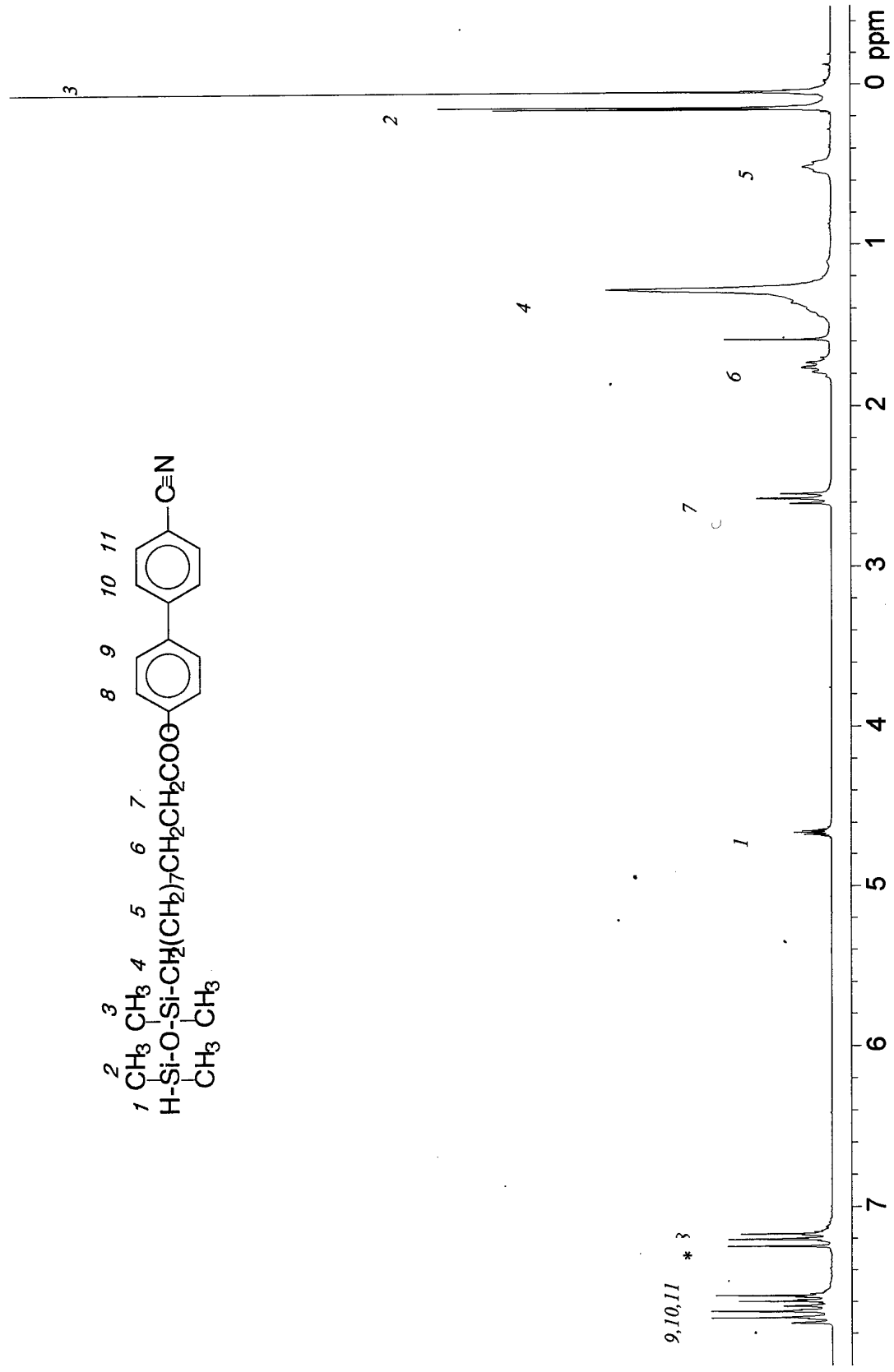
4) 250 MHz 1 H NMR spectra of the compound H-Si-Und-CB
