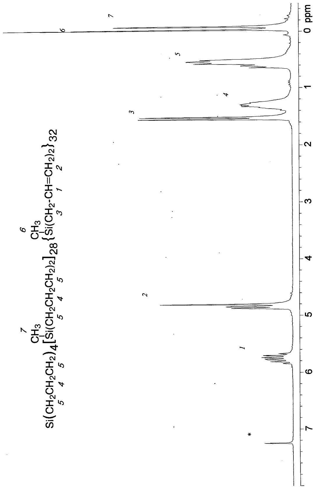
2) 250 MHz 1 H NMR spectra of the compound G-4(AII) 64
