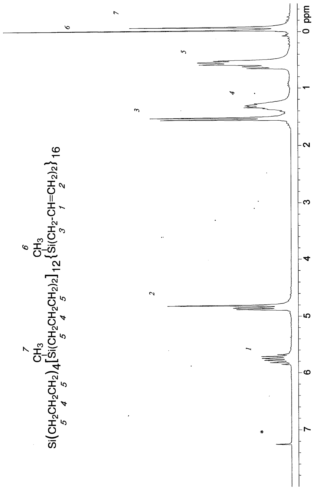
1) 250 MHz 1 H NMR spectra of the compound G-3(AII) 32
