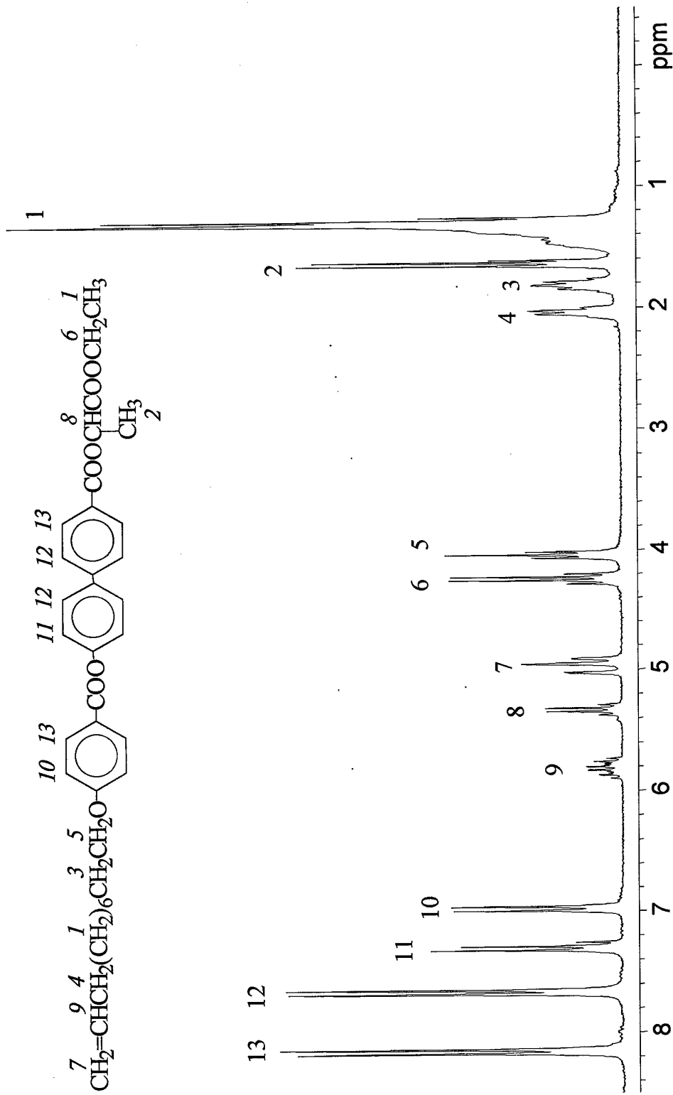
5) 250 MHz 1 H NMR spectra of the compound Und-PBL
