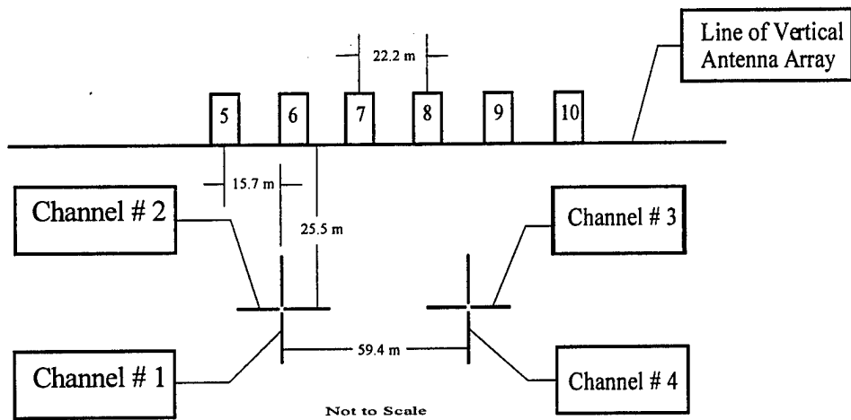
Figure 2 Receiving antenna configuration (top view)
