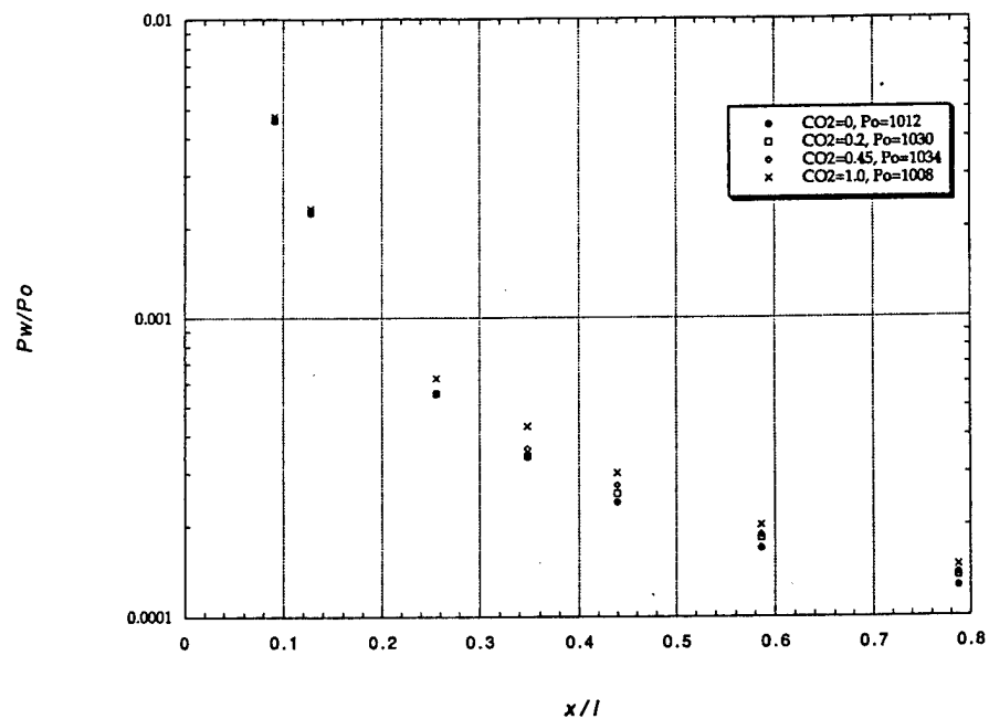
Figure 5. Nozzle pressure distribution. Pressure rise due to CO_2 seeding. Data averaged over multiple runs.
