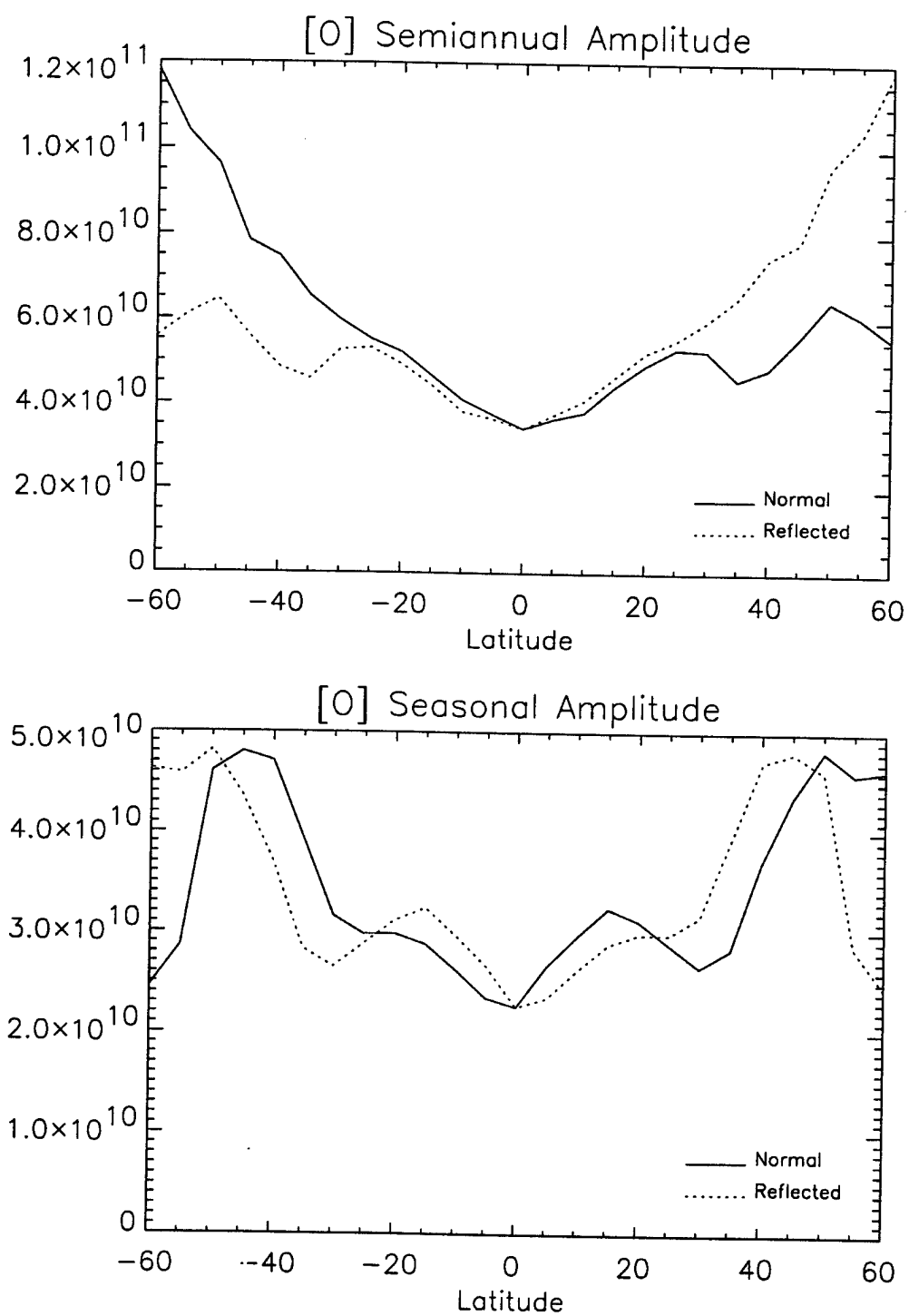
Figure 3. Latitude distribution (a) Semiannual and (b) Seasonal [\text{O}(^3\text{P})] amplitudes ( \text{cm}^{-3} )
