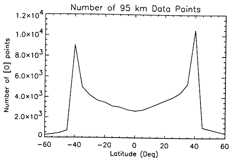
Figure 1. Latitude distribution of number of data points
