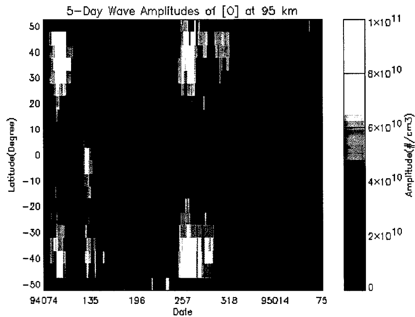
Plate 2: Latitude and time dependence of 5-Day wave amplitudes
