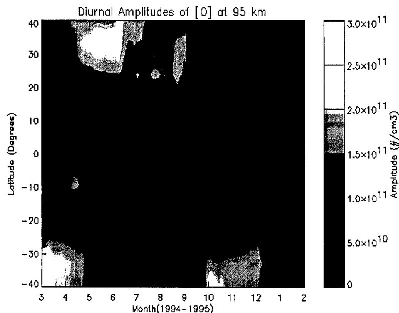
Plate 4. Latitude and time dependence of Diurnal Tidal [O(^3P)] amplitudes ( \text{cm}^{-3} )
