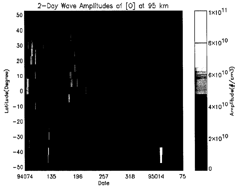
Plate 1: Latitude and time dependence of 2-Day wave amplitudes
