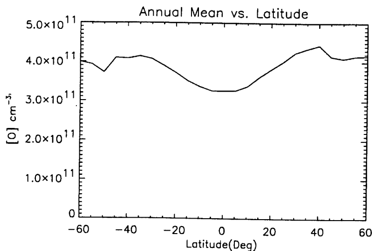
Figure 2. Annual Mean vs. Latitude
