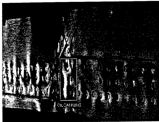
Figure 18 DAIS Results for Fuselage/Empennage Bulkhead
