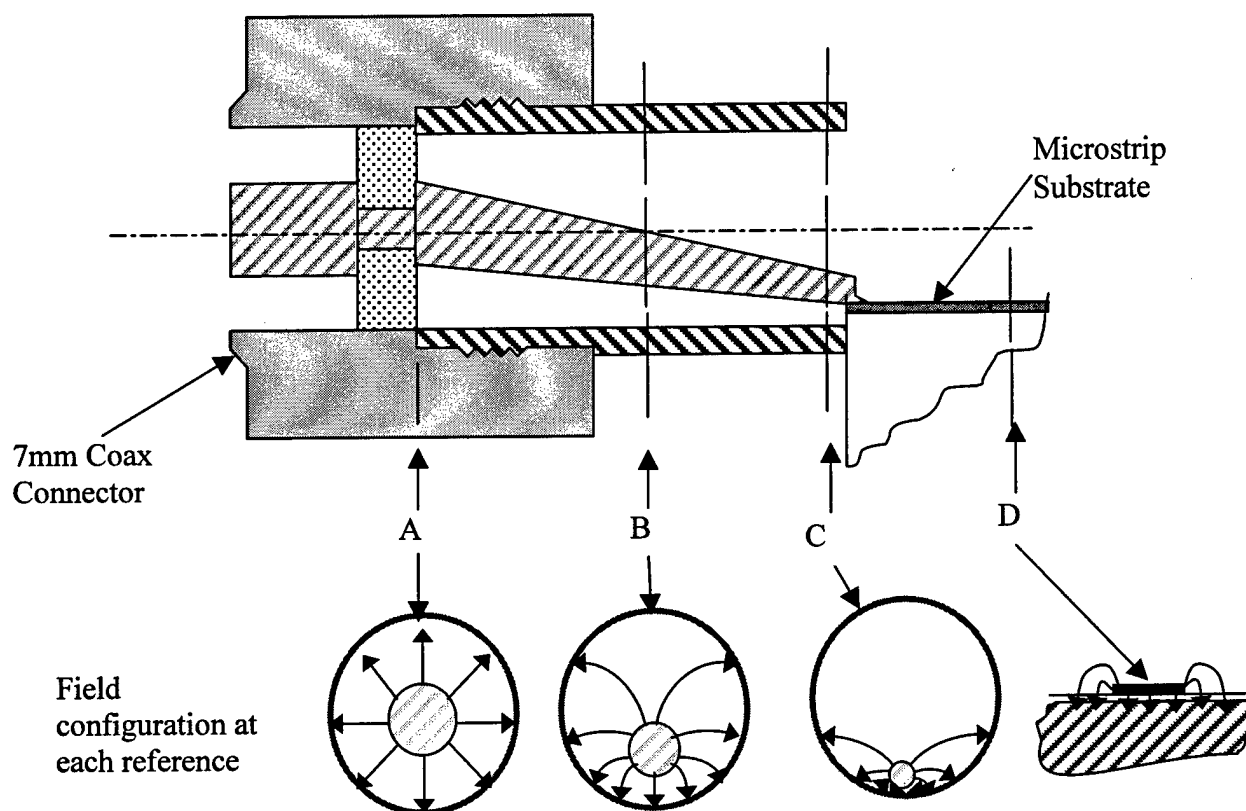
Figure 15. Cross section of Eisenhart connector
