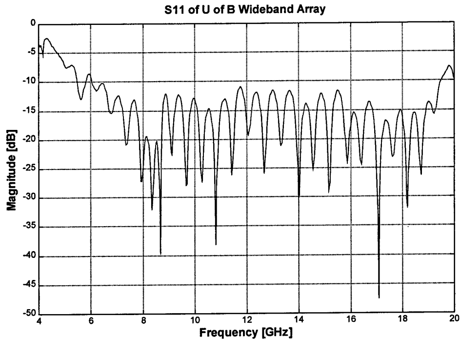
Figure 30. S11 of the U of B wideband array
