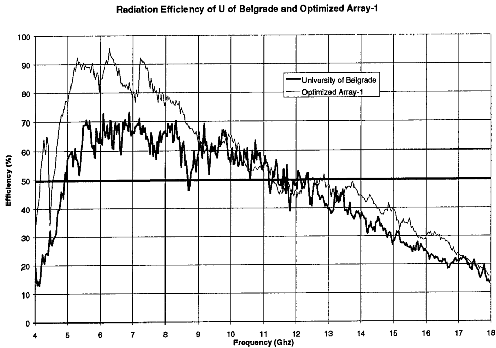
Figure 48. Radiation efficiency of U of B and Optimized Array-1 designs
