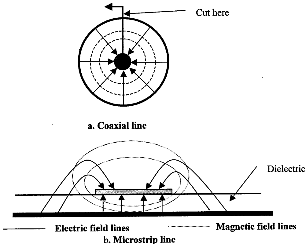
Figure 12. Evolution of microstrip line from coaxial line by unfolding
