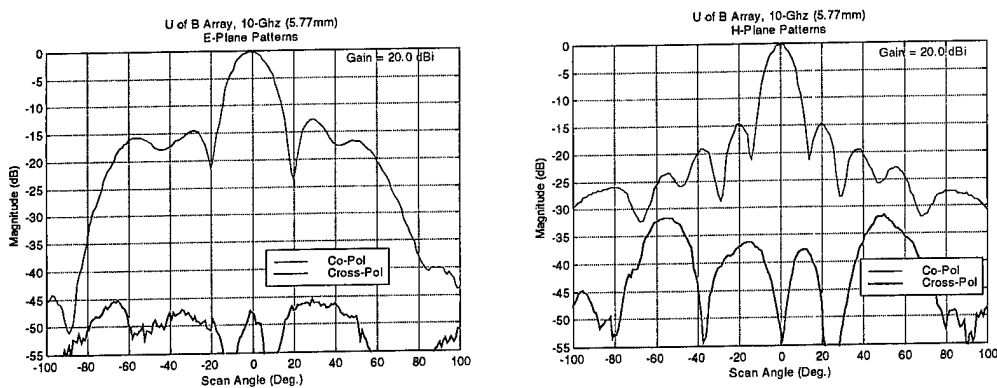
Figure 32. Representative U of B wideband array (10 GHz) E and H-plane patterns
