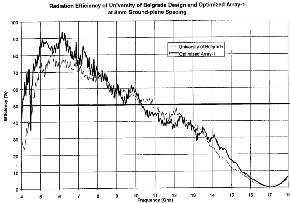
Figure 58. Radiation efficiency of the U of B and Optimized Array-1 at 8mm height
