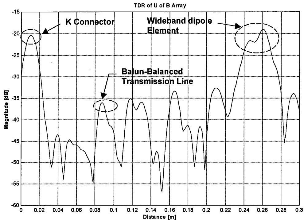
Figure 31. TDR of U of B wideband printed-dipole array
