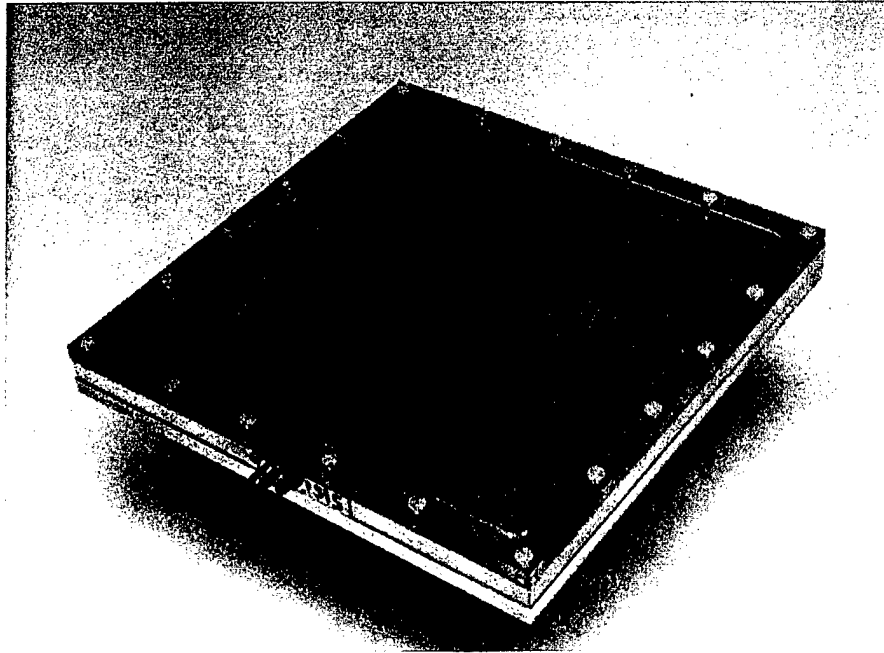
Figure 23. Photo of wideband printed-dipole array
