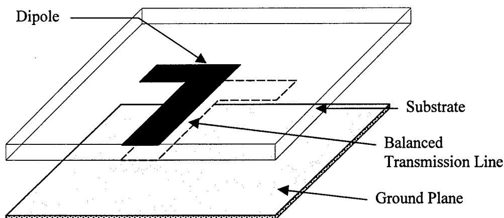
Figure 11. Printed-dipole element
