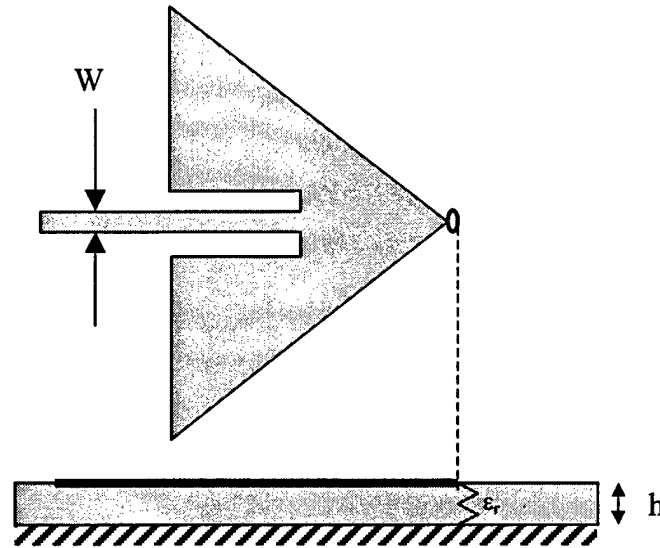
Figure 8. Triangular microstrip antenna with chip resistor loading
