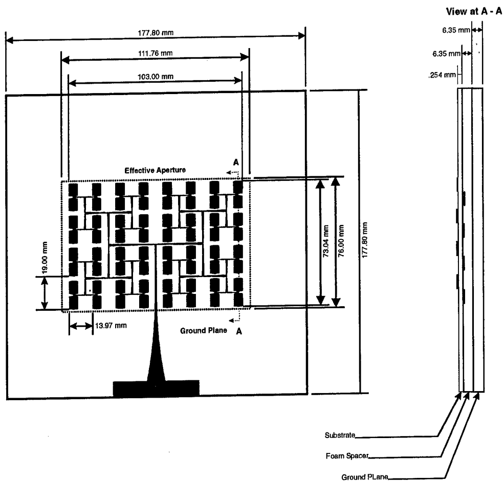
Figure 43. Optimized Array-1 (6.35mm) physical layout
