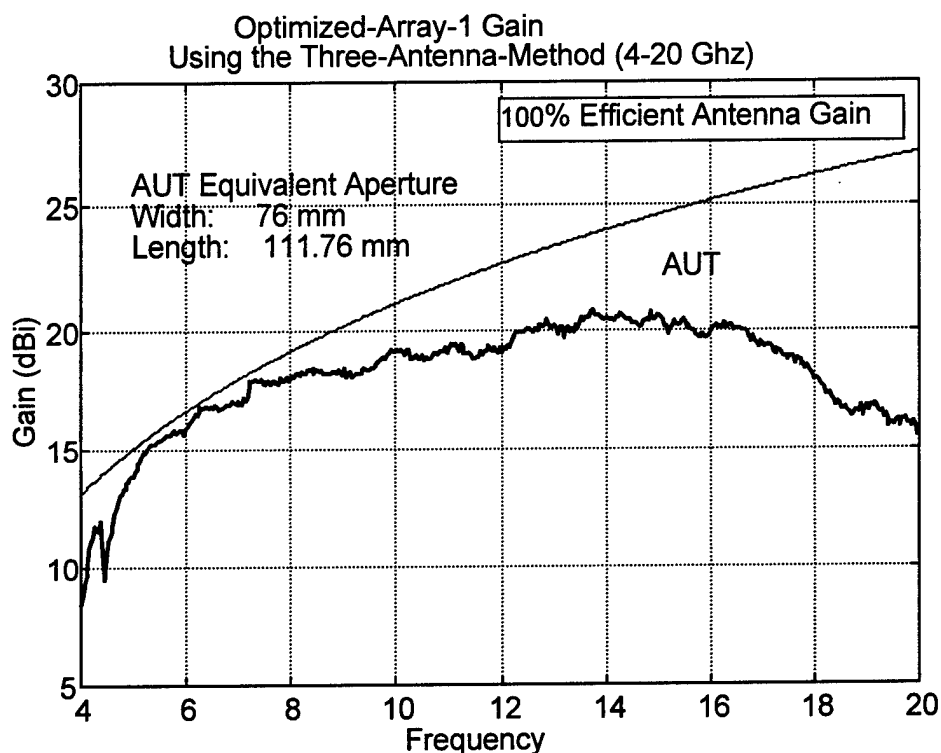
Figure 47. Optimized Array-1 gain using the 3 antenna method
