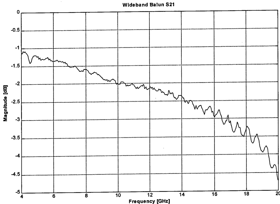
Figure 27. Double balun S_{21}
