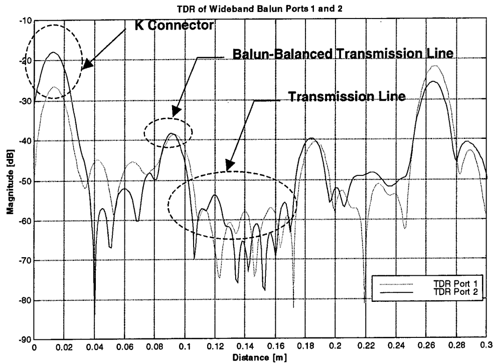
Figure 28. Double balun TDR of Ports 1 and 2
