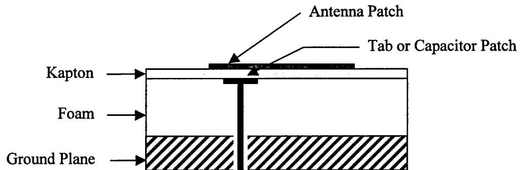
Figure 2. Implementation of series capacitance to compensate for probe inductance
