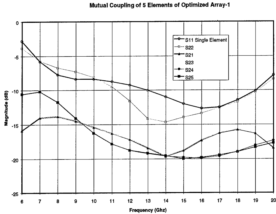
Figure 42. Mutual coupling of 5 elements of Optimized Array-1(6.35mm)
