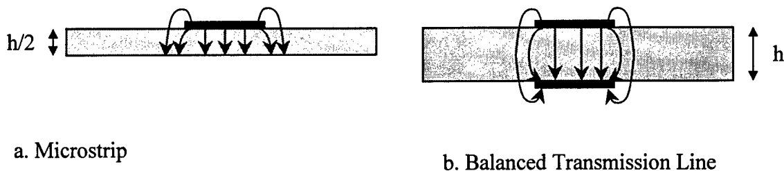
Figure 20. Field patterns of microstrip and balanced transmission line
