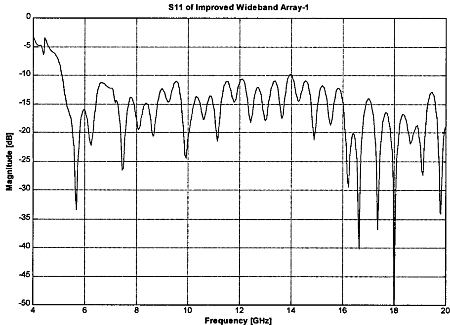
Figure 44. S11 of Optimized Array-1
