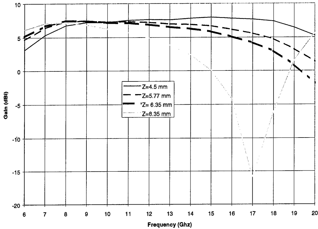
Gain vs Frequency for Various Heights Over Ground
