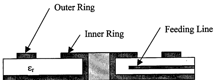
Figure 5. Double Shorted Annular Patch
