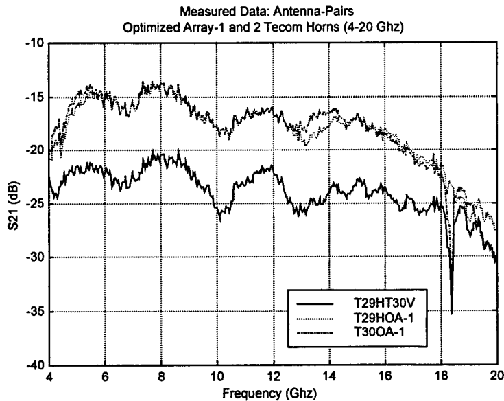
Figure 46. S_{21} measurements for three-antennas
