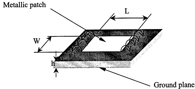
Figure 21. Microstrip patch antenna
