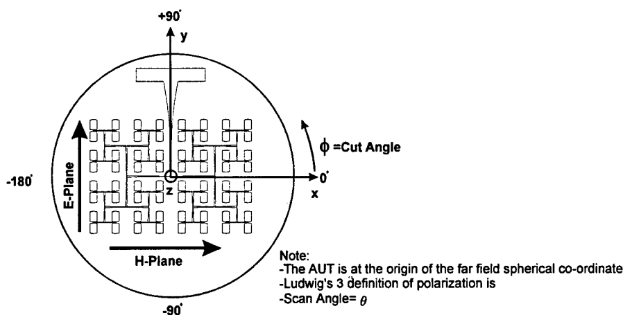
Figure 35. Relationship between the AUT and the spherical coordinate system
