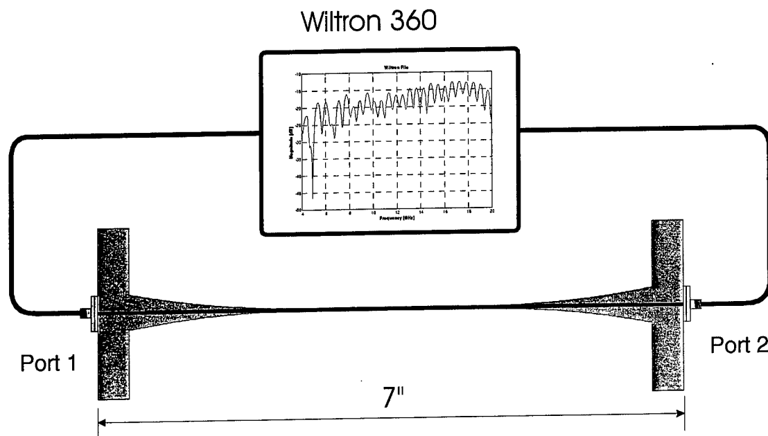
Figure 24. Balun test setup
