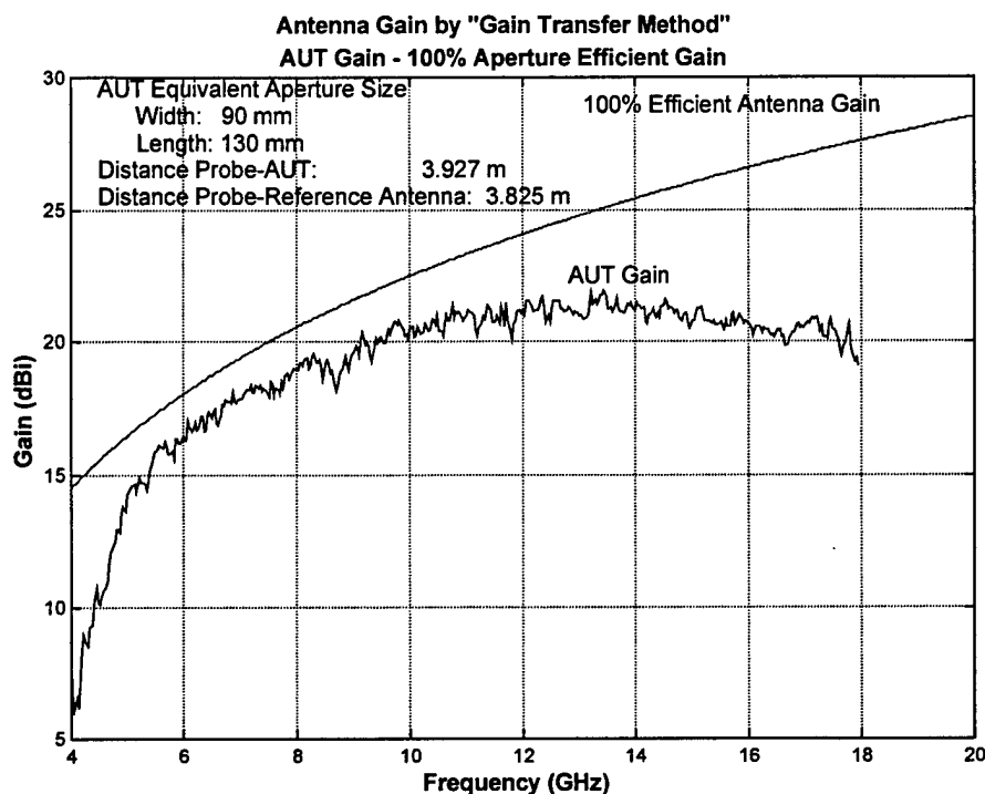
Figure 37. U of B Array(5.77mm) measured and theoretical gain
