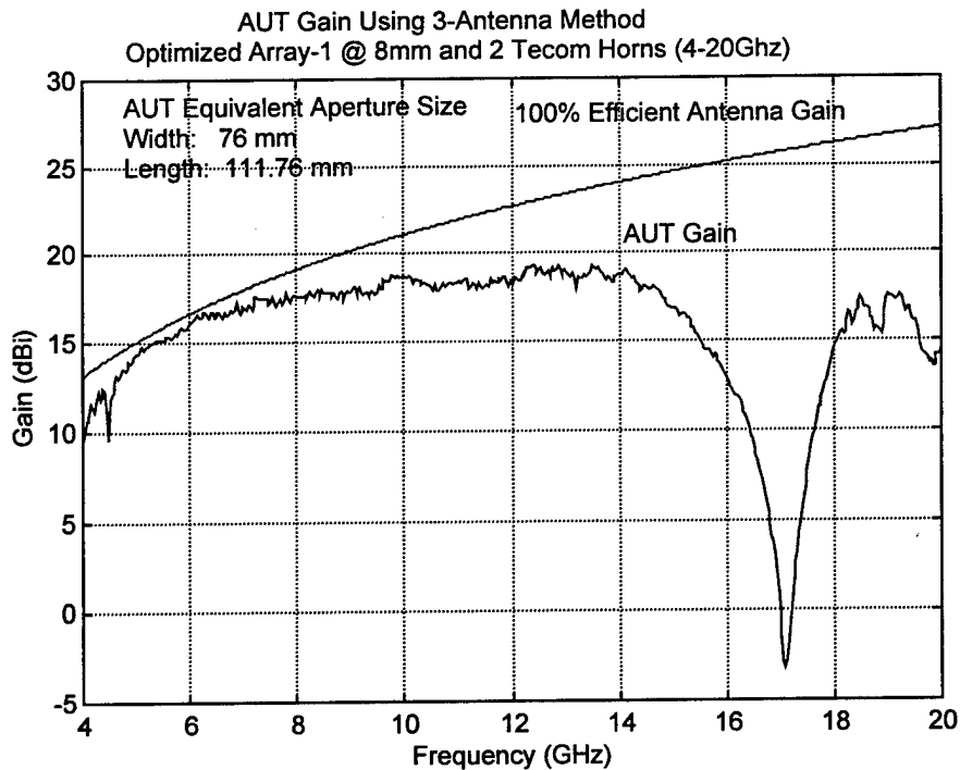
Figure 57. Optimized Array-1 gain at 8mm ground-plane spacing
