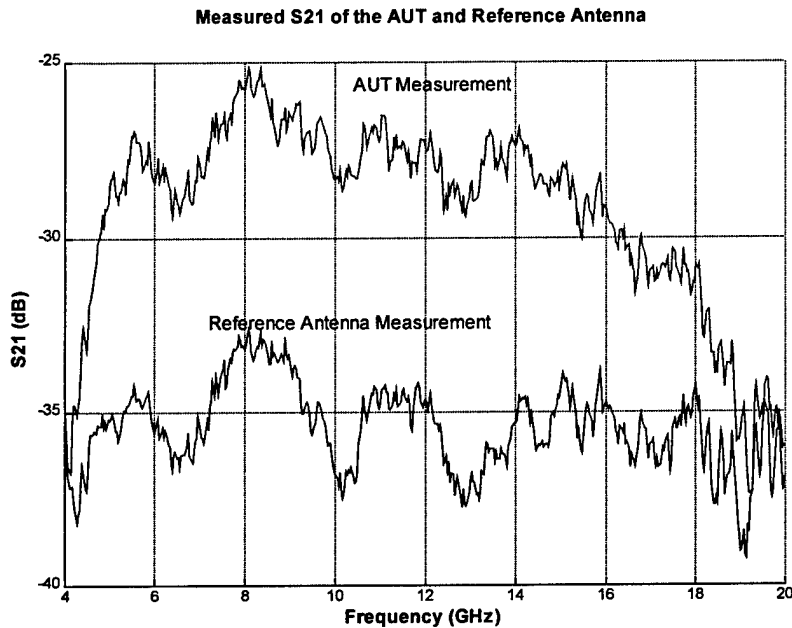
Figure 36. S_{21} of AUT and reference antenna
