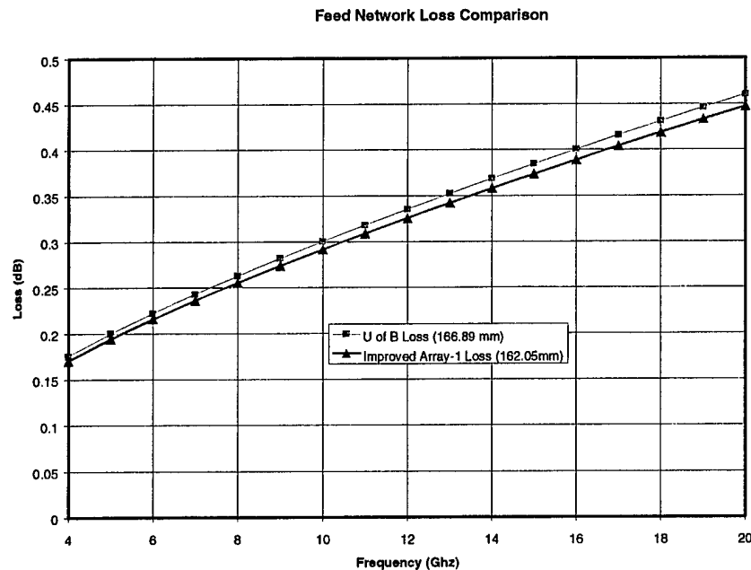
Figure 50. Comparison of feed network losses
