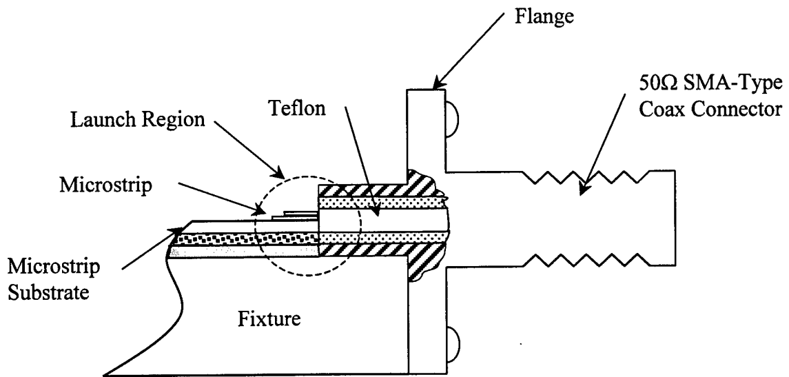
Figure 13. Typical Coaxial to microstrip transition
