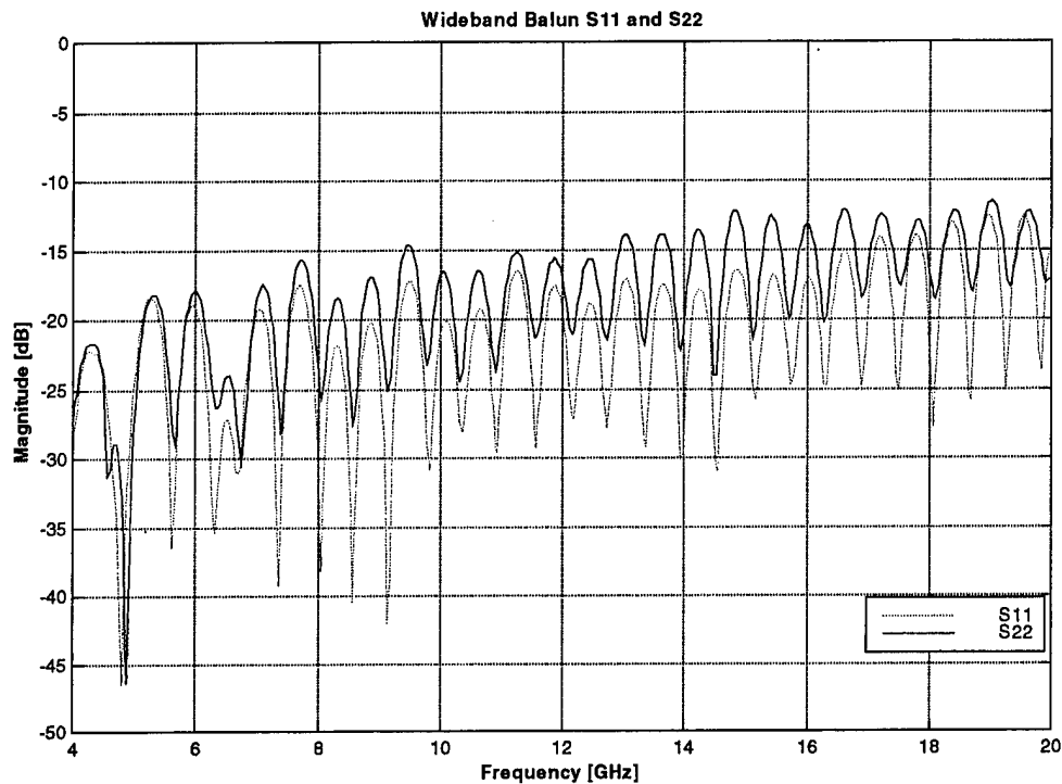
Figure 26. Double balun S_{11} and S_{22}
