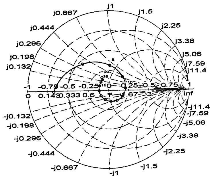
Figure 51. Smith chart of Original U of B wideband dipole element
