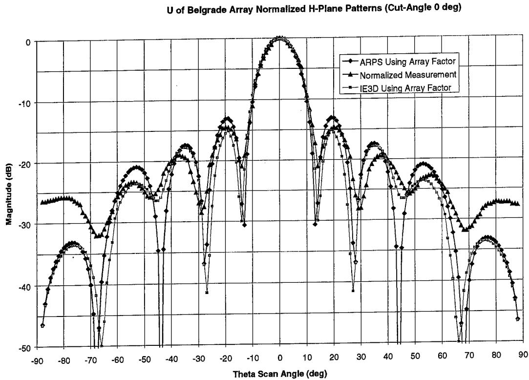
Figure 34. Comparison of simulated ( ARPS TM / IE3D TM ) vs. measured radiation pattern
