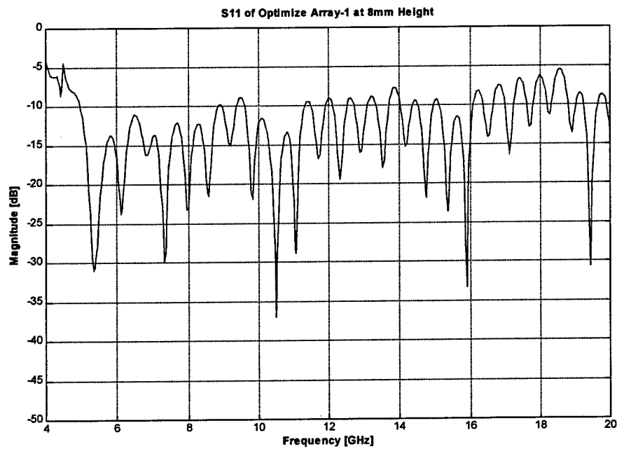
Figure 55. S11 of Optimized Array-1 at 8mm ground-plane spacing
