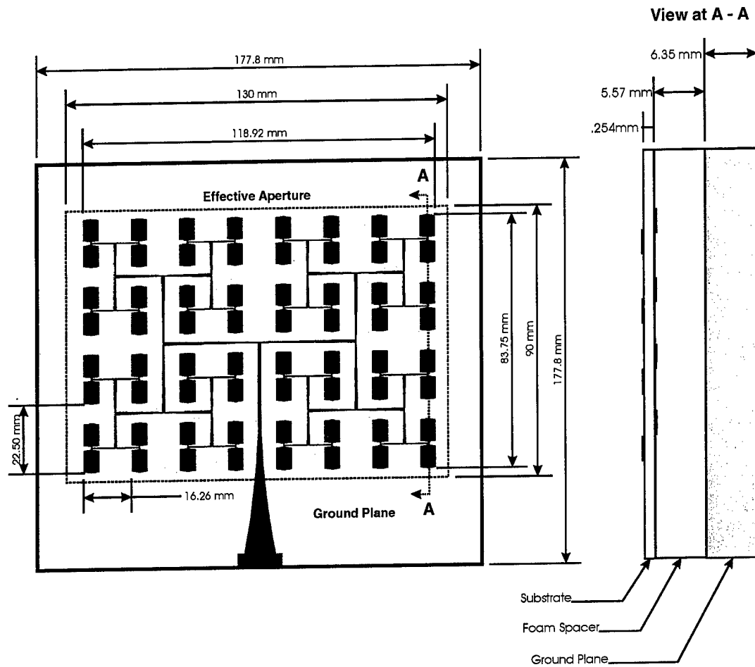
Figure 22. University of Belgrade wideband printed-dipole array
