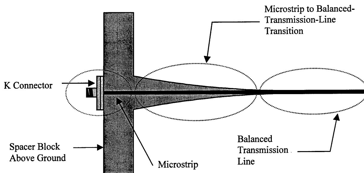
Figure 19. Wideband balun (top-view)
