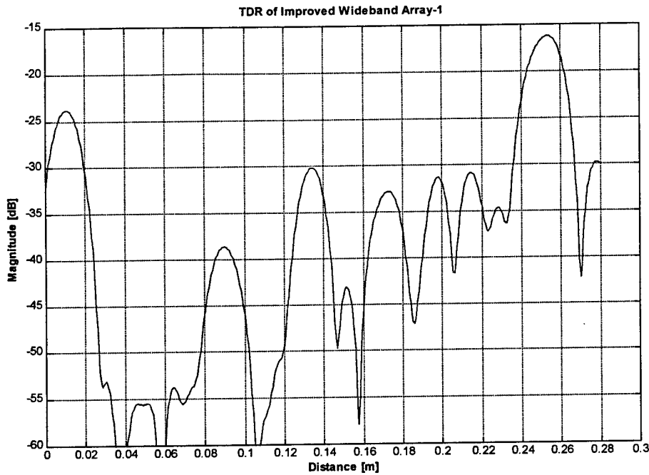
Figure 45. TDR of Optimized Array-1
