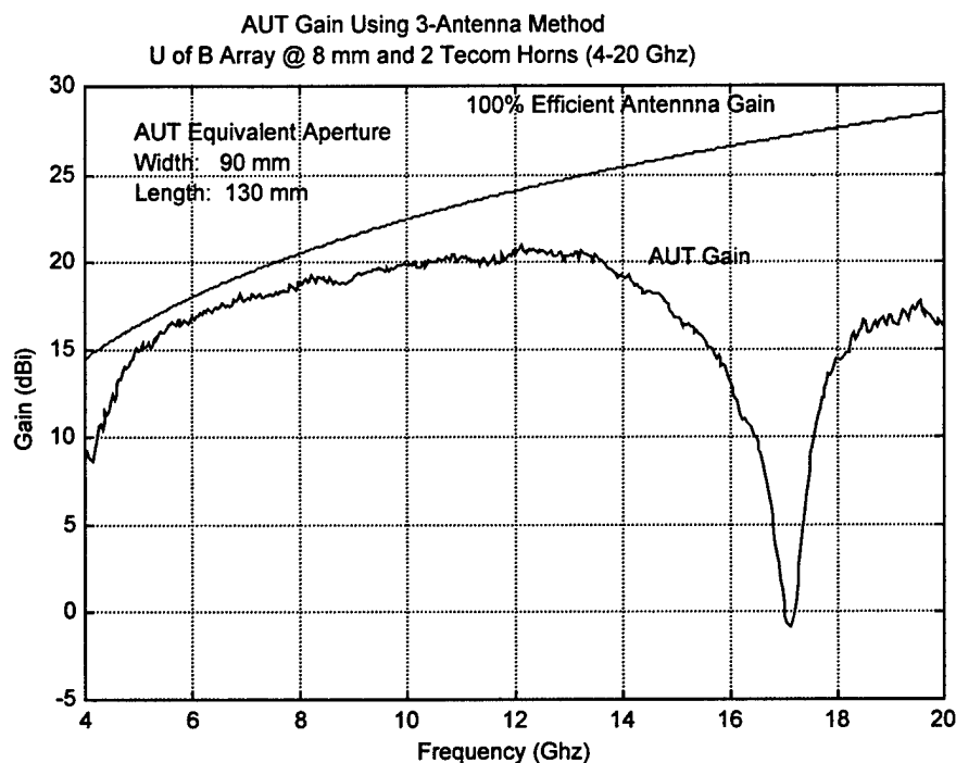
Figure 56. U of B Array gain at 8mm ground-plane spacing
