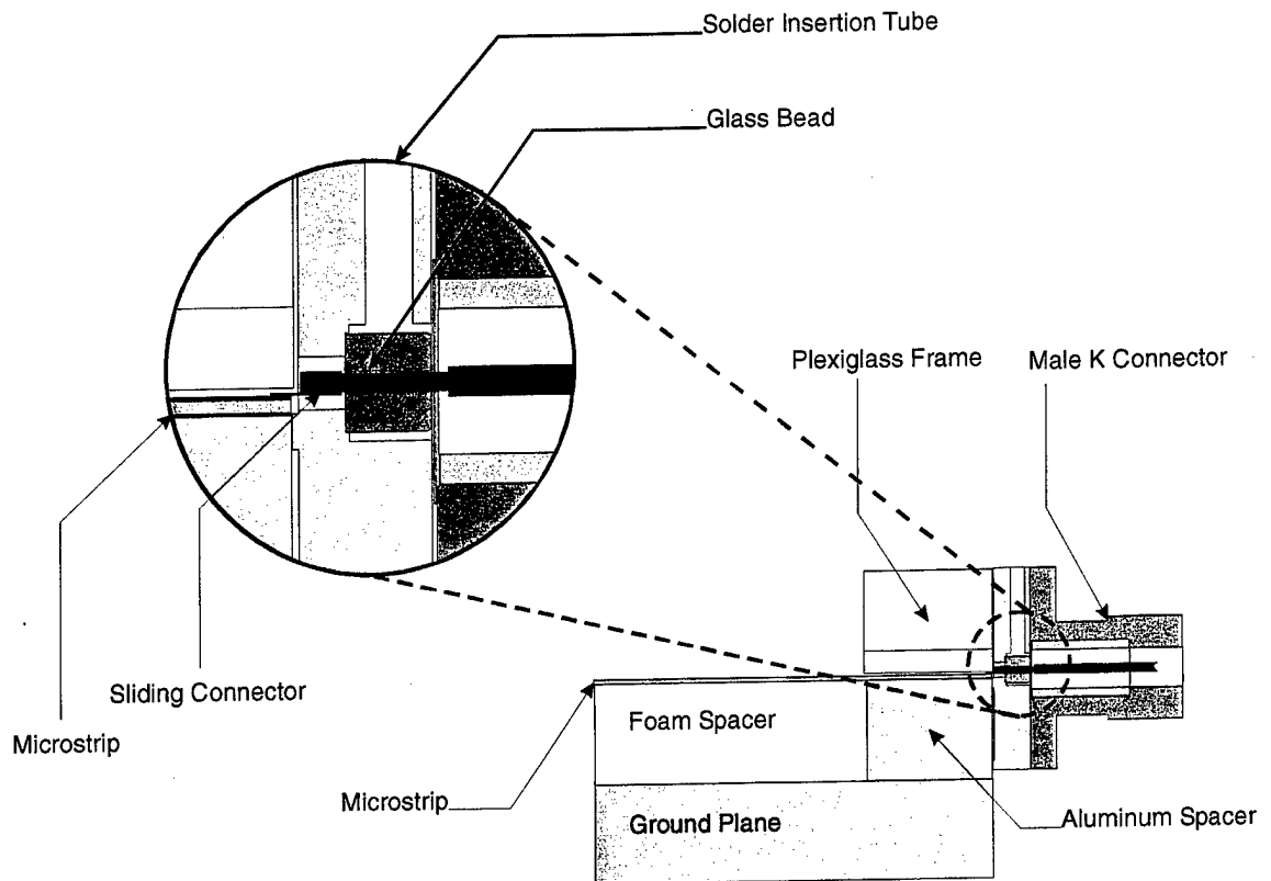
Figure 17. K Connector™ to printed antenna interface (side-view)
