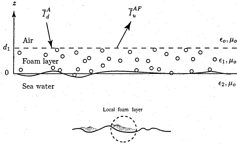
Figure 2: The configuration of local foam layer on wind-driven rough ocean surface.
