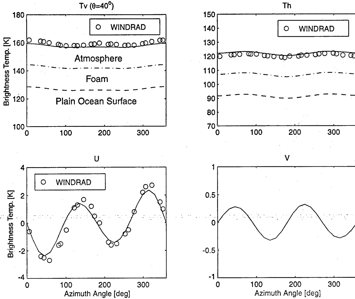
Figure 14: The brightness temperature of wind-driven ocean surface for nadir looking angle \theta = 40^\circ and the lower cutoff wavenumber k_d = 120 \text{ m}^{-1} .
