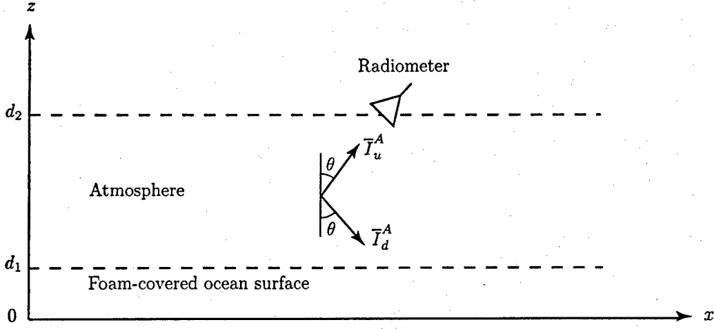
Figure 3: The atmospheric layer above a foam-covered ocean surface.
