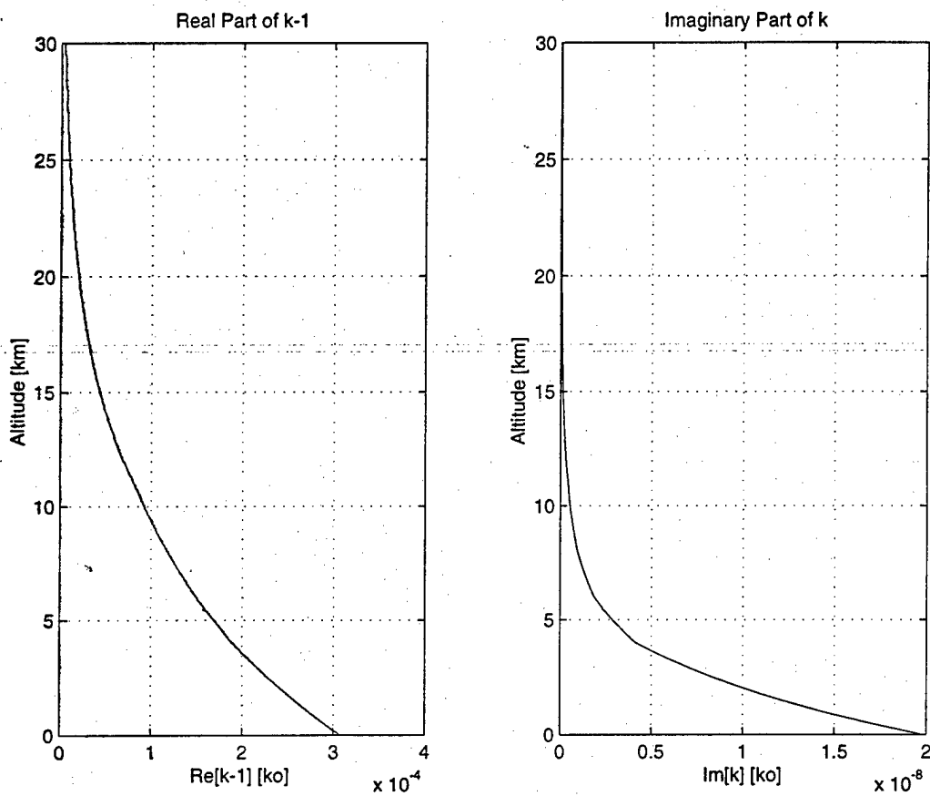
Figure 5: The complex wavenumber of electromagnetic wave with f = 19.35 GHz propagating in the atmosphere in terms of the wavenumber in free space.
