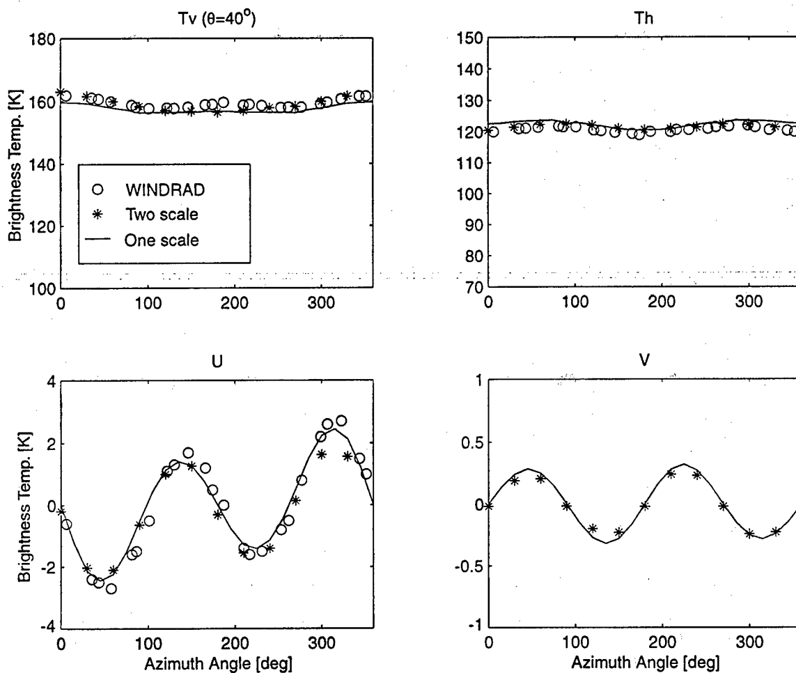
Figure 16: The comparison of the one-scale and two-scale models at \theta = 40^\circ .
