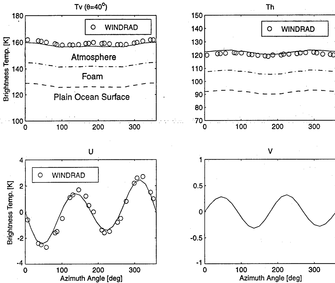
Figure 12: The brightness temperature of wind-driven ocean surface for nadir looking angle \theta = 40^\circ and the lower cutoff wavenumber k_d = 80 \text{ m}^{-1} .
