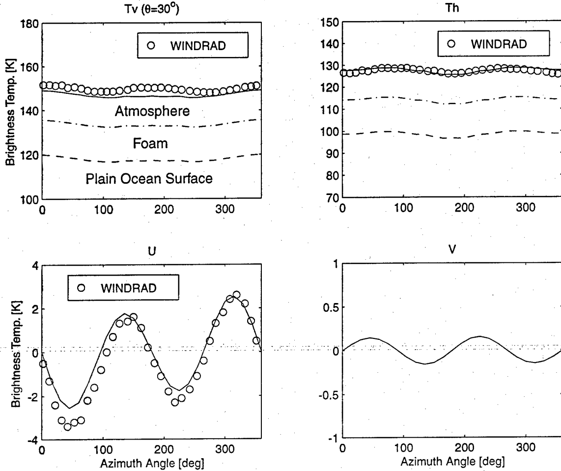
Figure 11: The brightness temperature of wind-driven ocean surface for nadir looking angle \theta = 30^\circ and the lower cutoff wavenumber k_d = 80 \text{ m}^{-1} .
