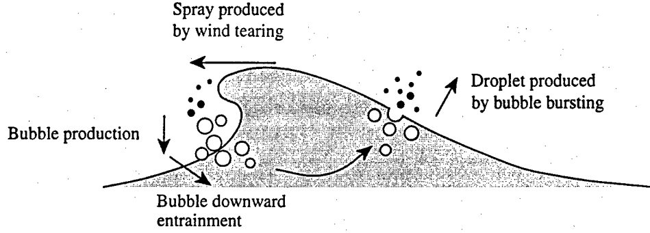
Figure 1: The generation of sea-foam.
