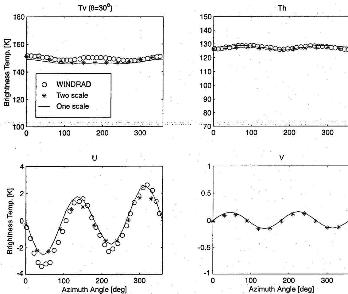
Figure 15: The comparison of the one-scale and two-scale models at \theta = 30^\circ .
