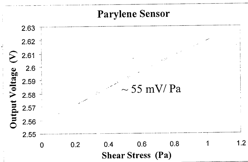
Figure 7: Windtunnel Test Result
