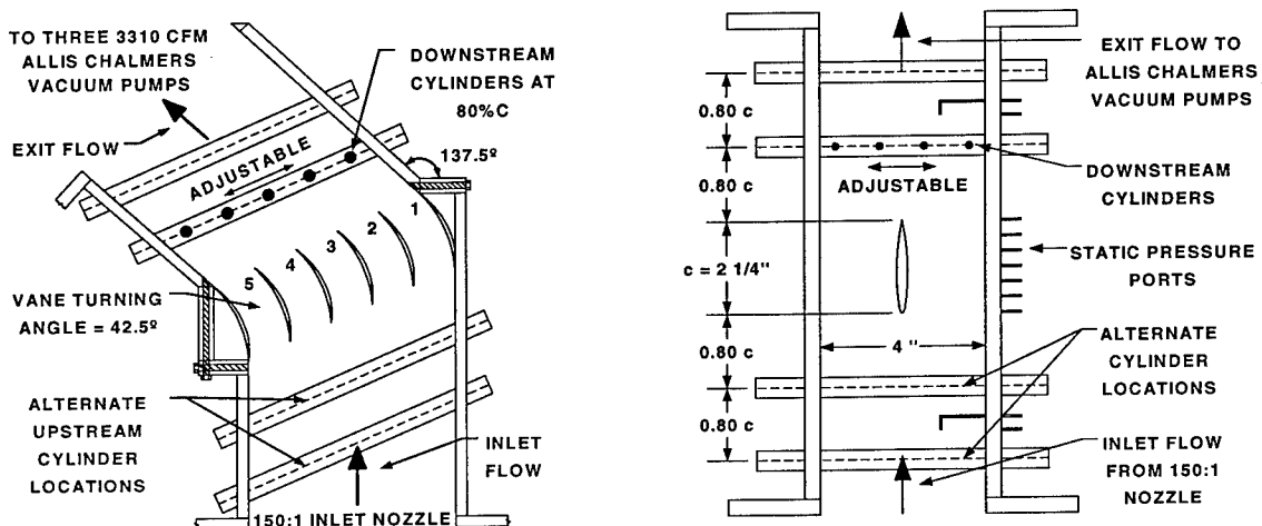
Figure 1. Top views of S&T Notre Dame cascade (left) and new, modified unloaded cascade (right).
