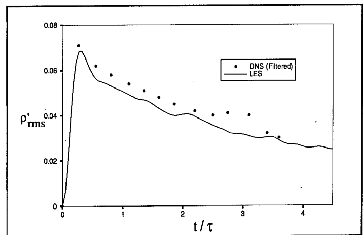
Fig.7 Time evolution of rms density fluctuation. Time has been non-dimensionalized by eddy turn over time. Mt=0.4 , Re_\lambda = 55 . The filtered DNS data is taken from Syropoulos and Blaisdell, 1996.
