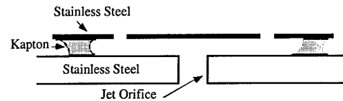
Figure 1. Schematic cross-section of robust microjet modulator
