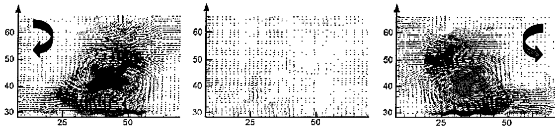
Figure 10: Vectored synthetic jets in a cross-flow
