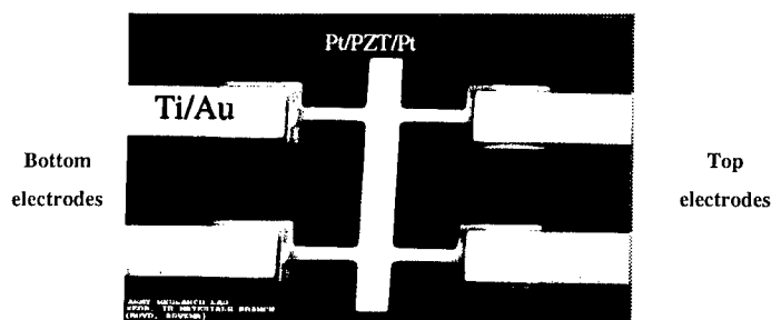
Figure 6. SEM of partly processed Pt/PZT/Pt xylophone structure
