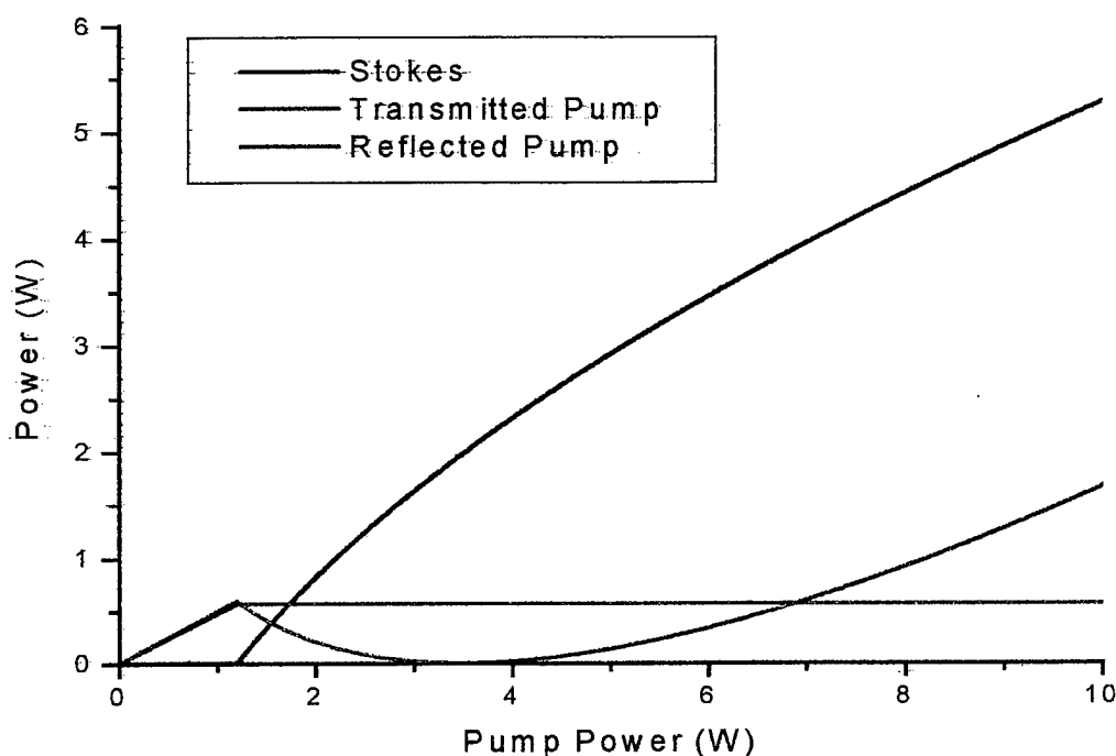
Figure 6. Theoretical results of the reflected pump, transmitted pump, ( 1.064 \mu m ) and Stokes ( 1.54 \mu m ) power as a function of input pump power from a methane cw Raman laser. The cw Raman laser has a cavity length of 5 \text{ cm} and mirror reflectivities of: R_F=.997 R_B=.9995 for the front and back mirrors at the pump wavelength and: R_F=.9995 R_B=.997 for the front and back mirrors at the Stokes wavelength. The absorption loss for all mirrors is A=15 \text{ ppm} .
