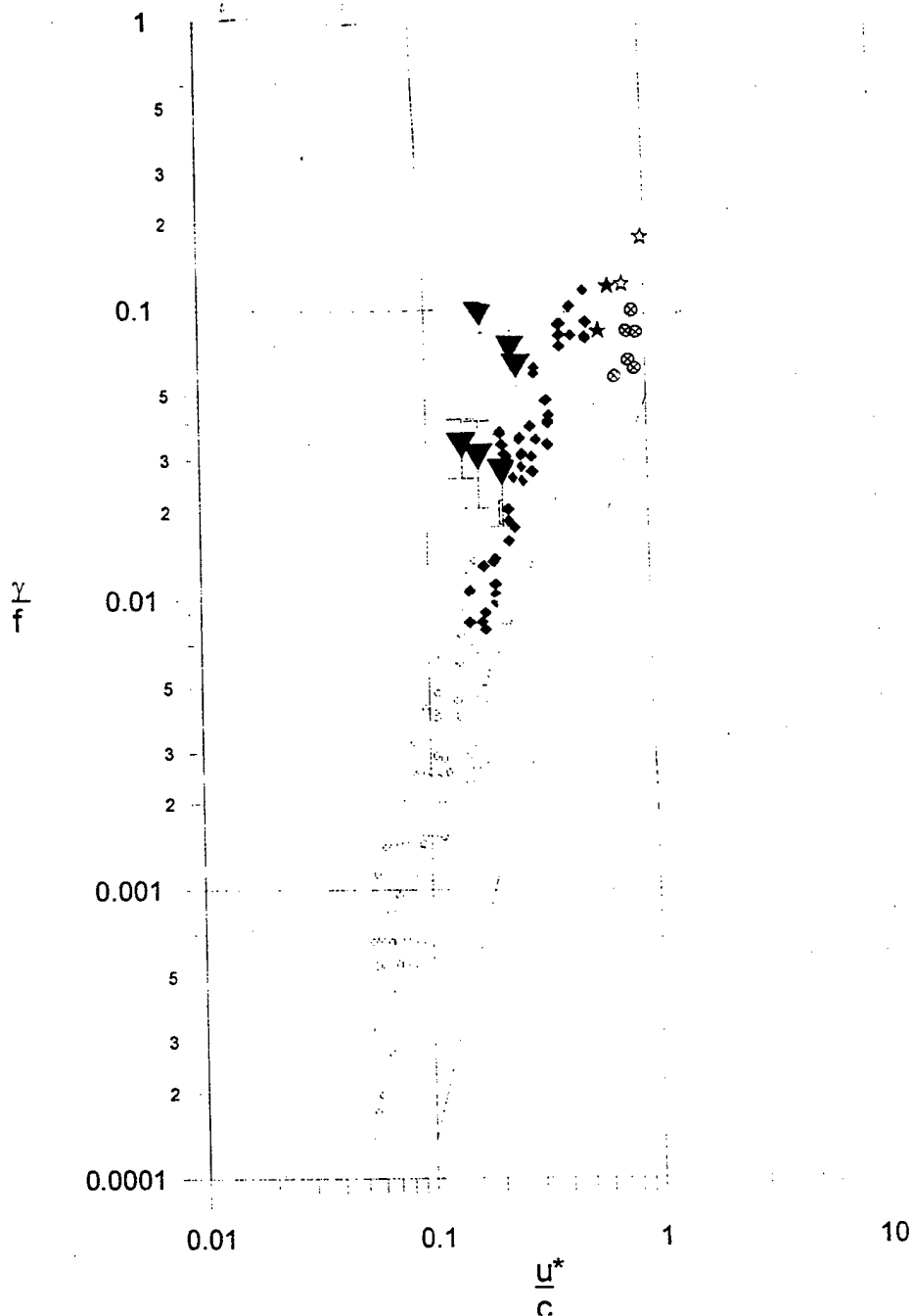
Growth rates from Snyder et al. (1981), open circles; Shemdin and Hsu (1967), open triangles; Mitsuyasu and Honda, (1982), solid diamonds; Banner (1990), stars; Mastenbroek et al. (1995), crossed square; and Banner and Peirson (1998), crossed circles. Estimated dissipation rates from Young and Sobey (1986) ak=0.16 , solid line; Harris et al. (1995), dotted line; Cohen (1997), dashed line. The measured dissipation rates in this study are shown as solid triangles.
