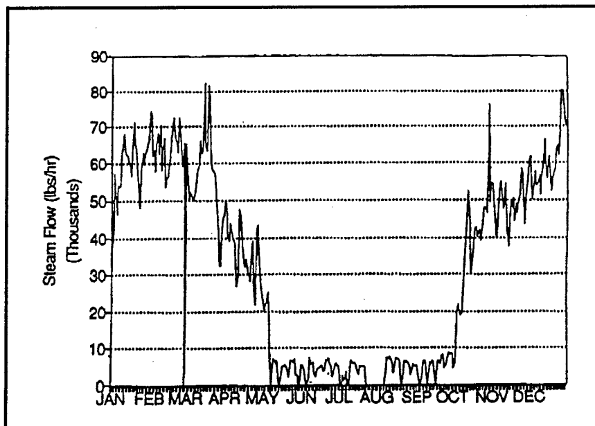
Figure 11. Steam load profile (klb/hr ) for January – December 1993.
