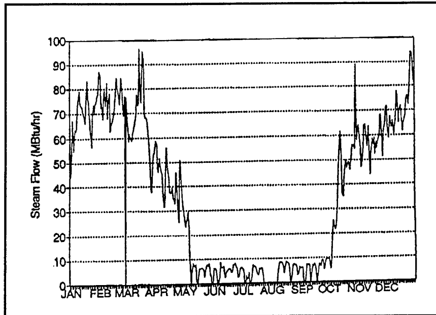
Figure 12. Steam load profile (MBtu/hr) for January – December 1993.
