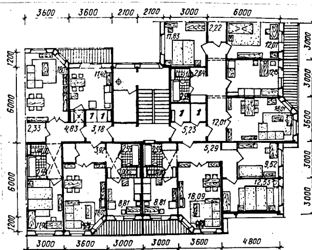
Figure 1. Plan for a corner block section for a Series 112 dwelling
