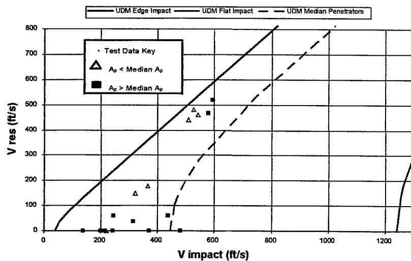
Figure B-12. Test Series 5 and 7, Impact and Residual Velocity Median Comparison
