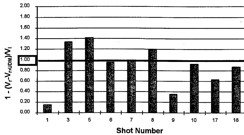
Figure B-5. Test Series 3, Prediction Accuracy
