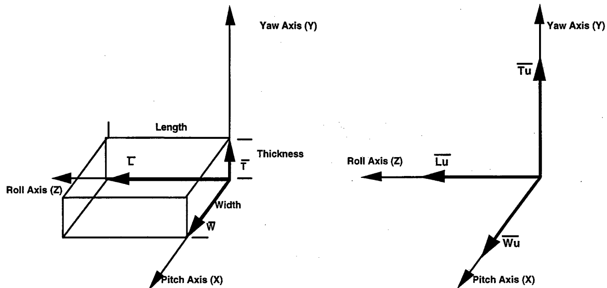
FIGURE 6. THREE-DIMENSIONAL FRAGMENT AND ORIENTATION UNIT VECTORS
