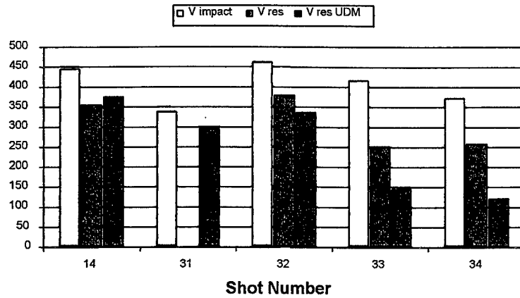
Figure B-1. Test Series 2, Impact and Residual Velocity Comparison
