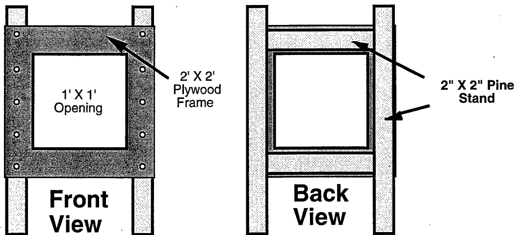
Figure 14: Residual Velocity Break Paper Stands
