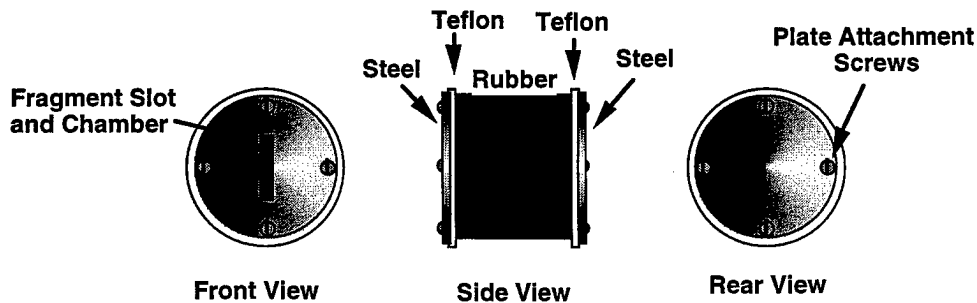
FIGURE 2. RUBBER SABOT
