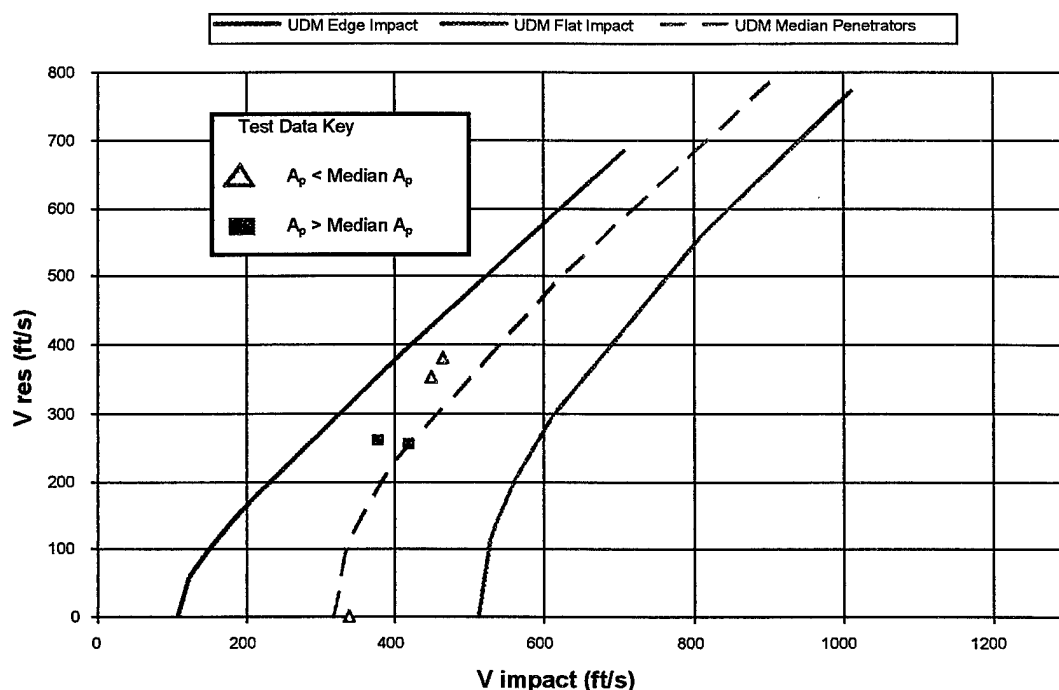
FIGURE 18. TEST SERIES 2, RESIDUAL VELOCITY CURVES ORIENTATION COMPARISON
