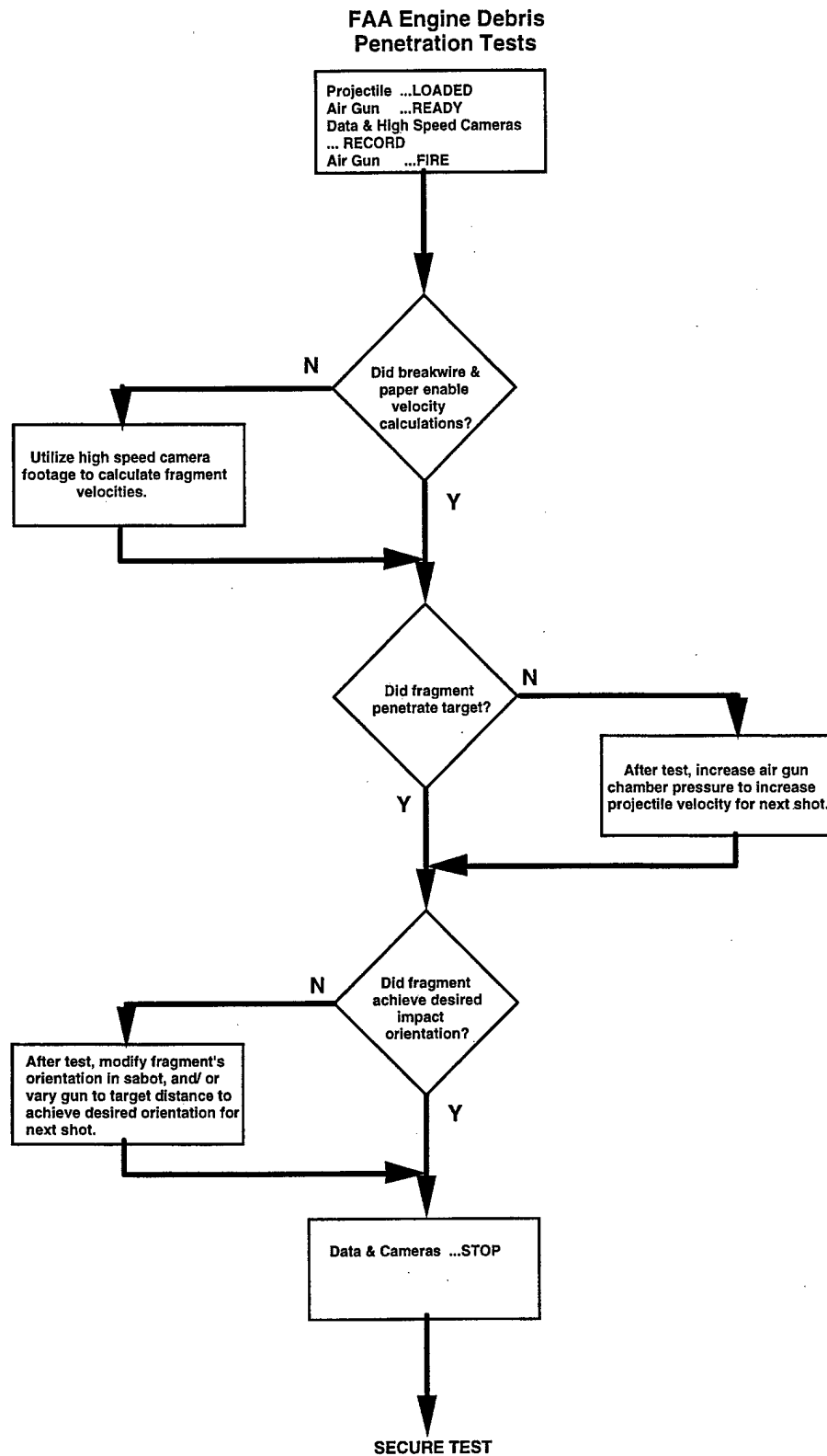
Figure 21: Test Logic Sequence
