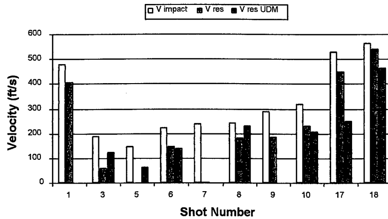
Figure B-4. Test Series 3, Impact and Residual Velocity Comparison
