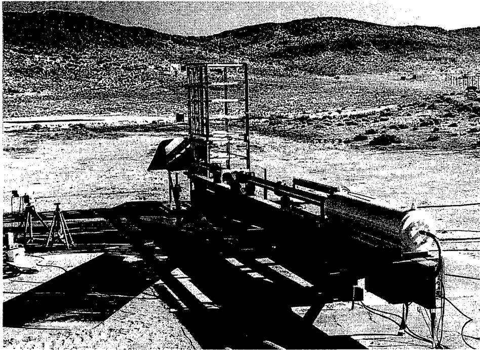
FIGURE 1. TEST SITE SETUP WITH MIKES GUN
