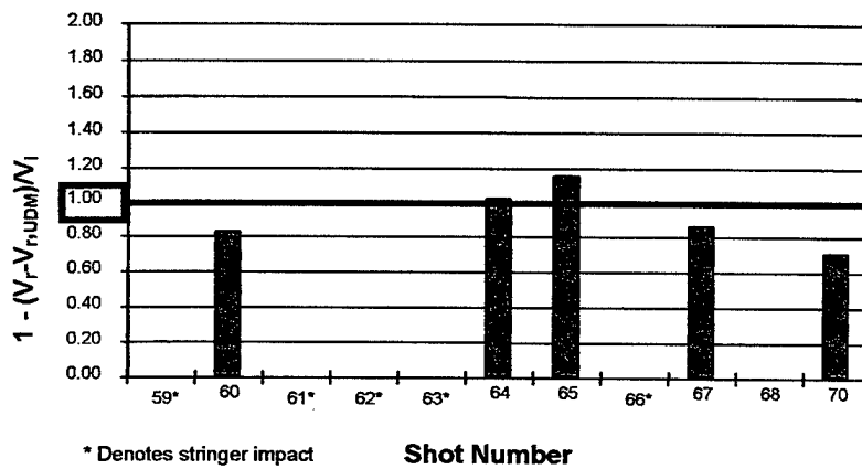
Figure B-17. Test Series 8, Prediction Accuracy
