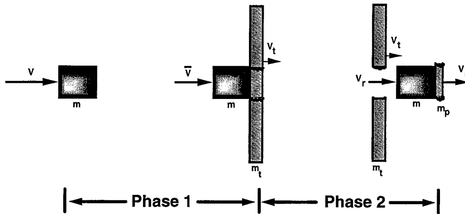
Figure A-1. Derivation of the Residual Velocity Equation
