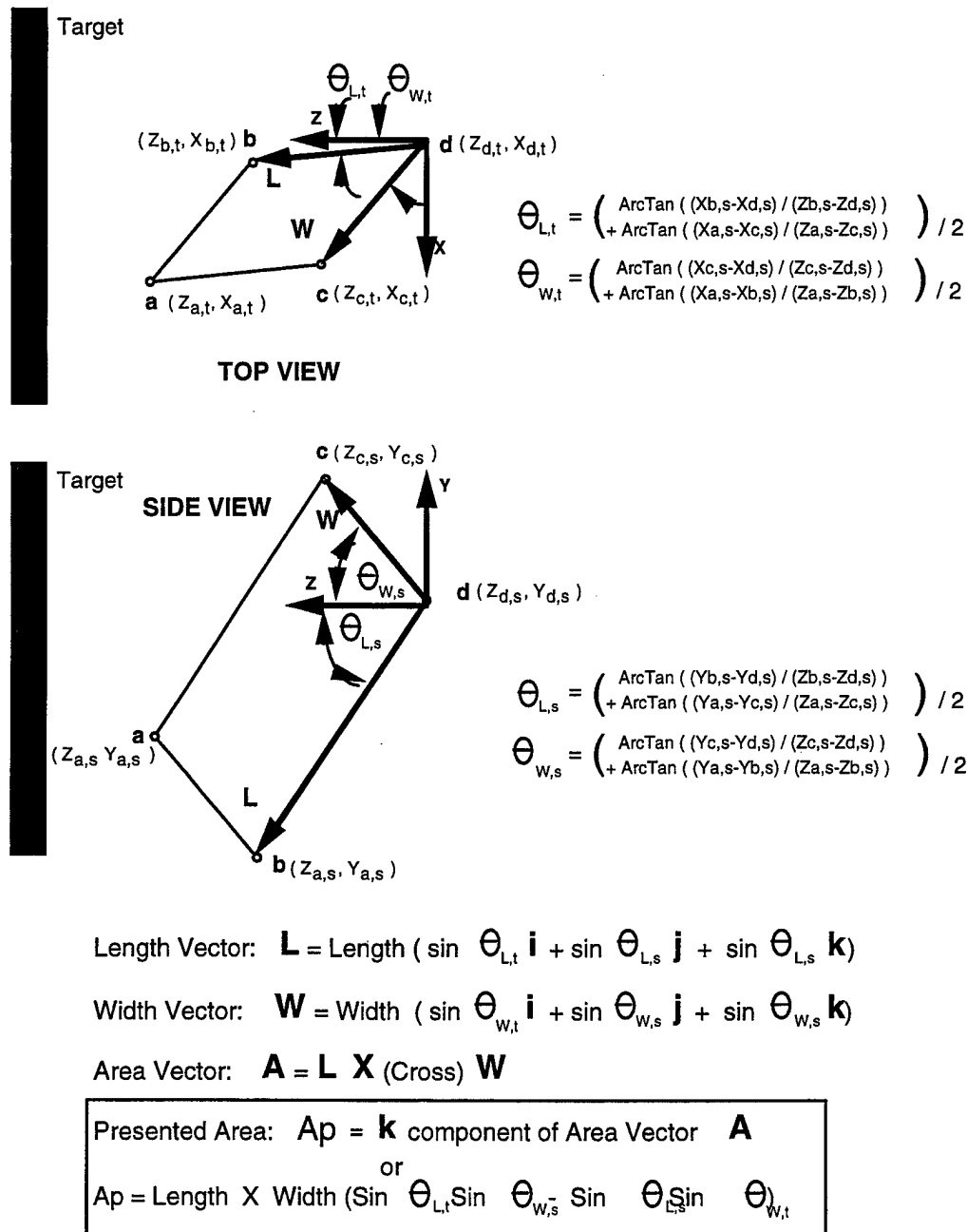
FIGURE 5. CALCULATION OF FRAGMENT PRESENTED AREA
