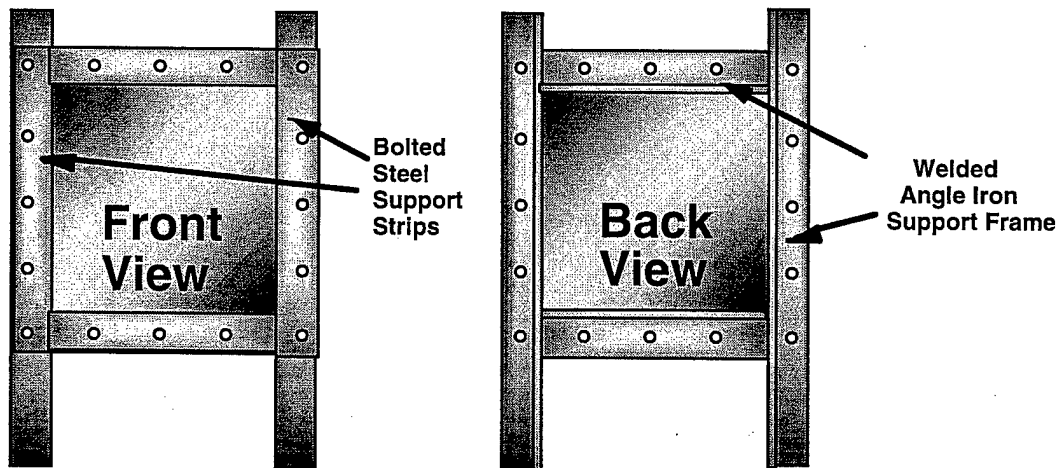
Figure 13: Plate Support Stand
