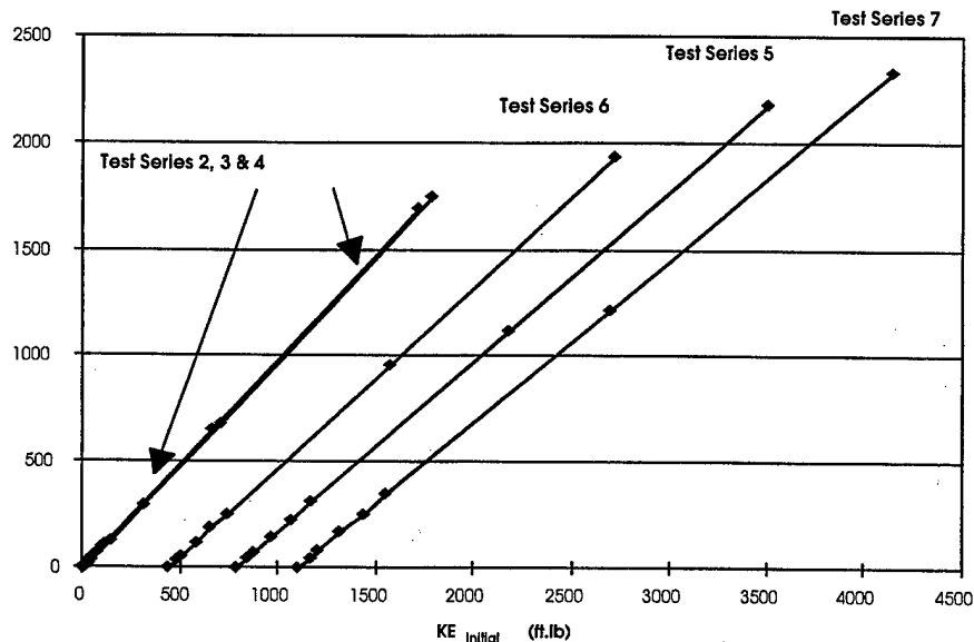
Figure 10: Pre-Test Prediction, Initial vs. Residual Kinetic Energy
