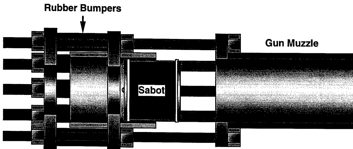
FIGURE 3. SABOT CATCHER
