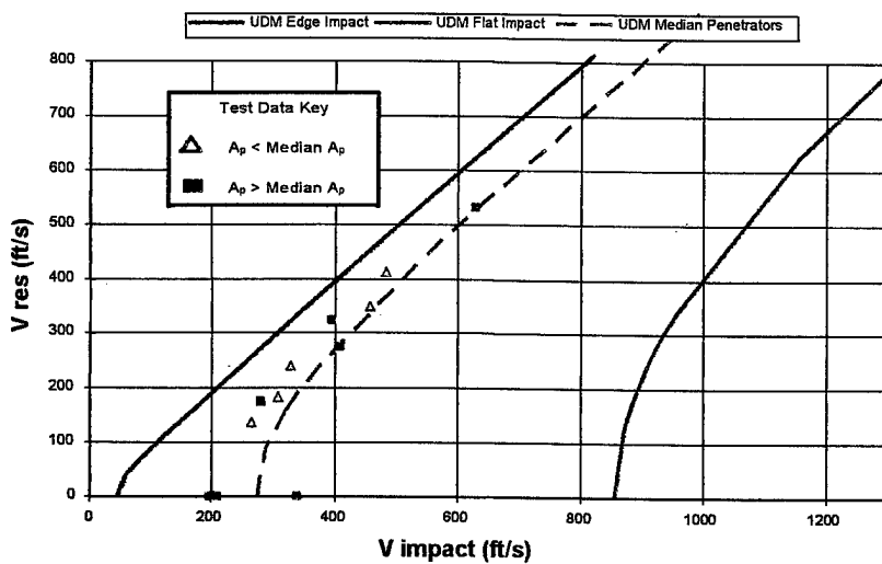
Figure B-9. Test Series 4, Impact and Residual Velocity Median Comparison
