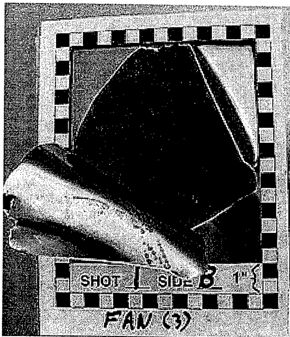
FIGURE 10. PETALING (SINGLE SIDED)
