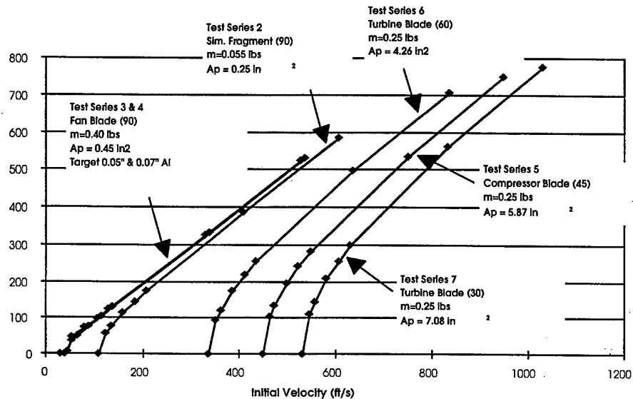
Figure 9: Pre-Test Predictions, Initial Impact vs. Residual Velocity
