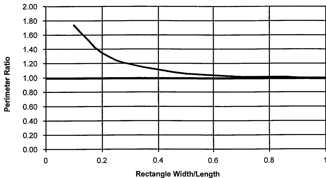
FIGURE 16. PERIMETER RATIO (RECTANGLE AND SQUARE OF EQUIVALENT PRESENTED AREA)
