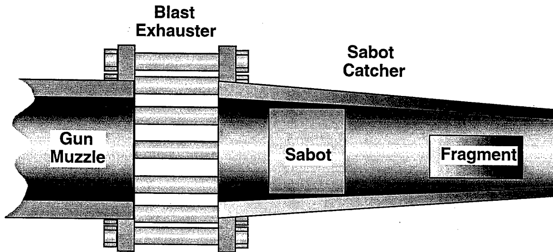
Figure 6: Sabot Catcher
