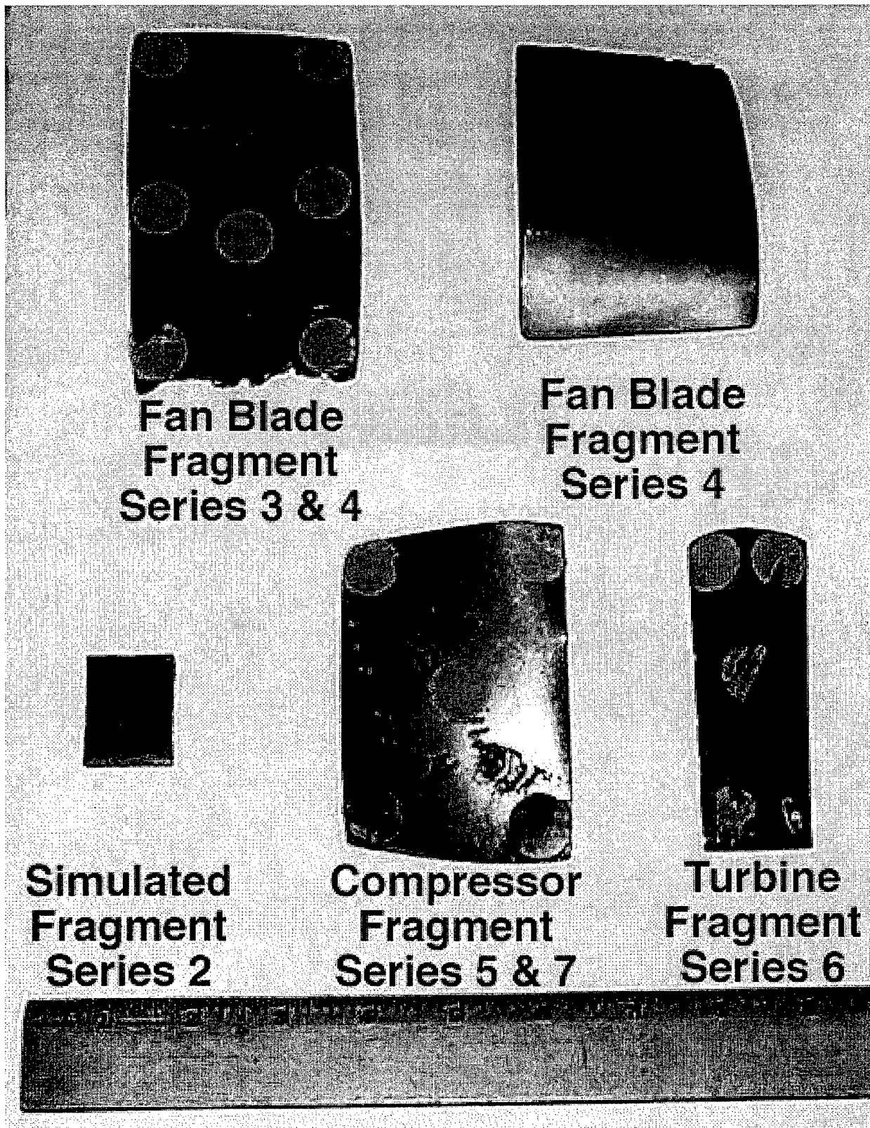
FIGURE 4. TEST SERIES FRAGMENT COMPARISON
