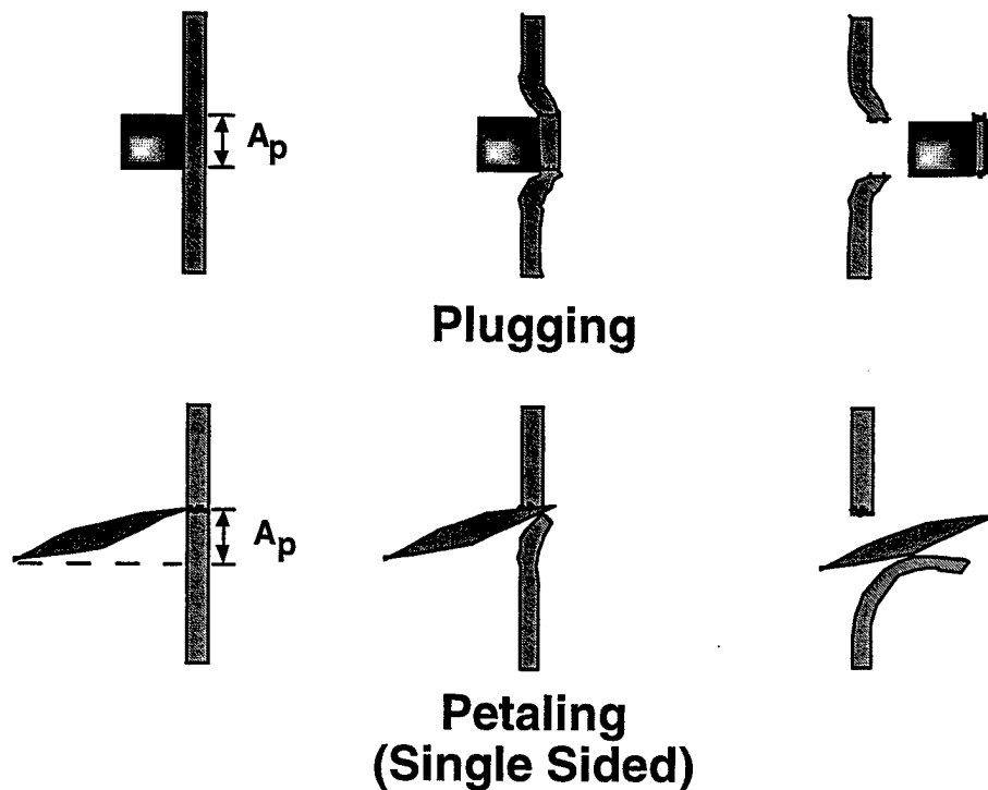
FIGURE 9. OBSERVED PERFORATION MODES
