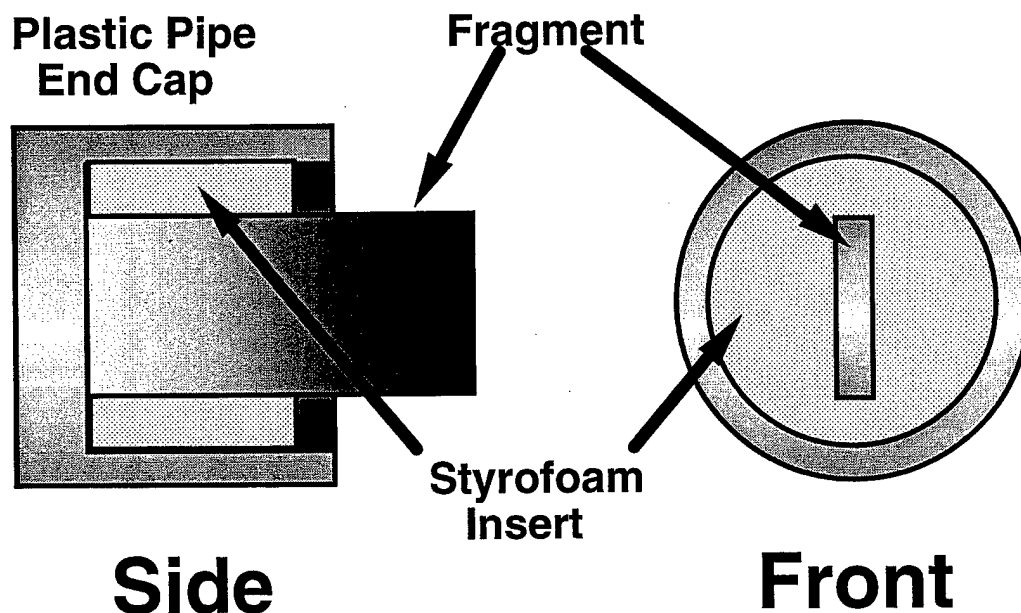
Figure 4: Saboted Fragment (90 deg. impact orientation)
