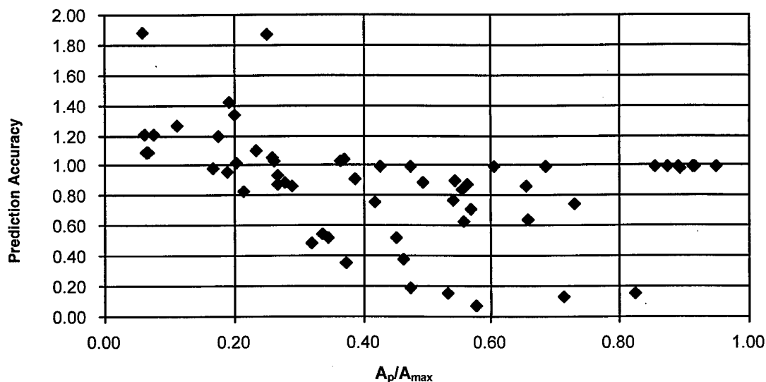
FIGURE 17. PREDICTION ACCURACY VERSUS AREA RATIO
