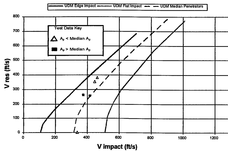
Figure B-3. Test Series 2, Impact and Residual Velocity Median Comparison
