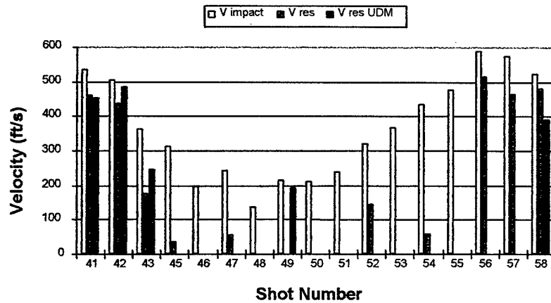
Figure B-10. Test Series 5 and 7, Impact and Residual Velocity Comparison
