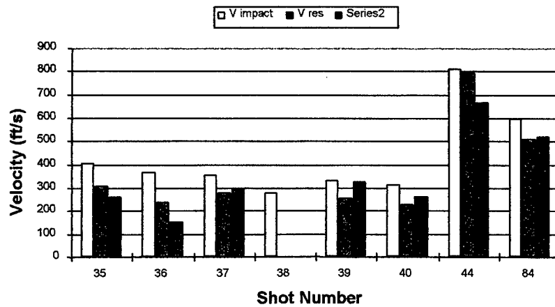
Figure B-13. Test Series 6, Impact and Residual Velocity Comparison
