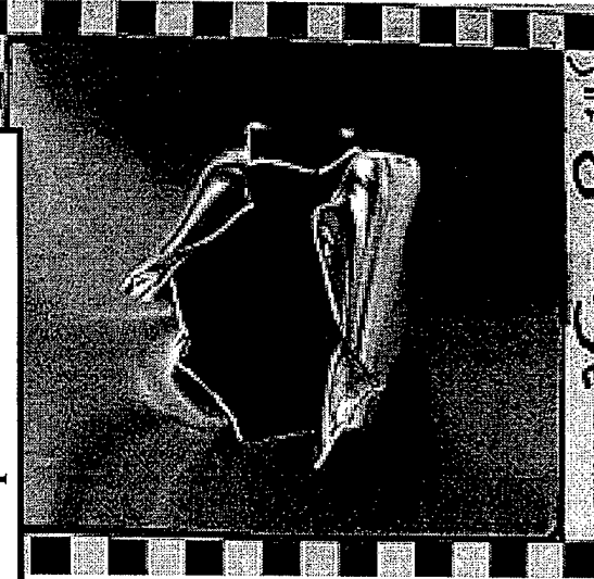
Figure C-133: Shot 35 Pre-Impact Orientation
