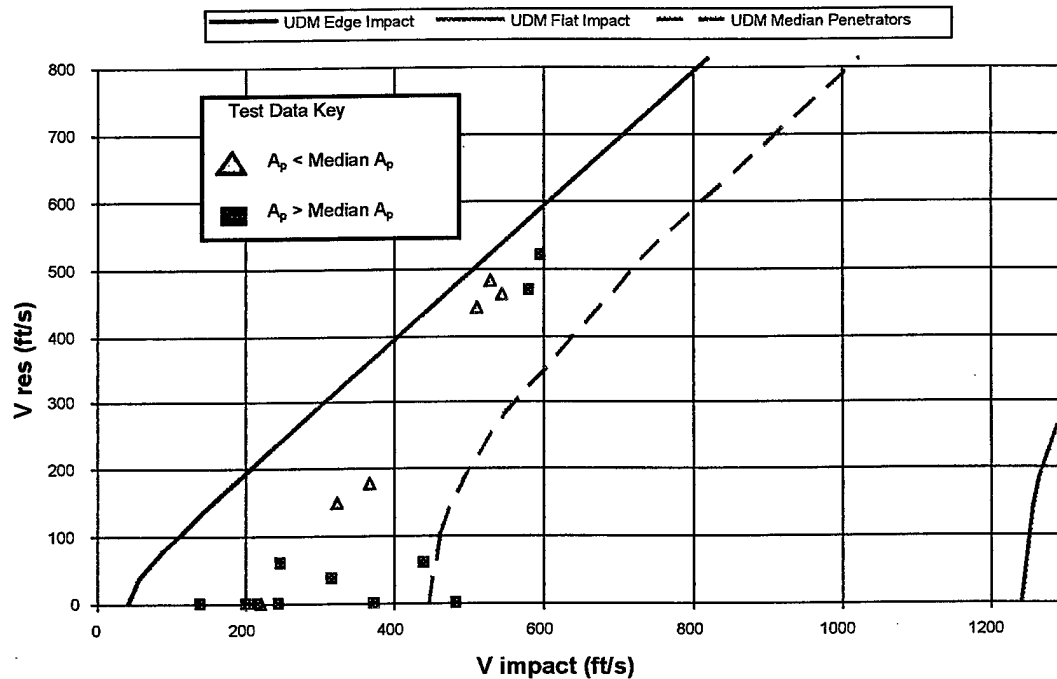
FIGURE 19. TEST SERIES 5 AND 7, RESIDUAL VELOCITY CURVES ORIENTATION COMPARISON
