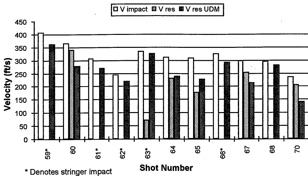
FIGURE 23. TEST SERIES 8 PREDICTION COMPARISON
