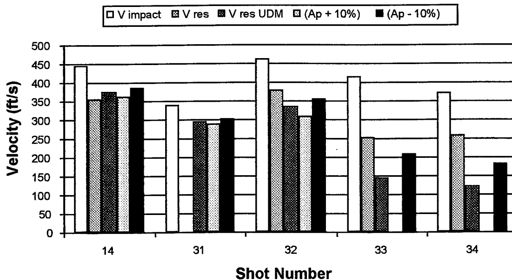
FIGURE 20. EFFECTS OF PRESENTED AREA INACCURACIES
