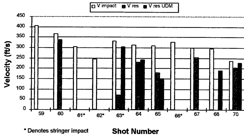
Figure B-16. Test Series 8, Impact and Residual Velocity Comparison
