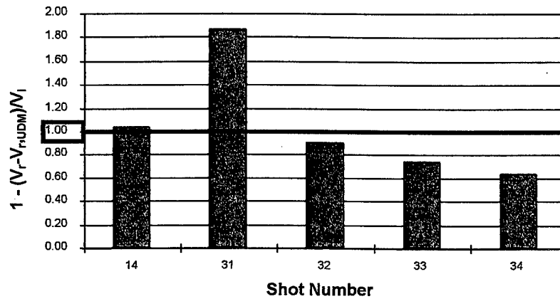
Figure B-2. Test Series 2, Prediction Accuracy
