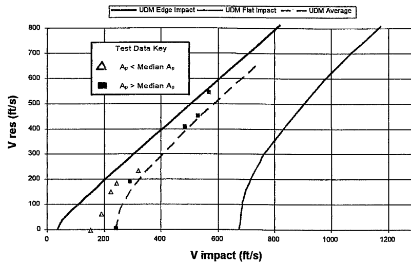
Figure B-6. Test Series 3, Impact and Residual Velocity Median Comparison
