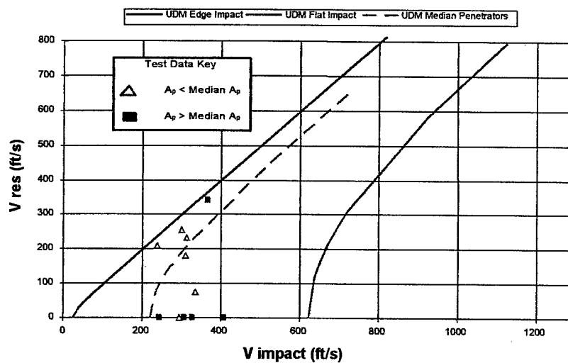
Figure B-18. Test Series 8, Impact and Residual Velocity Median Comparison
