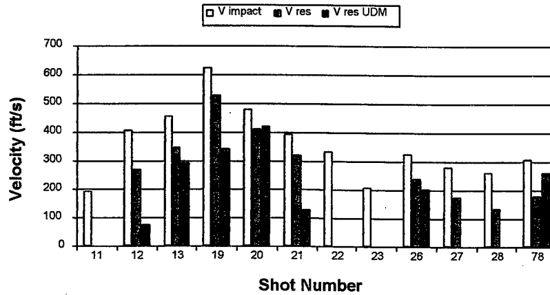
Figure B-7. Test Series 4, Impact and Residual Velocity Comparison
