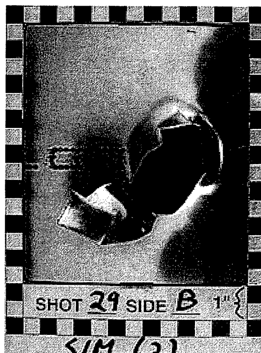
FIGURE 13. PLUGGING AND PETALING
