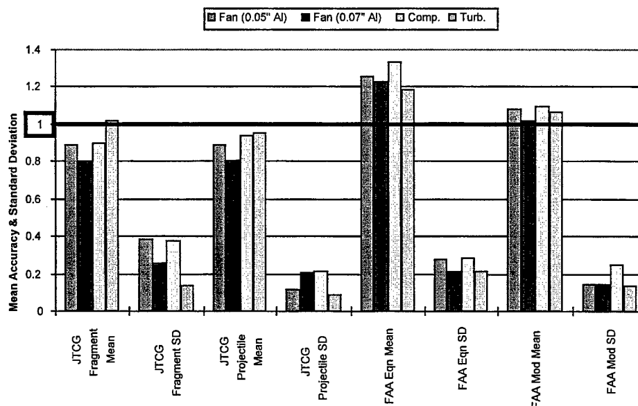
FIGURE 30. PREDICTION ACCURACY BY PREDICTION MODEL
