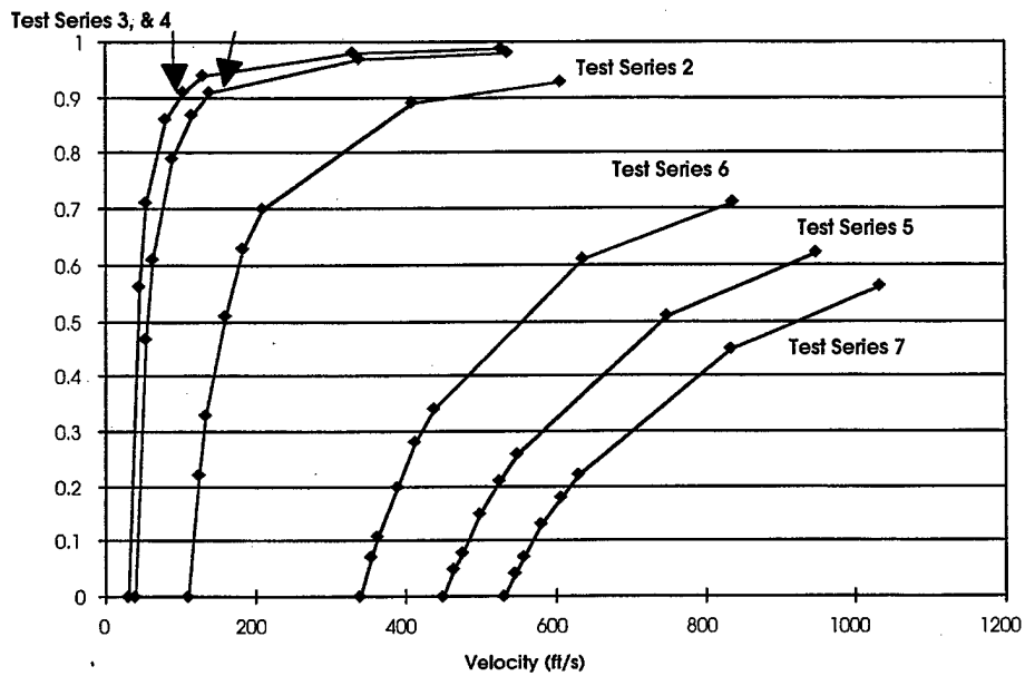
Figure 11: Pre-Test Prediction, Impact Velocity vs. Kinetic Energy Ratio
