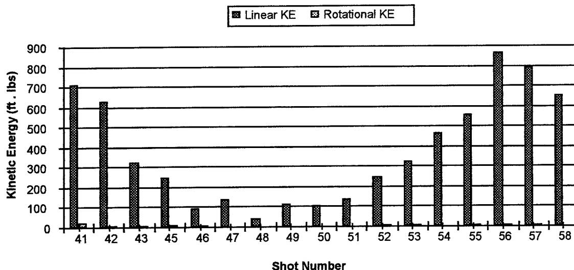
FIGURE 27. TEST SERIES 5 AND 7, KINETIC ENERGY GRAPHICAL COMPARISON
