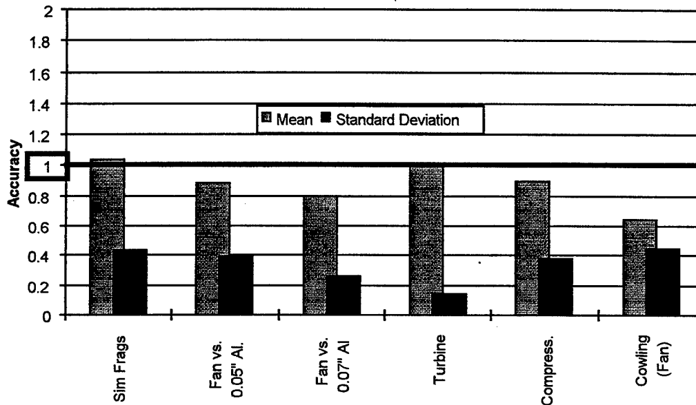
FIGURE 29. PREDICTION ACCURACY BY FRAGMENT TYPE
