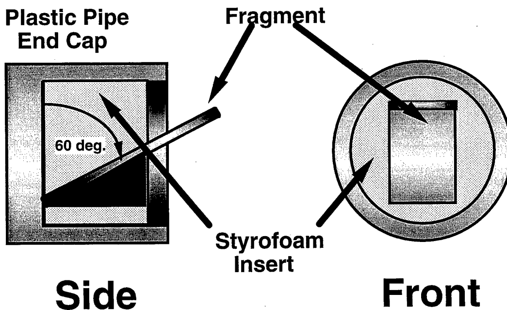
Figure 5: Sabot Impact Orientation Angle Control, (60 degrees shown)
