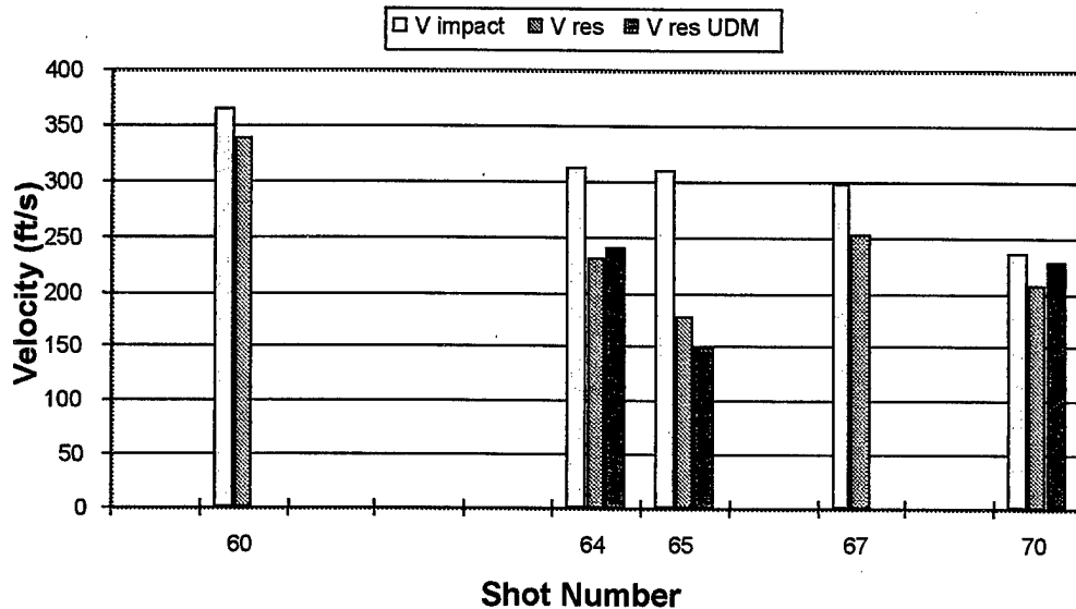
FIGURE 24. TEST SERIES 8 PREDICTIONS (SKIN IMPACTS ONLY)
