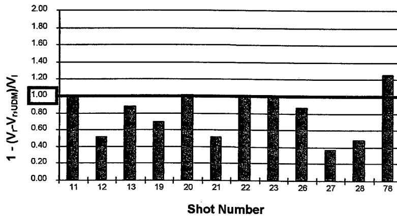
Figure B-8. Test Series 4, Prediction Accuracy
