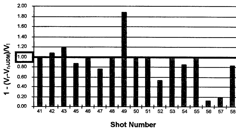
Figure B-11. Test Series 5 and 7, Prediction Accuracy
