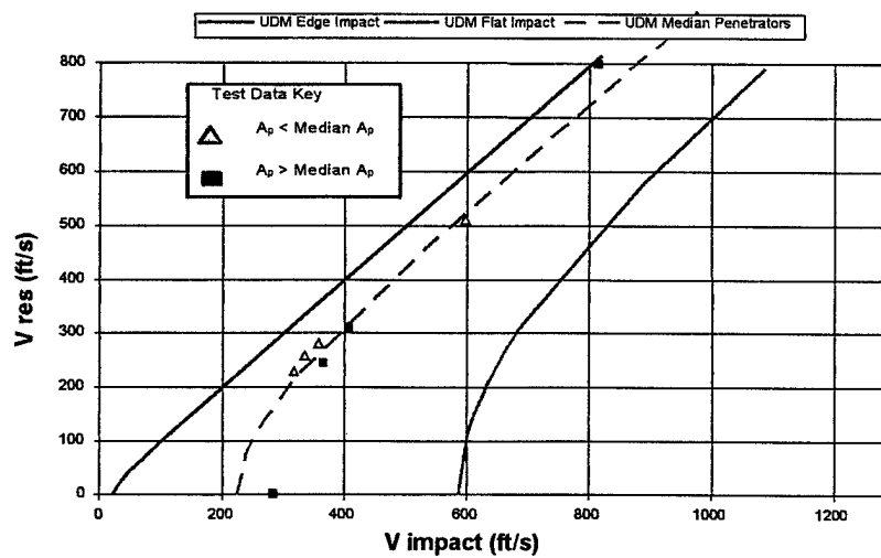
Figure B-15. Test Series 6, Impact and Residual Velocity Median Comparison
