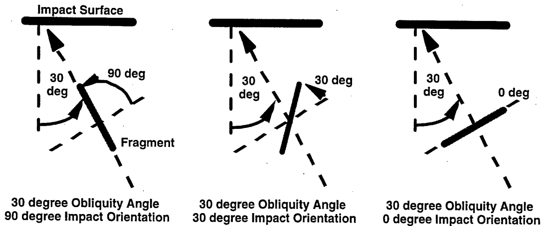
Figure 2: Examples of Obliquity and Impact Orientation
