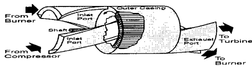
Figure 6: Four-port wave rotor schematic diagram.
