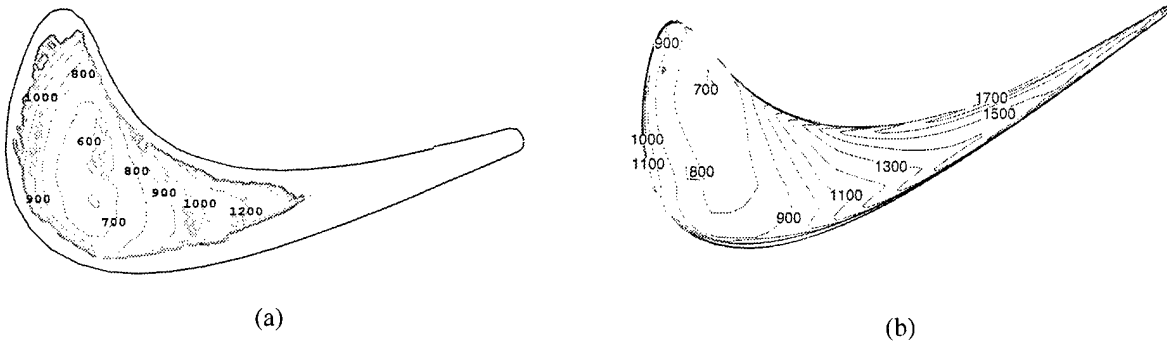
Figure 3: Rounded edge blade tip heat transfer coefficient ( W/m^2/K ) for 2.03 mm clearance and Tu=5\% , (a) measure and (b) calculated, (Ref. 6).
