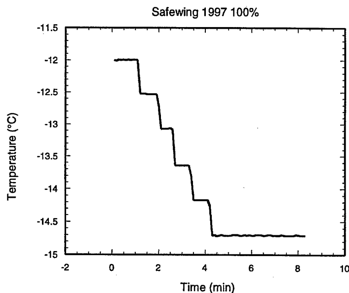
FIGURE 9. TIME SERIES OF TEMPERATURE FOR A TYPICAL FLUID TEST
