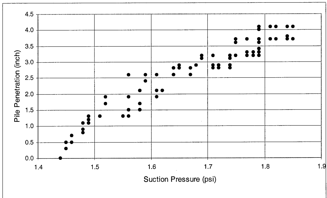
Figure I50. Suction Pressure vs. Pile Penetration (Series 18 - A)
