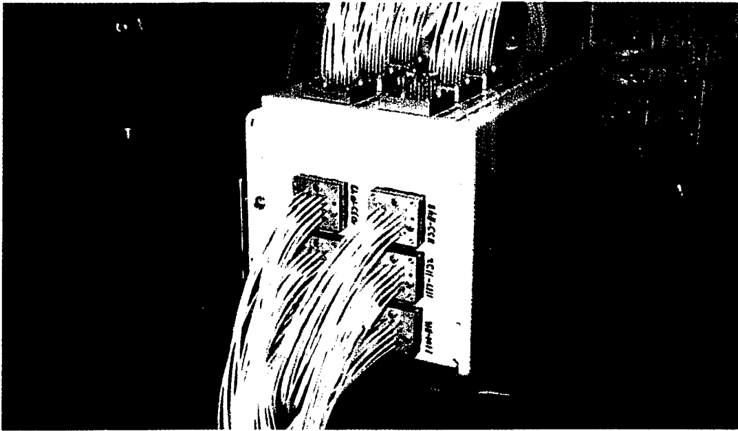
Figure 42. PSI Pressure Measurement Terminal Box
