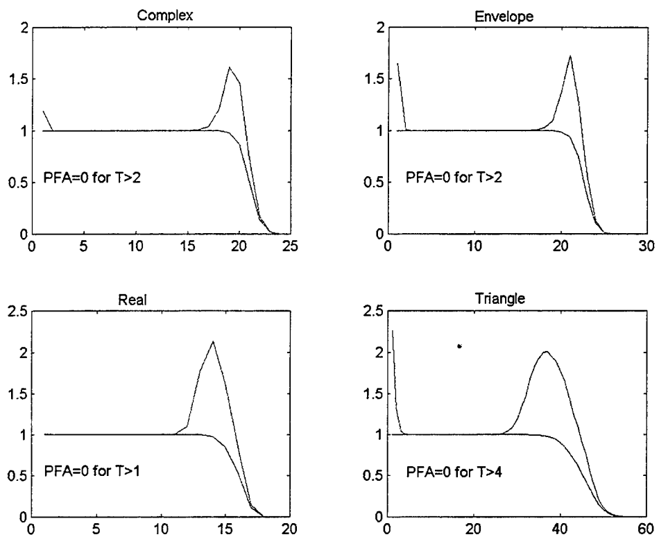
Figure 2a. Performance curve normalized percentage versus noise sigma, SNR=20dB.
