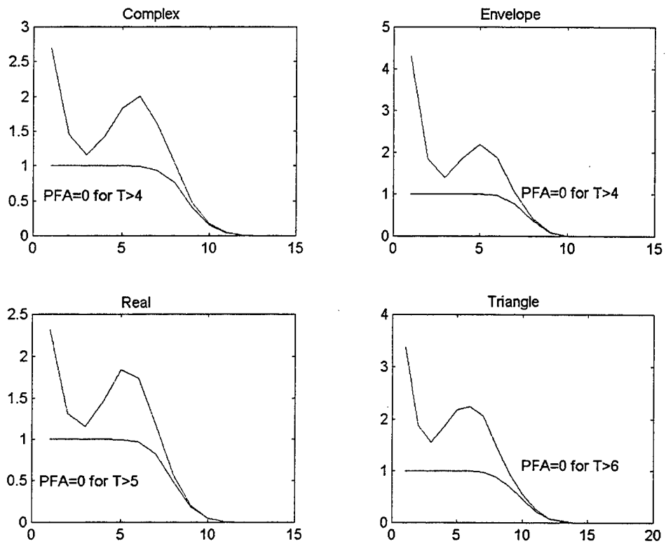
Figure 2c. Performance curve normalized percentage versus noise sigma, SNR=6dB.
