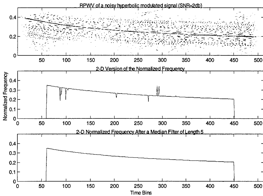
Figure VII.3: Extraction of the instantaneous normalized frequency expression from the time-frequency image. Before and after median smoothing, L=5 .
