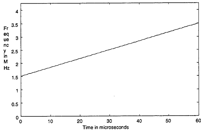
Figure VI.13: Instantaneous frequency for the heterodyned signal; Normalized frequency f_s = 1 .
