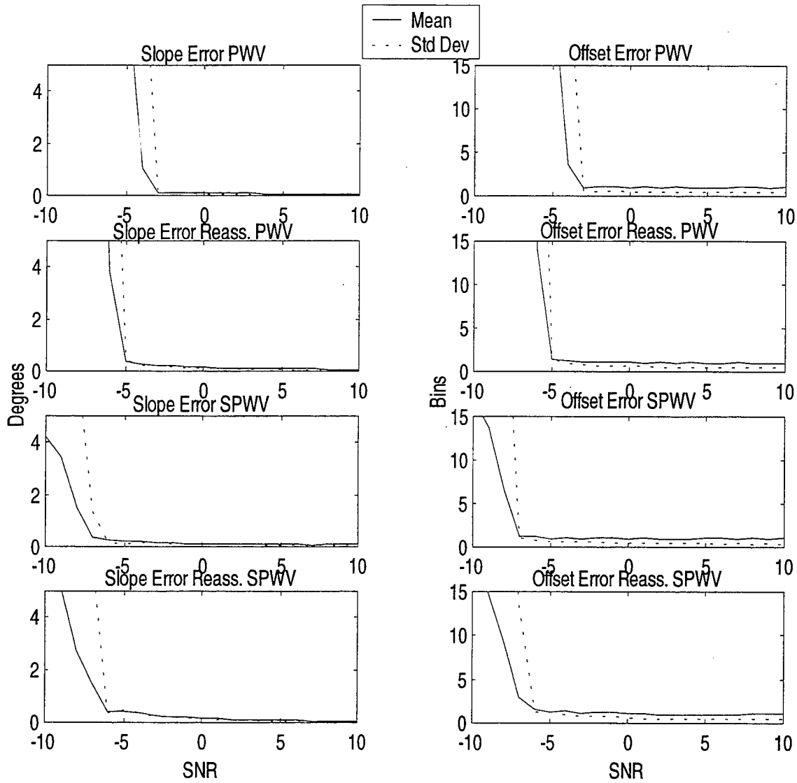
Figure VI.8: Slope and offset errors for the PWV, reassigned PWV, SPWV, and reassigned SPWV decompositions; linear chirp signals; SNR given in dB.
