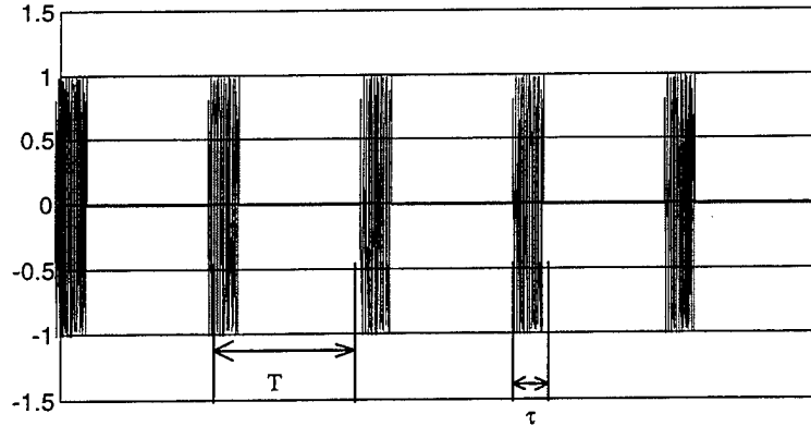
Figure VI.4: Synthetic radar signal; linear chirp modulation.
