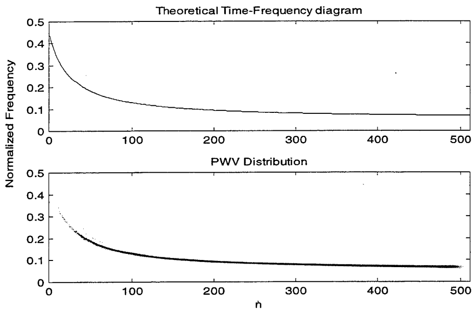
Figure VII.1: Hyperbolic modulation; normalized frequency for a=10 , n_0=25 , b=0.05 .
