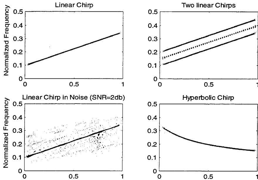
Figure V.3: Pseudo Wigner-Ville distribution; time is normalized over the pulse duration.
