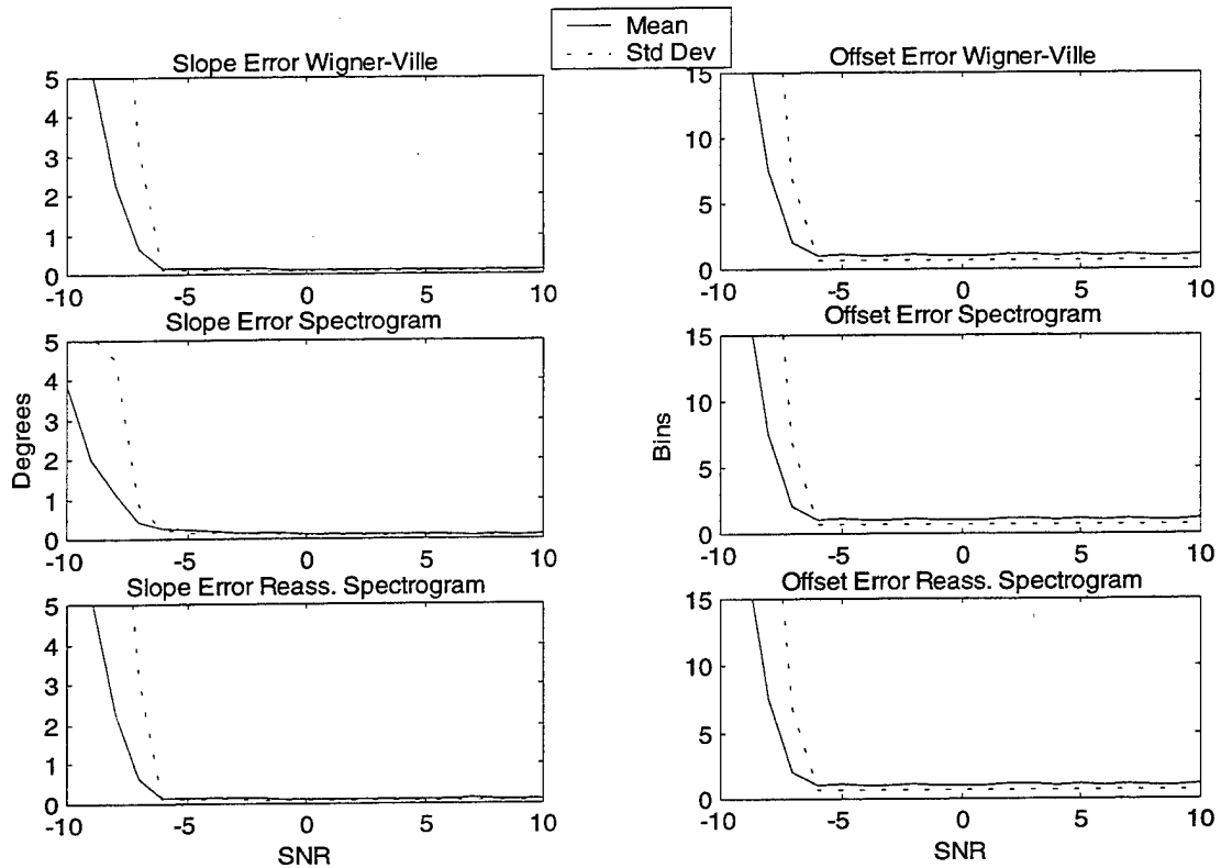
Figure VI.9: Slope and offset errors for the Wigner-Ville decomposition, Spectrogram, and reassigned Spectrogram; linear chirp signals; SNR given in dB.
