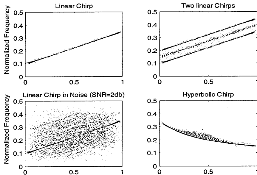
Figure V.2: Wigner-Ville distribution; time normalized to the pulse length.
