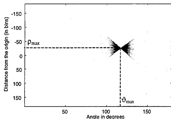
Figure VI.3: Radon transform for line shown in Figure VI.2; for \vartheta=0^\circ, \dots, 180^\circ, 1^\circ inc.
