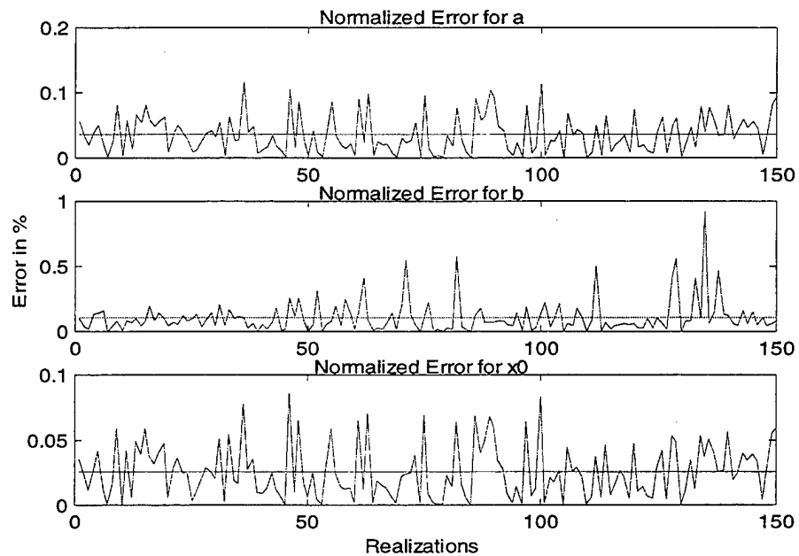
Figure VII.4: Normalized errors obtained for a , b , n_0 ; 150 randomly generated hyperbolic chirps.
