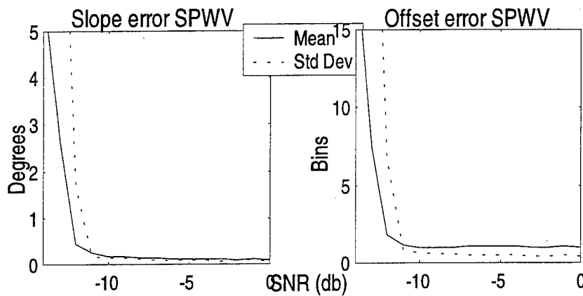
Figure VI.12: Slope and offset error for the SPWV distribution; five realizations.
