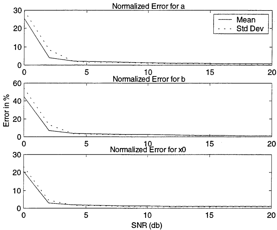
Figure VII.7: Hyperbolic chirp; normalized errors for the RPWV distribution.
