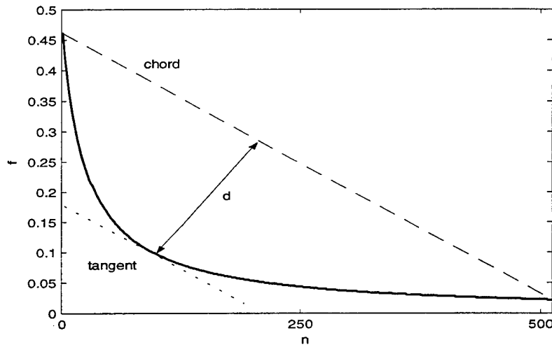
Figure VII.2: Maximum distance between a hyperbolic line and its chord; a=12 , n_0=25 , b=0 .
