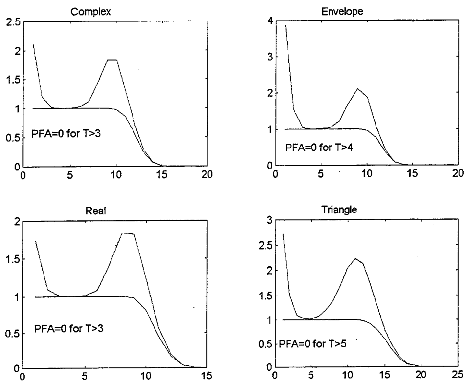
Figure 2b. Performance curve normalized percentage versus noise sigma, SNR=10dB.
