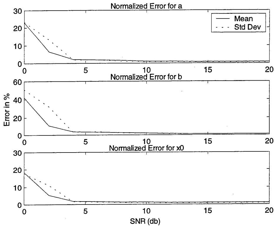
Figure VII.8: Hyperbolic chirp; normalized errors for the RSPWV distribution.
