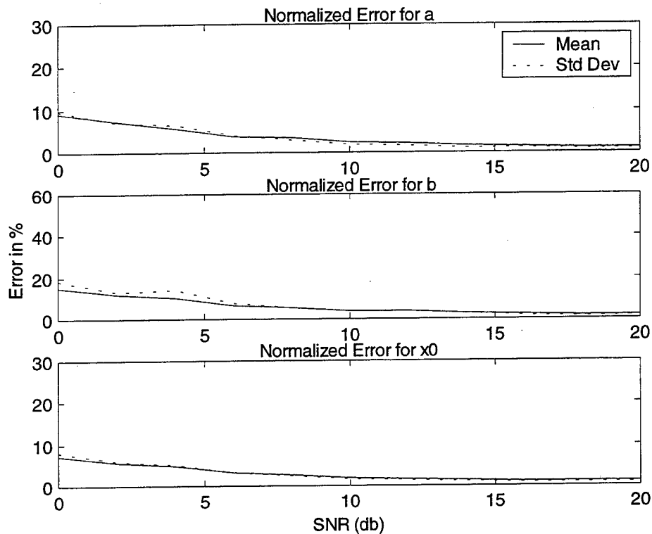
Figure VII.6: Hyperbolic chirp; normalized errors for the SPWV distribution.
