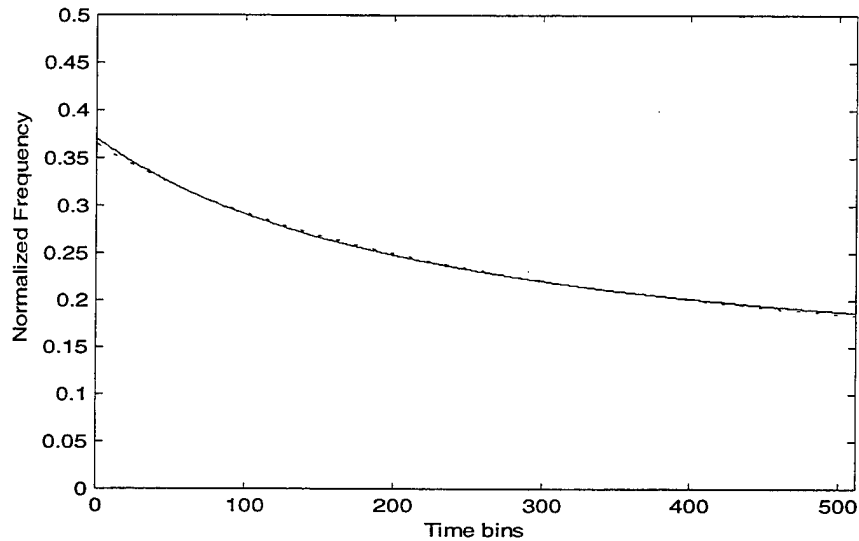
Figure VII.5: Two hyperbolic lines; Solid line: true hyperbolic curve ( a=65 , b=0.1 and n_0=240 ), dotted line: estimated hyperbolic curve ( a=84 , b=0.08 and n_0=294 ).
