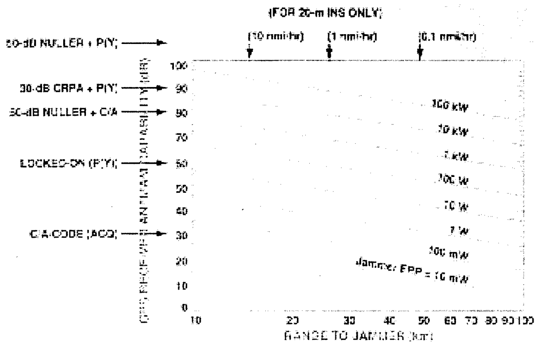
Figure 3.2 GPS Calculations From Ref. Alterman, 1995, p. 54.
