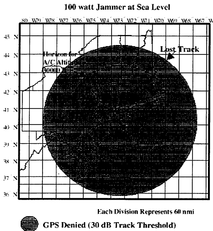
Figure 3.1 Outage Area Caused by a 100-W Jammer From Ref. Corrigan et al., 1999, p. 5-7.
