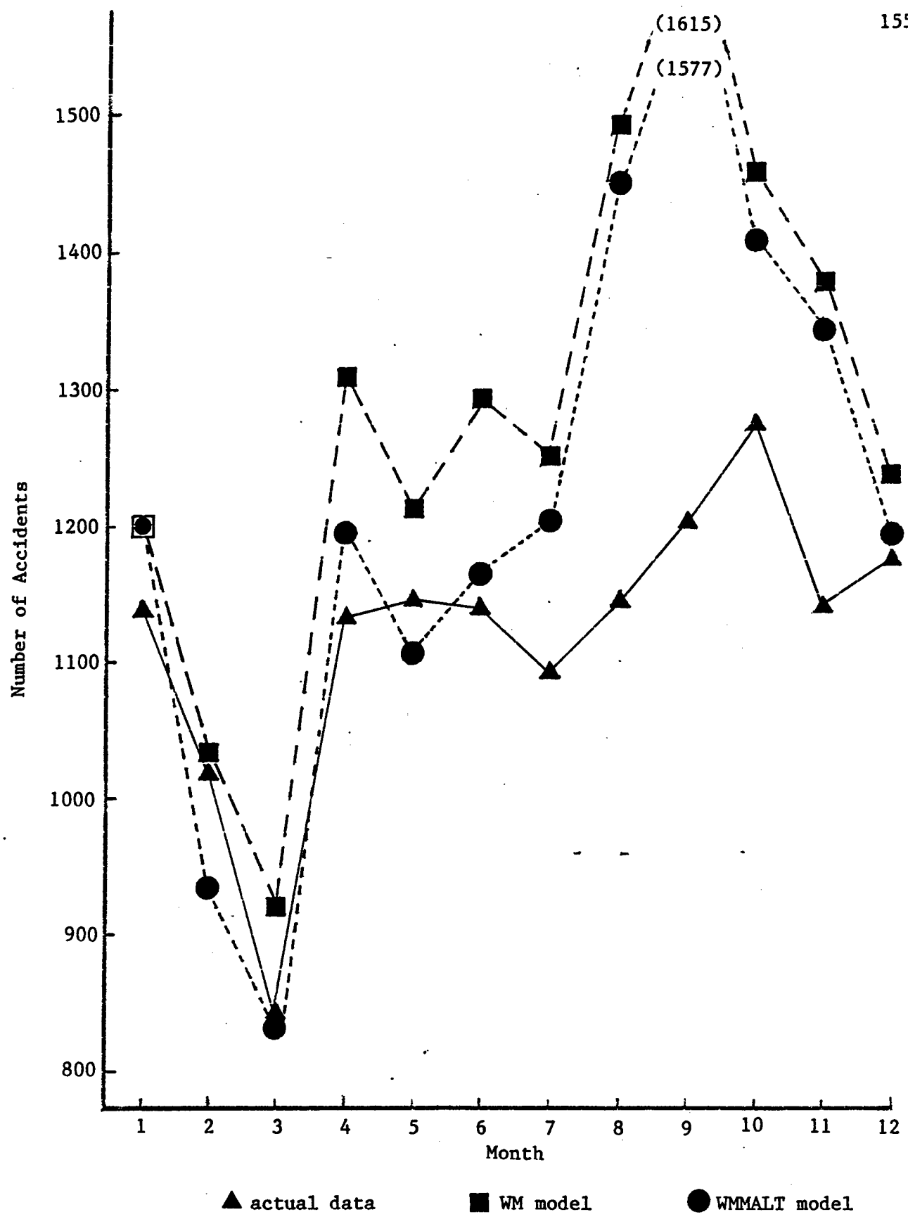
Figure 4. Forecasts for ARMYWIDE total.
