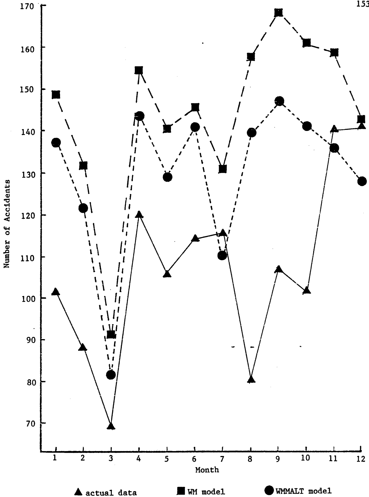
Figure 2. Forecasts for TRADOC total.
