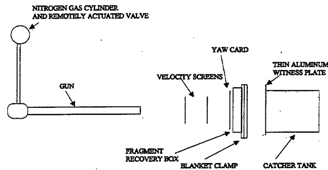
Figure 5. Test Layout.
