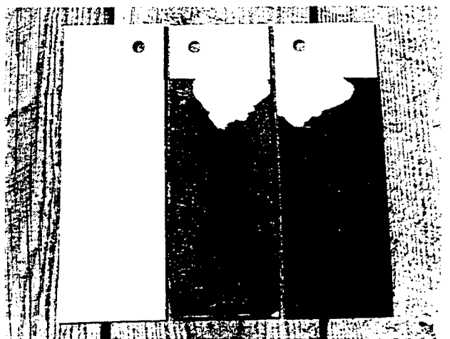
FIGURE 6 - Examples of crevice corrosion affecting partially coated stainless steel with (left to right) barrier coating and antifouling ablative-Cu and elastomeric type coating. (Top) S31603 (80% coated), (center) S20910 (20% coated), and (bottom) N08367 (80% coated).
