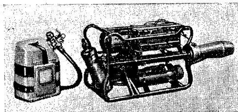
Fig. 1. AGD aerosol generator ready to work.
