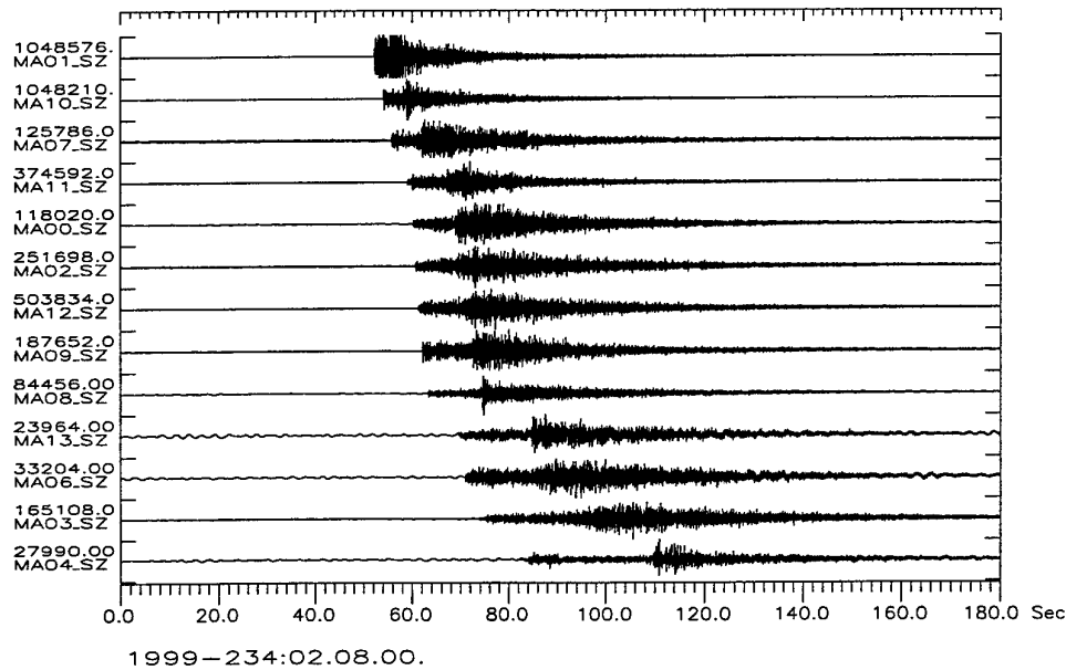
Fig. 6.4.4. The unfiltered vertical-component records at all MASI-1999 stations of the 22 August 1999 M_L 2.6 event at the Stuuragurra fault. The stations observed the event in epicentral distances between 0.2^\circ and 2^\circ . The closest station MA01 was clipped.
