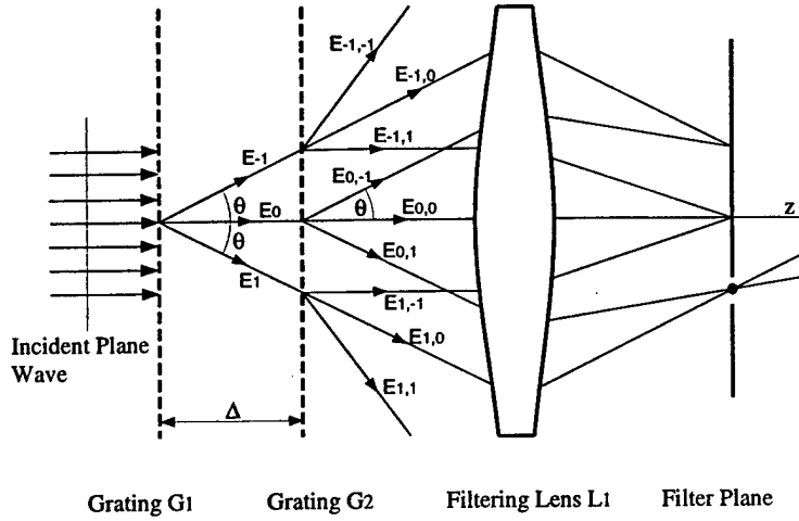
Figure 3.3: Schematic of the principle of CGS.
