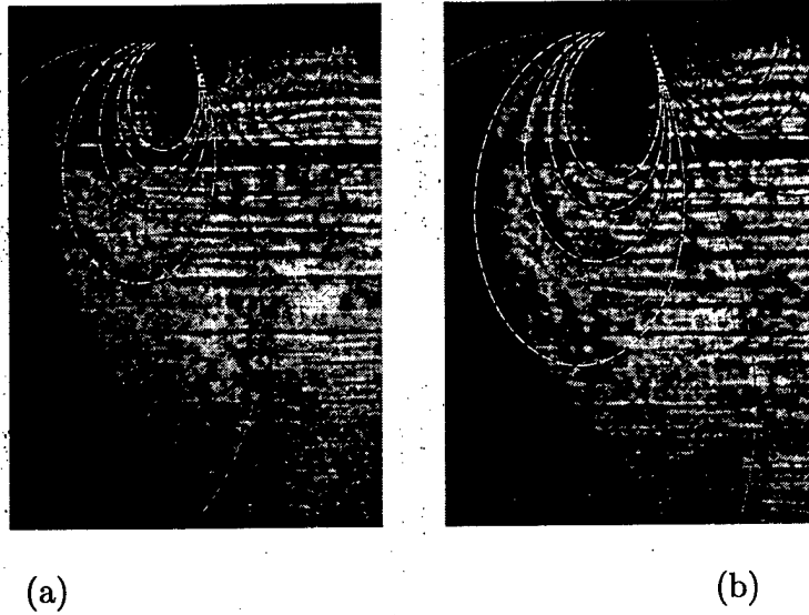
Figure 3.21: Experimental CGS interferograms and numerical simulation reconstructed from one term fitting analysis. Composite materials. (a) At t = 12 \mu\text{s} and (b) at t = 20 \mu\text{s} .
