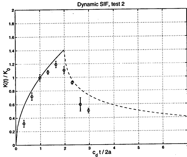
Figure 3.17: Normalized dynamic stress intensity factor for the punch test. Second test.
