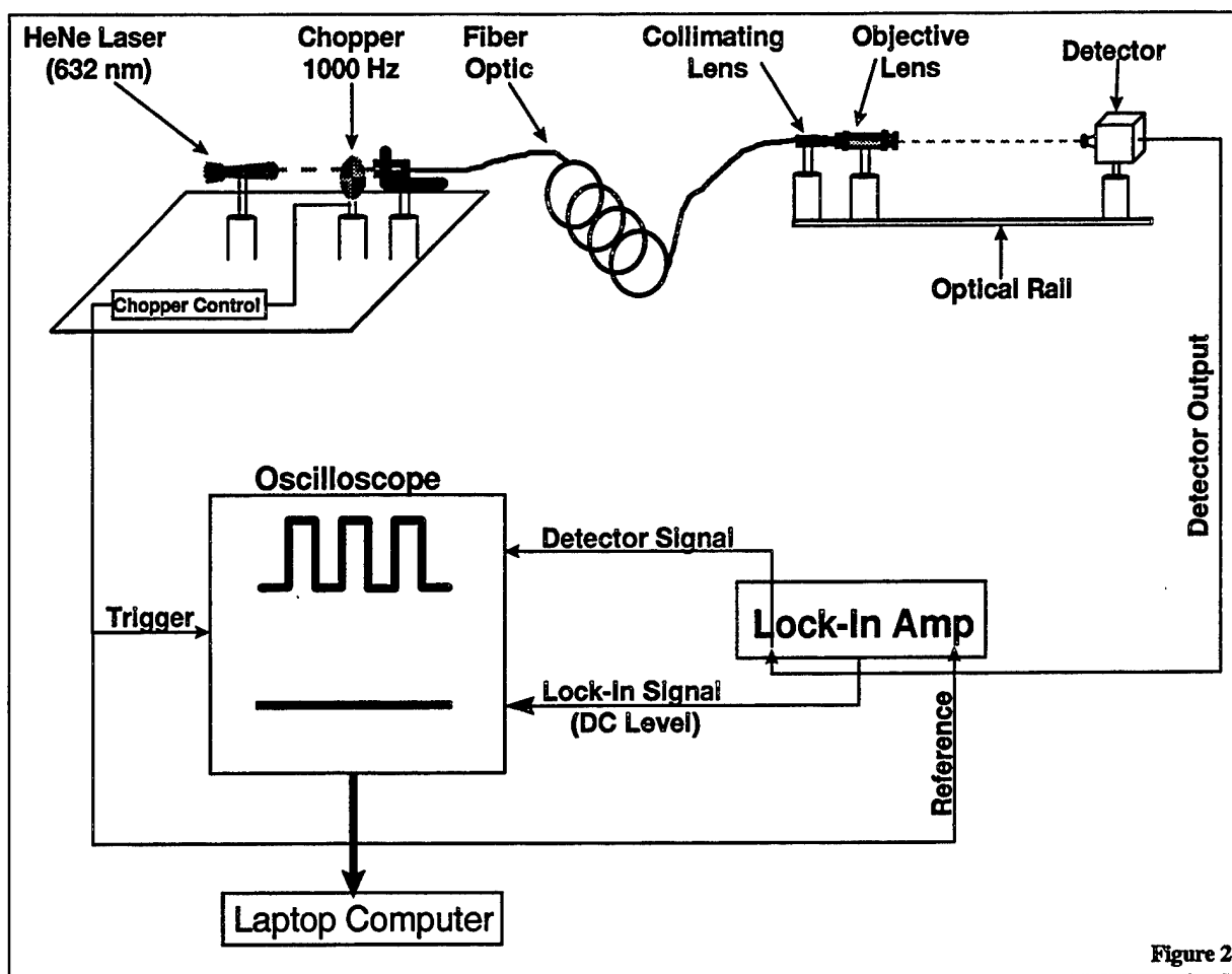
Figure 2. Schematic Diagram of Light-Attenuation Measurement Apparatus.
