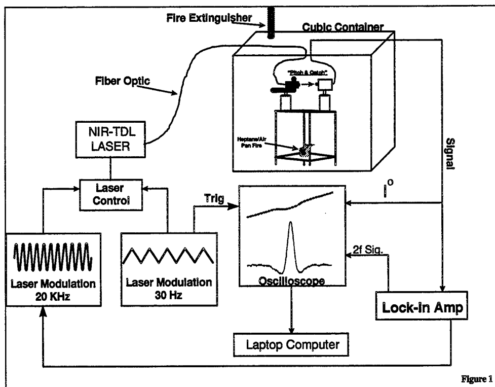
Figure 1. Schematic Diagram of Experimental HF Measurement Apparatus.
