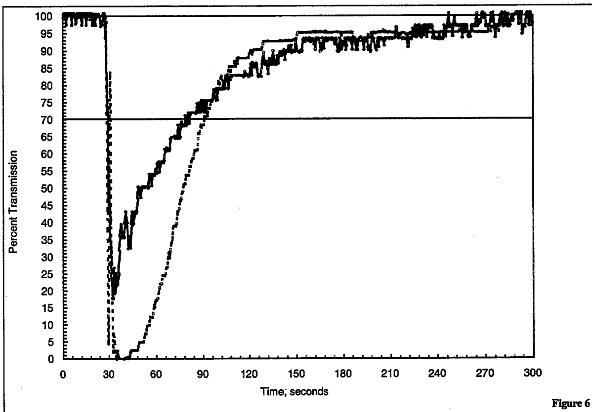
Figure 6. Percent Transmission Profiles Collected From Measurement of Light Attenuation, While an Extinguisher Containing Either FE-36 Plus APP (Solid Line) or FE-36 Plus NaHCO 3 (Dashed Line) Was Released Inside an M1-Abrams Combat Vehicle. The Horizontal Line Drawn Across the Graph Is the 70% Transmission Level, Which Corresponds to Clear Visibility by the Human Eye.
