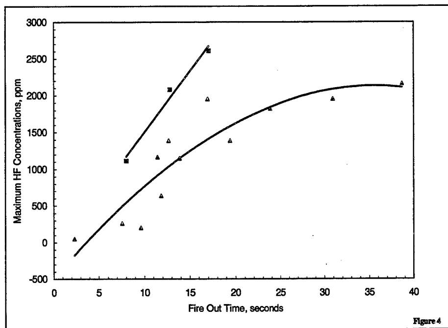
Figure 4. Peak HF Concentrations vs. Fire Out Times for Fires Extinguished by FE-36 (■) and FE-36 Plus APP (▲).
