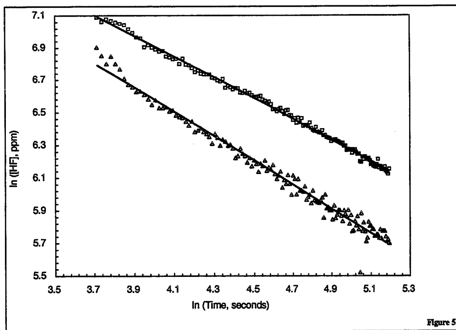
Figure 5. Rate Plot of ln HF Concentrations vs. ln Time for Fires Extinguished by FE-36 (□) and FE-36 Plus 7% APP (Δ). The Straight Solid Lines Represent Linear Regression Analysis of the Data.
